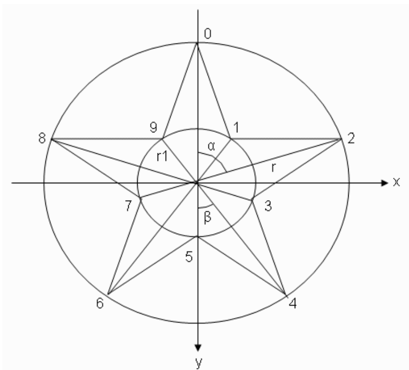
Figure 1-15 Coordinates of a star.
