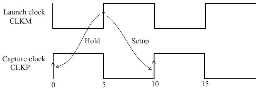
Figure 8-30 Clock waveforms for half-cycle path - case 2.
