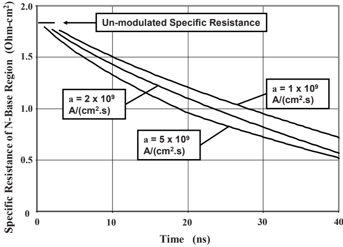
Fig. 9.93 Decrease of the N-base region resistance during the forward recovery process
