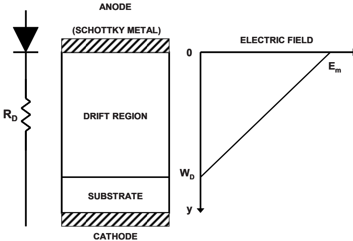
Fig. 4.1 Electric field distribution in a Schottky rectifier
