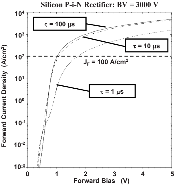
Fig. 5.10 On-state characteristics for 3,000-V P-i-N rectifiers
