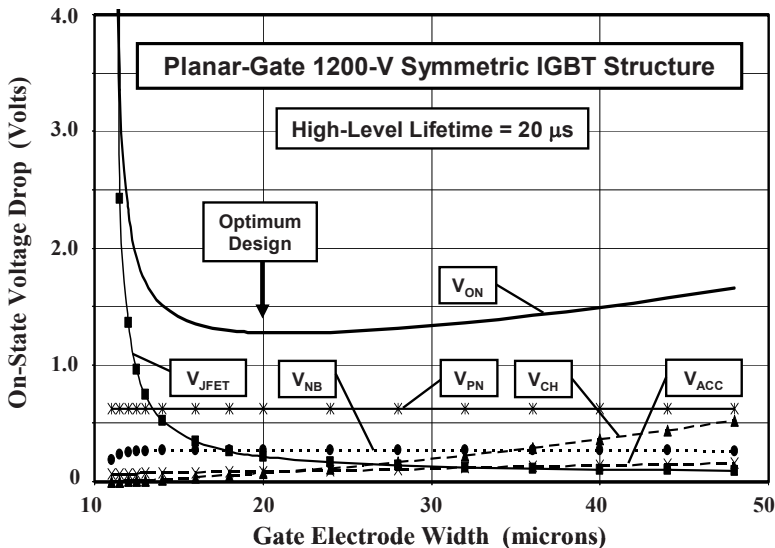
Fig. 9.208 Optimization of the on-state voltage drop of the 1,200-V planar-gate symmetric IGBT structure with a high-level lifetime of 20\text{ }\mu\text{s} in the N-base region
