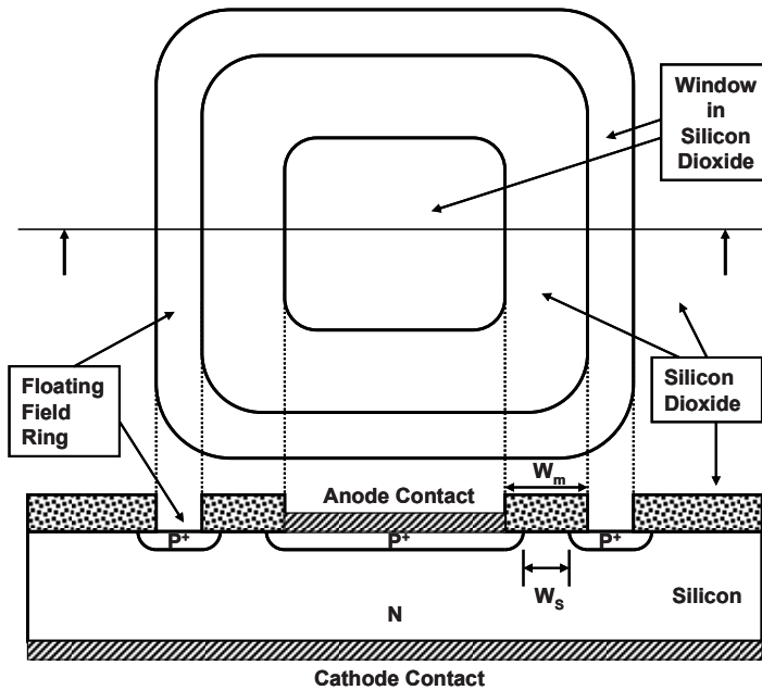
Fig. 3.20 The planar junction with floating field ring
