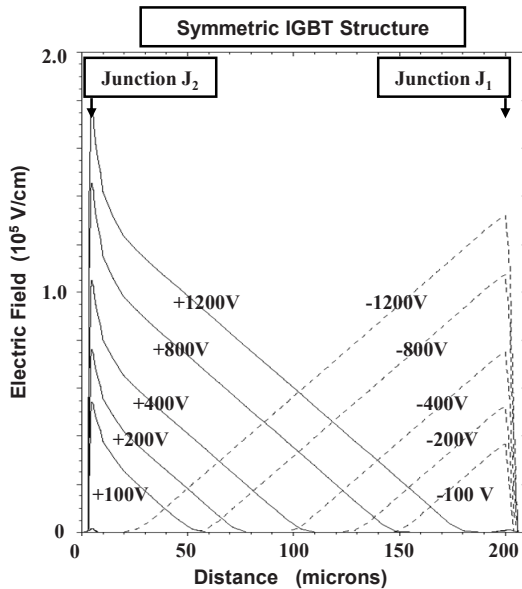
Fig. 9.22 Electric field profiles in the forward- and reverse-blocking mode for the symmetric IGBT structure
