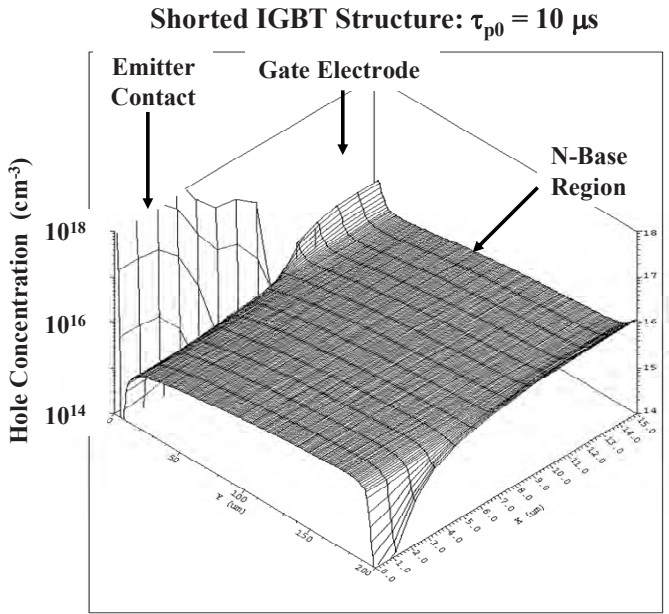
Fig. 9.225 Hole distribution in the on-state for the IGBT structure with the collector short
