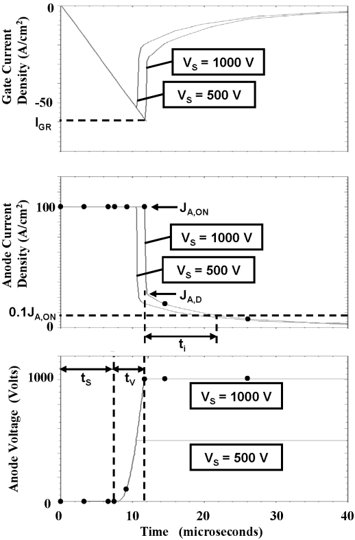
Fig. 8.71 GTO turn-off waveforms
