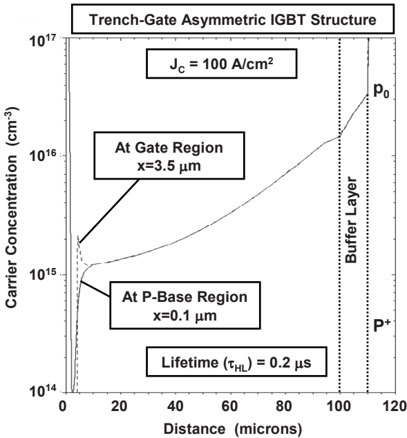
Fig. 9.185 Hole concentration profiles for the trench-gate asymmetric IGBT structure at the P-base and gate regions
