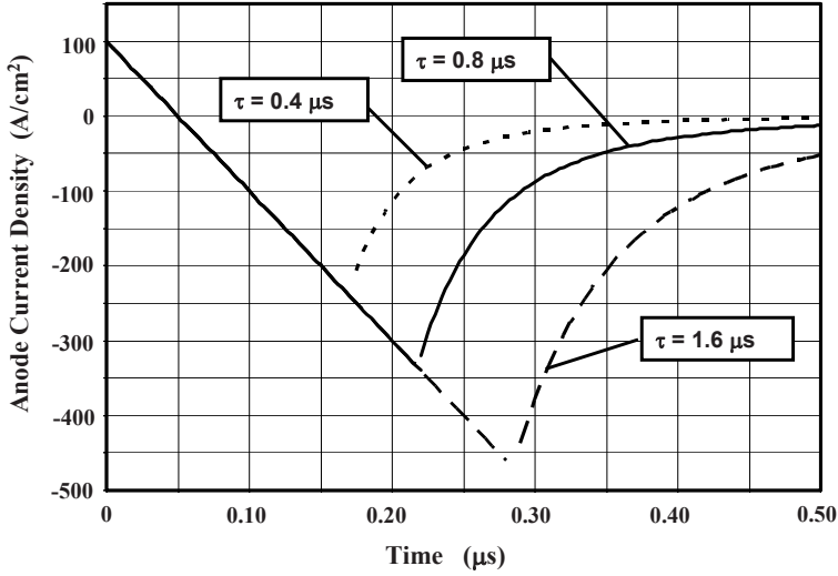
Fig. 5.52 Analytically calculated reverse recovery current waveforms for the nonpunch-through structure
