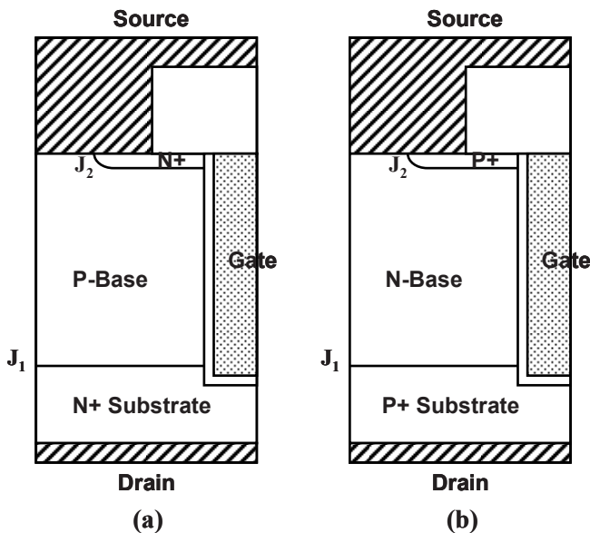
Fig. 6.136 INV-FET power MOSFET structures
