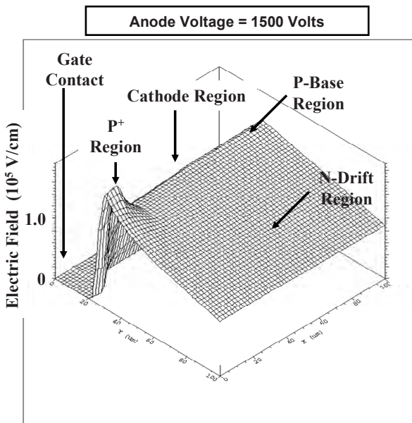
Fig. 8.58 Electric field distribution for a thyristor structure with self-protection in gate region
