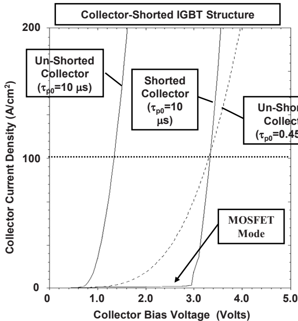
Fig. 9.223 Comparison of the on-state characteristics of the IGBT structures with and without the collector short
