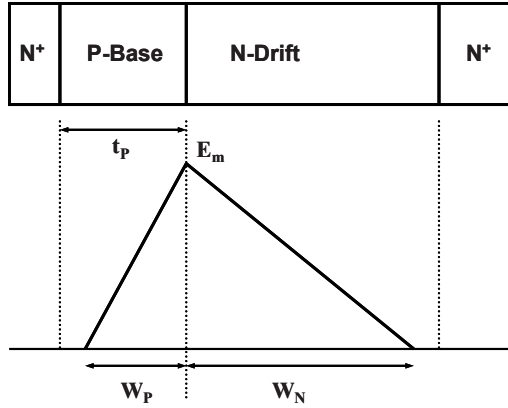
Fig. 6.148 Reach-through in a power MOSFET structure
