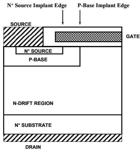
Fig. 6.147 Planar power MOSFET structure
