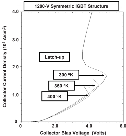
Fig. 9.204 Latch-up characteristics for the 1,200-V symmetric IGBT structure
