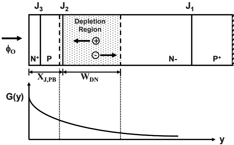
Fig. 8.55 Optically induced current in the gate region of the light-activated thyristor structure
