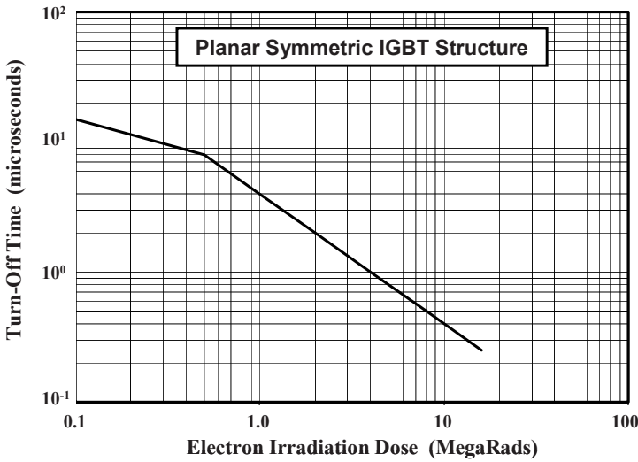
Fig. 9.205 Controlling turn-off time of the symmetric IGBT structure with 3-MeV electron irradiation
