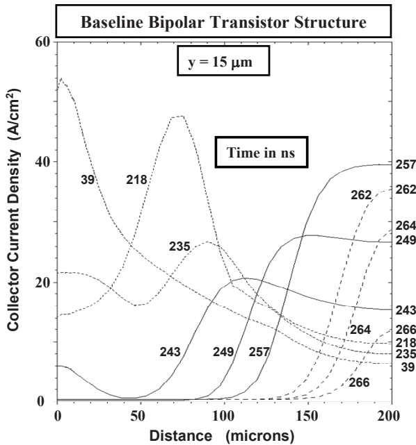
Fig. 7.82 Collector current density within the P-base region of the bipolar power transistor during the turn-off transient
