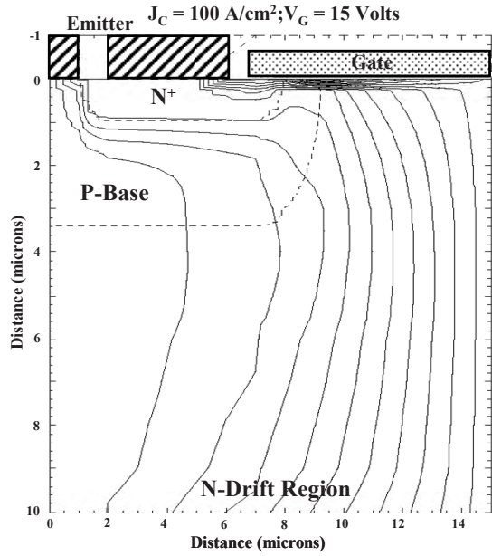
Fig. 9.157 Current distribution ( flow lines ) in the symmetric IGBT structure without the bipolar bypass path
