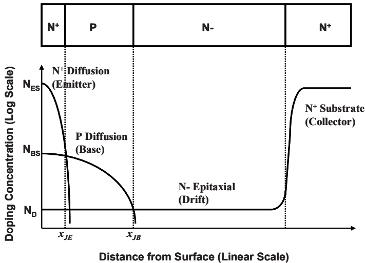
Fig. 7.2 Doping profile for the power bipolar N–P–N transistor structure
