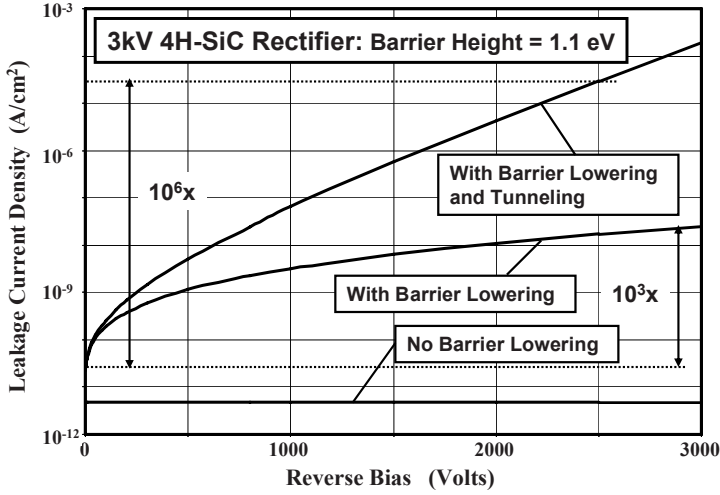
Fig. 4.18 Leakage current density for a 3-kV 4H-SiC Schottky rectifier
