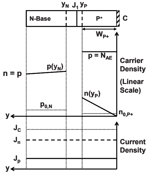
Fig. 9.59 On-state carrier and current distributions at the P^+ collector/N-base junction within the IGBT structure with transparent emitter
