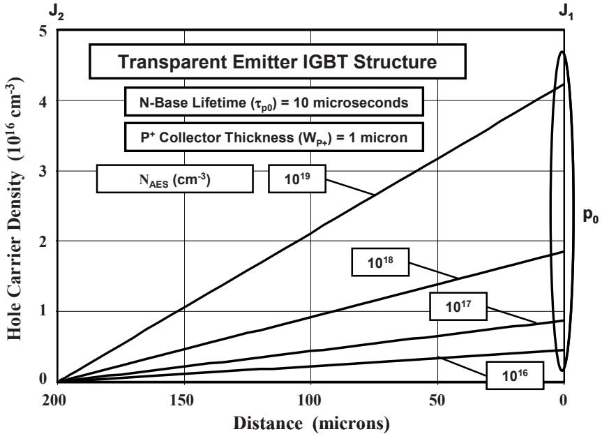
Fig. 9.60 On-state hole distribution within the transparent emitter IGBT structure under the deep P^+ region
