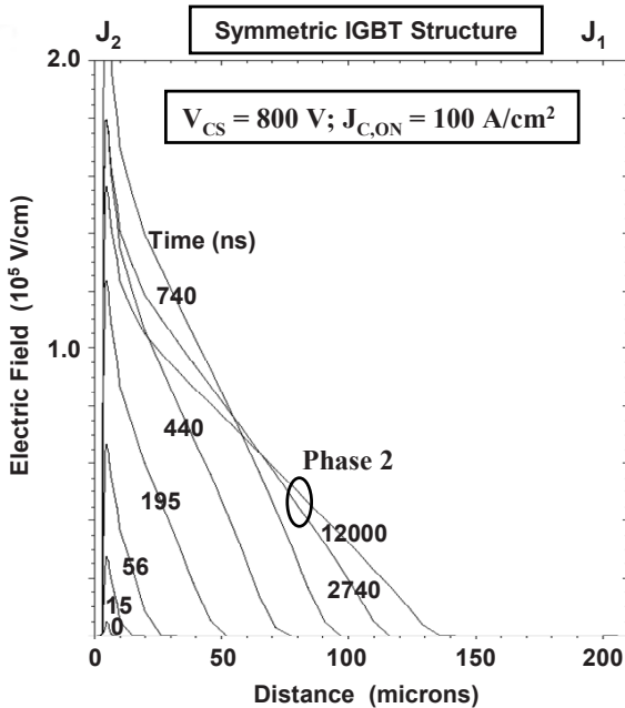
Fig. 9.111 Electric field distribution during inductive load turn-off conditions for the symmetric IGBT structure
