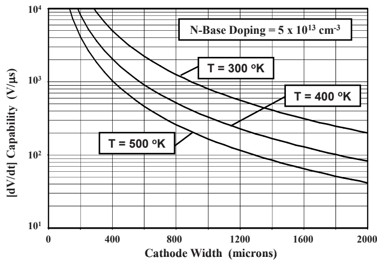
Fig. 8.45 [dV/dt] capability for a typical thyristor structure
