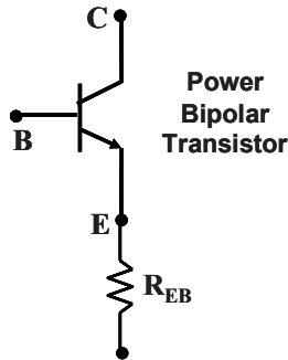
Fig. 7.84 Emitter ballasting resistance for the bipolar power transistor
