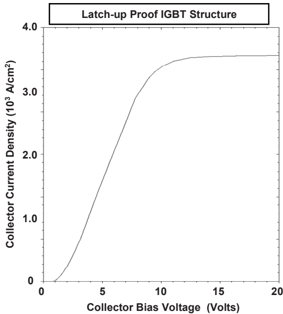
Fig. 9.168 Latch-up proof characteristics of the symmetric IGBT structure with deep P^+ region and diverter
