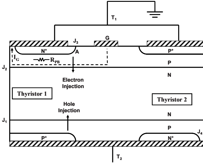
Fig. 8.90 Gate-triggering mode 1 for the triac structure
