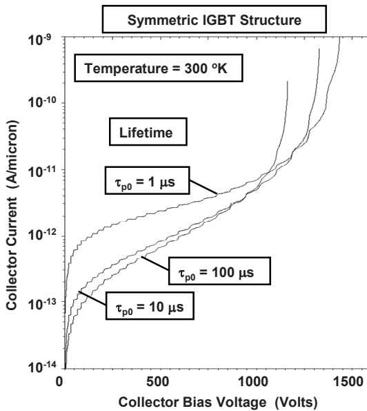
Fig. 9.21 Forward-blocking characteristics for the symmetric IGBT structure
