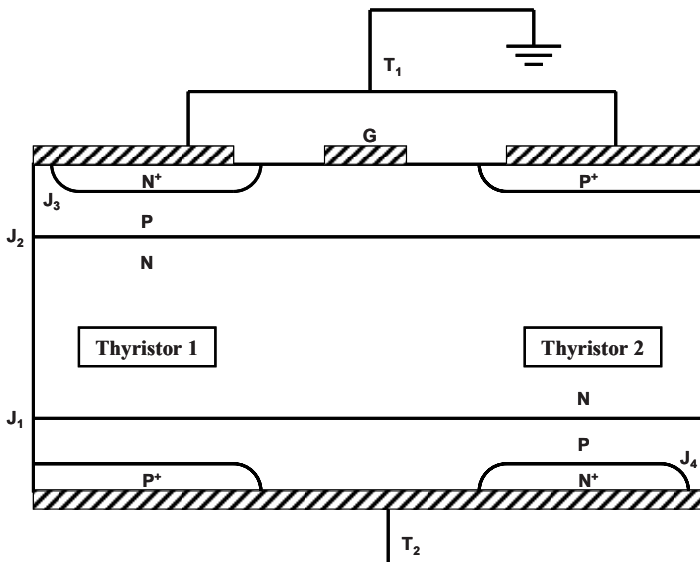
Fig. 8.89 Monolithic triac structure
