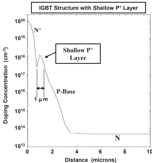
Fig. 9.147 Vertical doping profile in the IGBT structure with shallow \text{P}^+ layer
