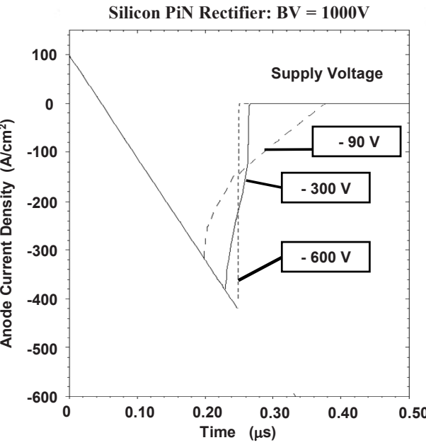
Fig. 5.49 Current waveforms for a 1,000-V silicon P-i-N rectifier during the reverse recovery transient with various supply voltages
