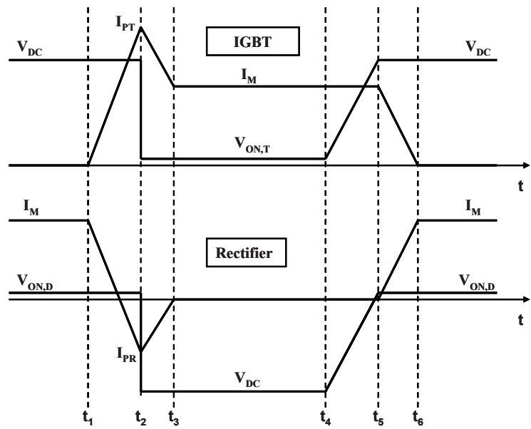
Fig. 10.2 Typical waveforms during PWM operation
