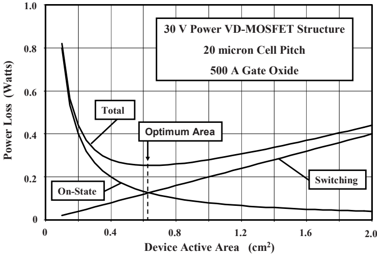
Fig. 6.114 Optimization of the active area for the power VD-MOSFET structures with 20- \mu\text{m} cell pitch
