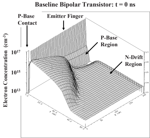
Fig. 7.73 Initial electron charge distribution within the bipolar power transistor
