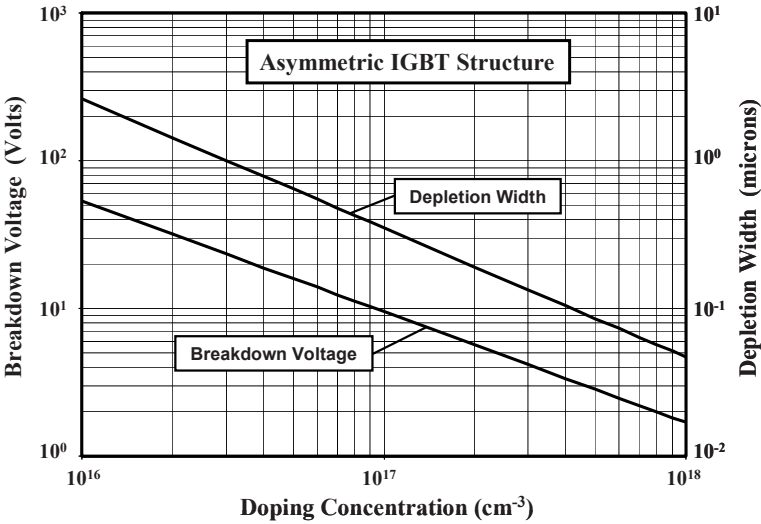
Fig. 9.27 Reverse breakdown voltage for the asymmetric IGBT structure and the corresponding depletion layer width
