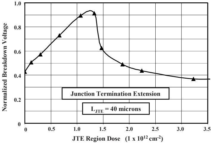
Fig. 3.56 Breakdown voltage obtained with the junction termination extension for a length of 40\text{ }\mu\text{m}
