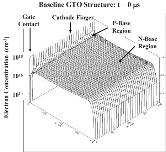
Fig. 8.72 Initial electron charge distribution within the GTO structure
