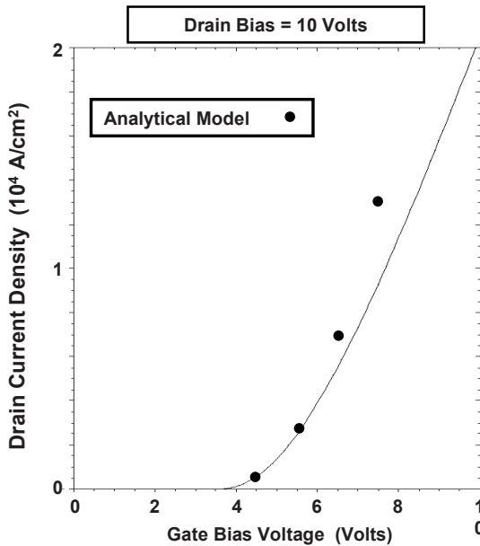
Fig. 6.67 Transfer characteristics for the VD-MOSFET structure with 20- \mu\text{m} cell pitch
