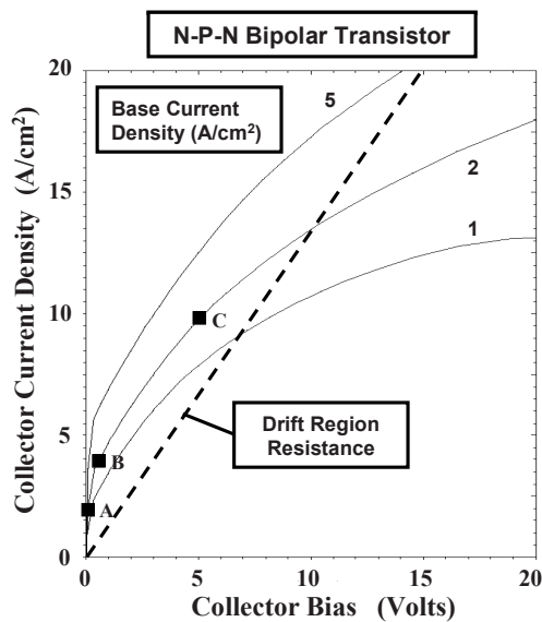
Fig. 7.52 Quasisaturation characteristics for a bipolar power transistor
