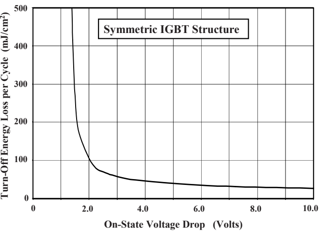
Fig. 9.126 Tradeoff curve for the symmetric IGBT structure obtained by varying the lifetime in the N-base region
