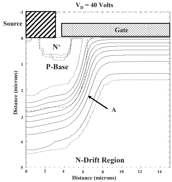
Fig. 6.11 Potential contours for the power VD-MOSFET structure with half-cell pitch of 15 \mu\text{m}
