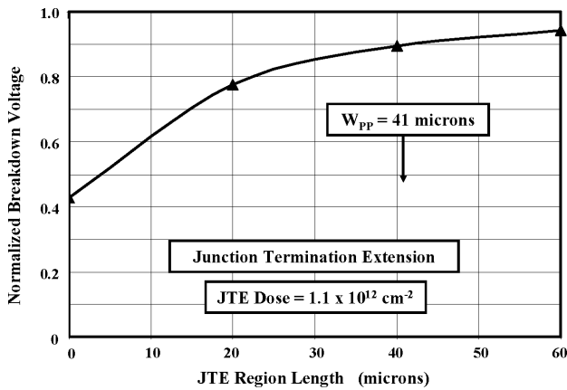
Fig. 3.58 Breakdown voltage obtained with the junction termination extension
