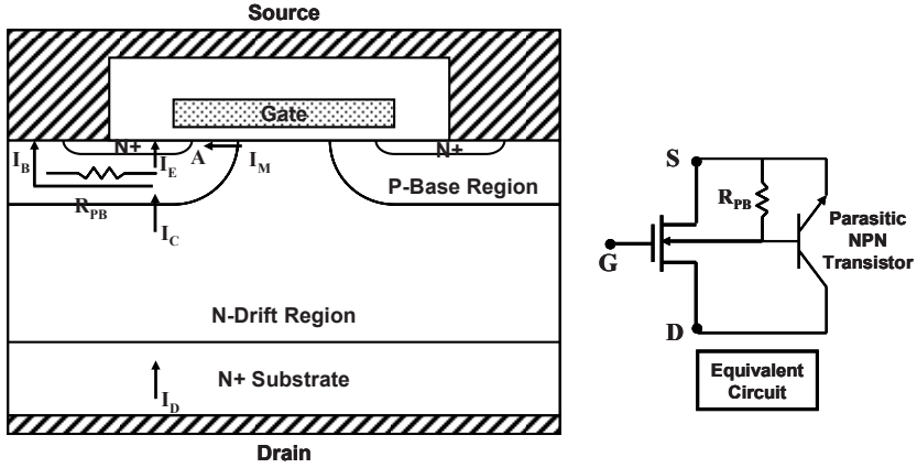
Fig. 6.129 Impact of parasitic bipolar transistor in the power MOSFET structure
