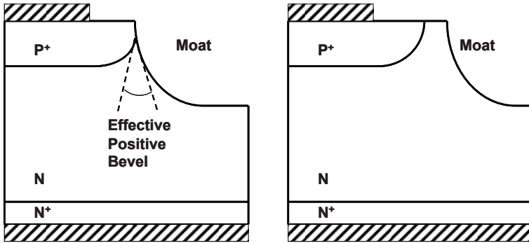
Fig. 3.53 Moat etch termination
