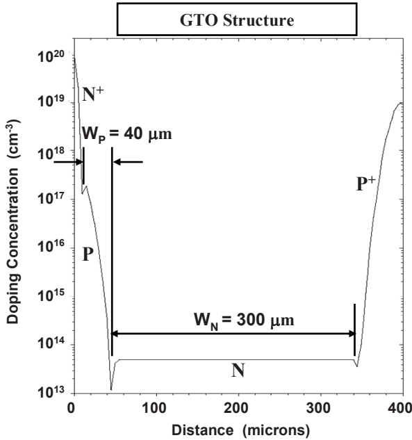
Fig. 8.70 Doping profile for the GTO structure
