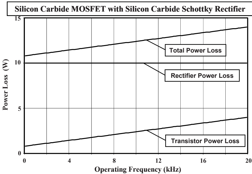
Fig. 10.14 Power losses during motor control with 400-V DC bus: silicon carbide MOSFET with silicon carbide Schottky rectifier
