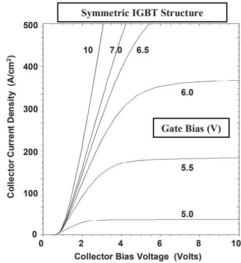
Fig. 9.66 Current saturation in the symmetric IGBT structure
