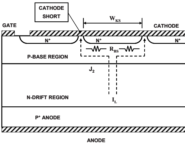
Fig. 8.13 Cathode-shortcd power thyristor structure
