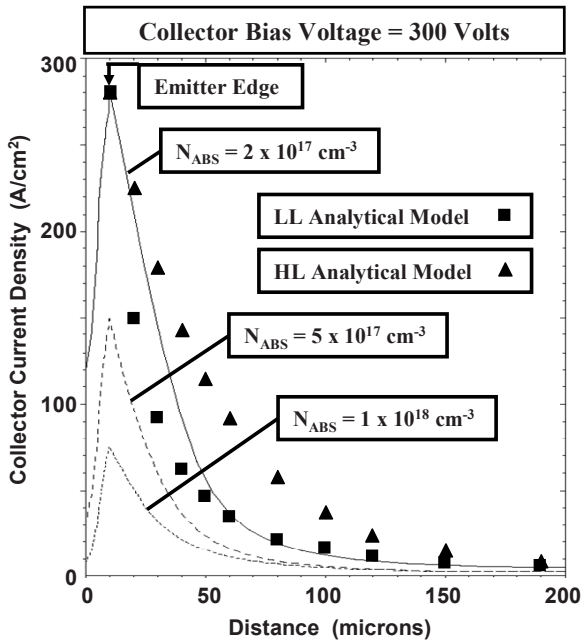
Fig. 7.40 Emitter current crowding in bipolar power transistors
