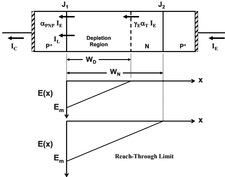
Fig. 3.60 Open-base transistor breakdown analysis
