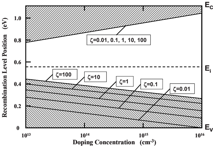
Fig. 2.30 Preferred locations for the recombination center for silicon devices operating under low-level injection conditions in the on-state
