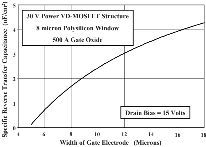
Fig. 6.79 Gate-drain capacitance for power VD-MOSFET structures
