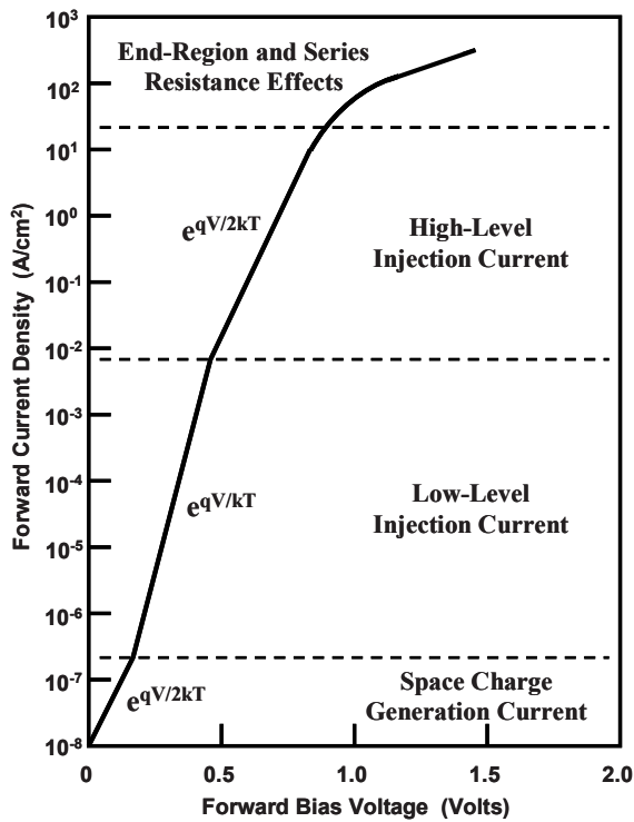
Fig. 5.7 On-state characteristics for a P-i-N rectifier
