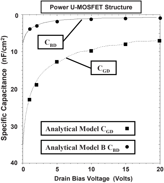
Fig. 6.94 Reverse transfer and output capacitances for the U-MOSFET structures with 2- \mu\text{m} cell pitch
