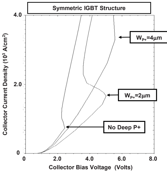
Fig. 9.144 Latch-up characteristics of symmetric IGBT structures
