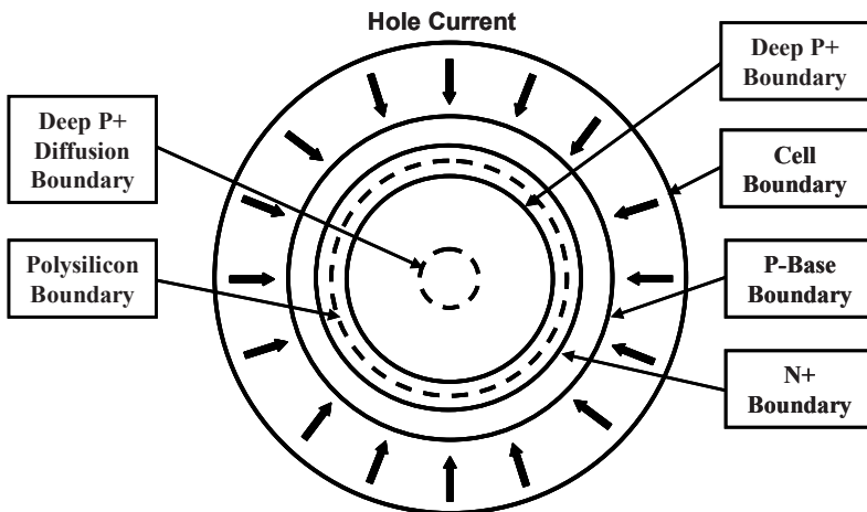
Fig. 9.165 Bipolar current distribution in the IGBT structure with circular polysilicon window in a circular array
