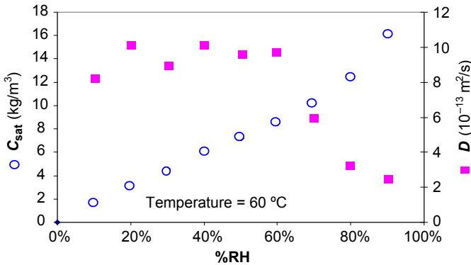
Figure 4.10 C_{\text{sat}} and D_z of the low-dielectric polymeric material.
