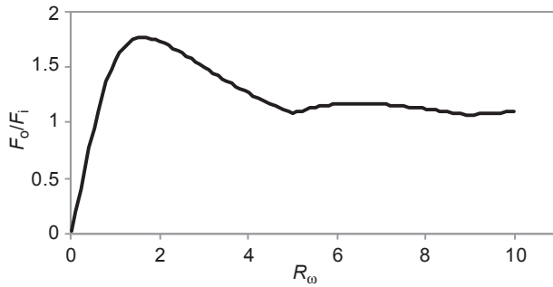
Figure 7.21 Amplification of impact force.
