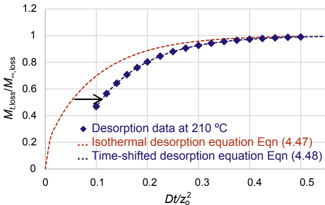
Figure 4.13 Extraction of D_z using the time-shift method.
