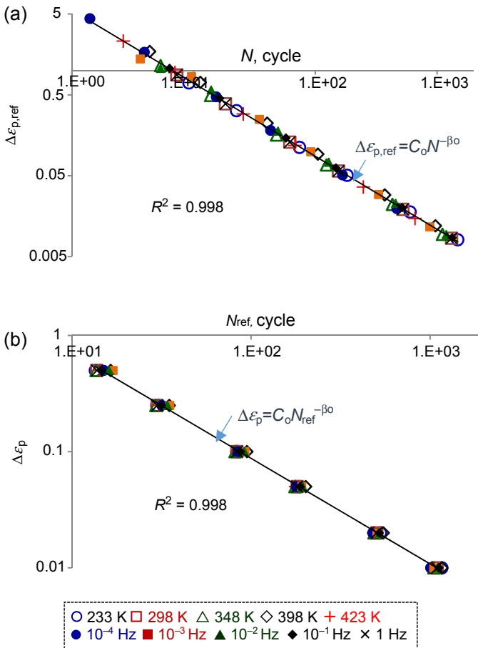
Figure 3.10 (a) \Delta\epsilon_{p,ref} versus N and (b) \Delta\epsilon_p versus N_{ref} for eutectic SnPb solder.
