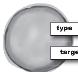
Event object
