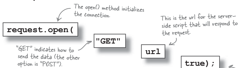
thumbnails.js
