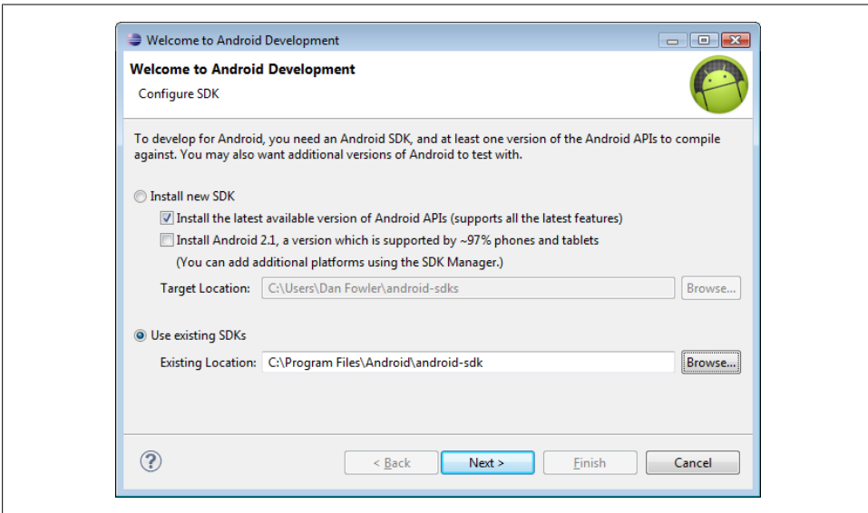
Figure 1-13. Connecting the newly installed SDK to the newly installed ADT plug-in
