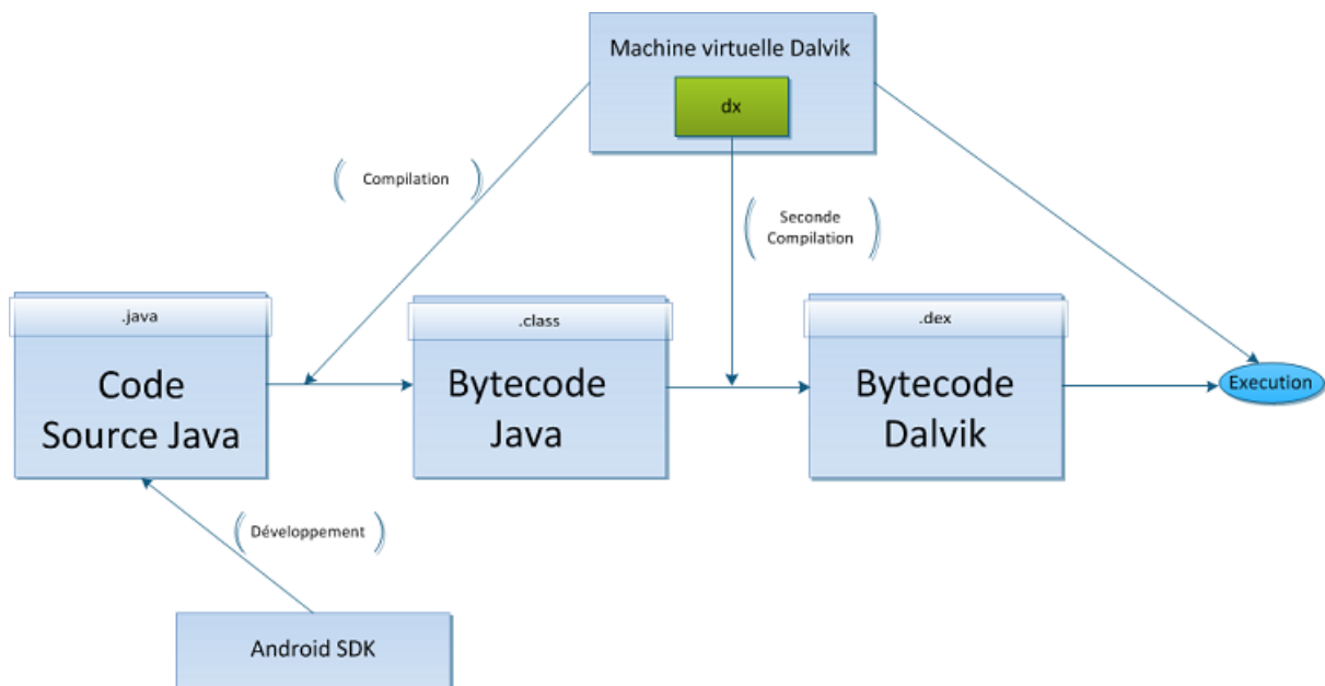
Figure 7.14 : Dalvik
