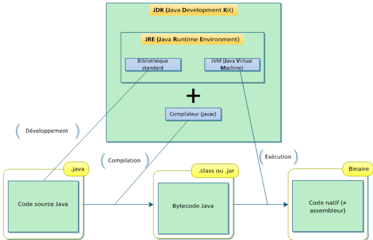
Figure 7.13 : Architecture Java
