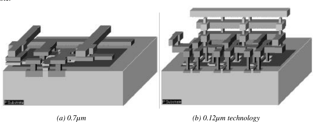
Figure 5-1: Evolution of interconnect between 0.7 \mu\text{m} technology and 0.12 \mu\text{m} technology (Inv3.MSK)
