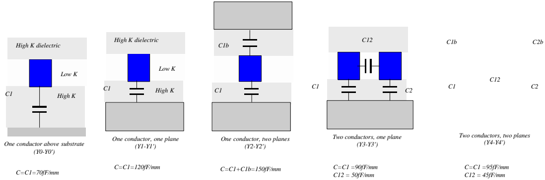
Figure 5-22: Basic configurations illustrating the cross-sections of the interconnect network (0.12μm)
