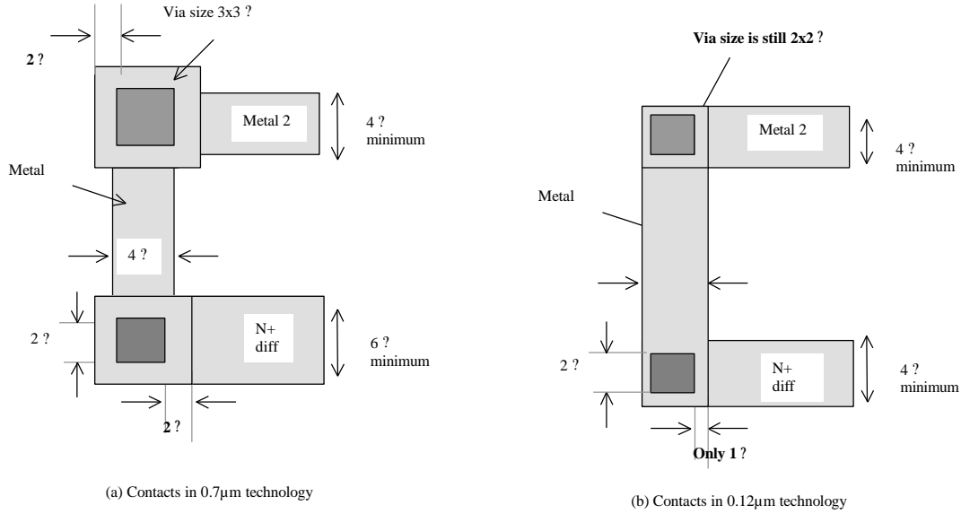
Figure 5-2: Contacts in 0.7µm technology require more area than in 0.12µm technology
