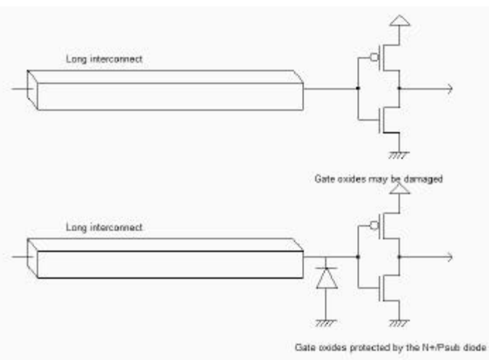
Figure 5-58 Inserting a diode to discharge the interconnect during plasma etching (AntennaRules.SCH)
