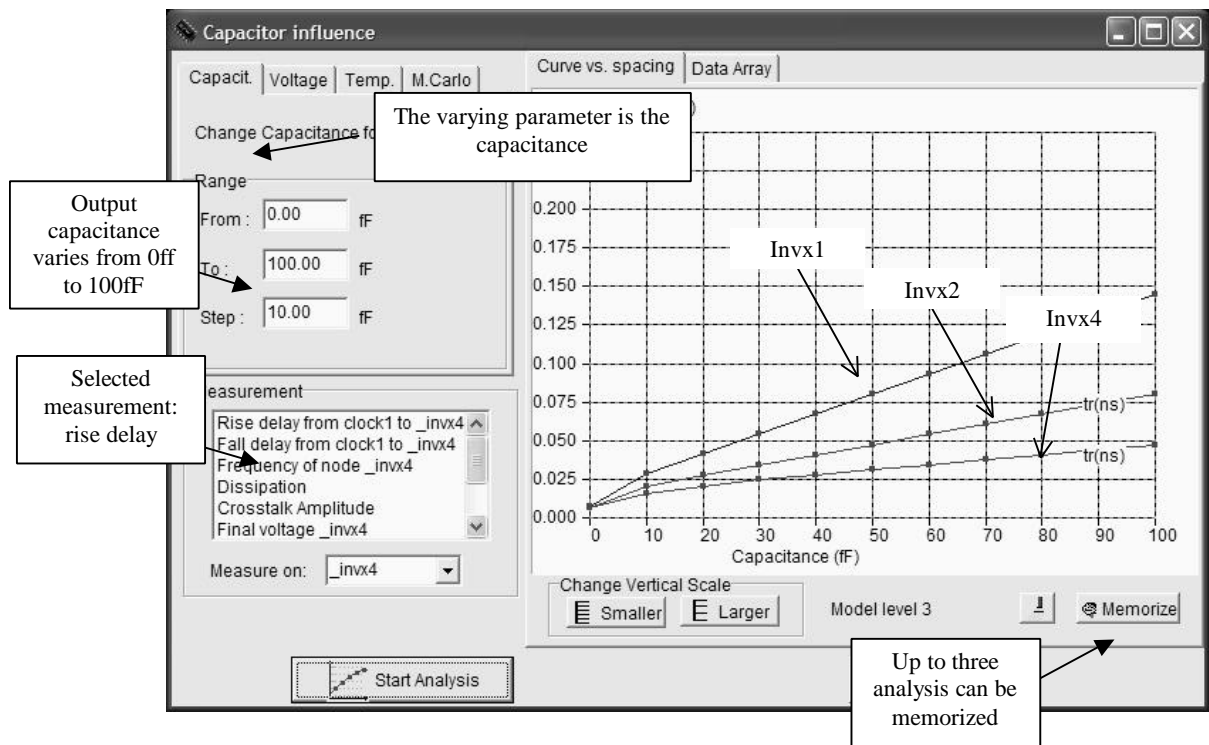
Figure 5-46: Three sizes of inverters used to investigate the delay vs. capacitance load (Invx124.MSK)
