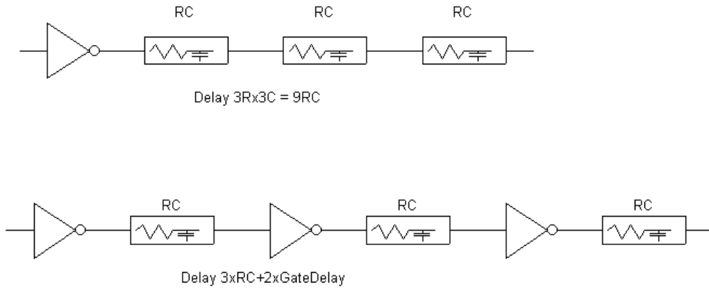
Fig. 5-47 : The propagation delay of a long line with one inverter can be longer than with three inverters (RcLines.SCH)
