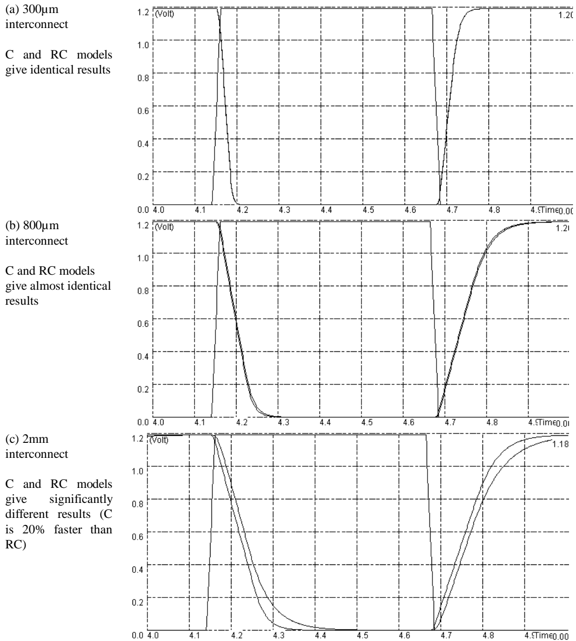
Figure 5-42: Comparative simulation of the C and RC model in signal propagation (RCModel.MSK)
