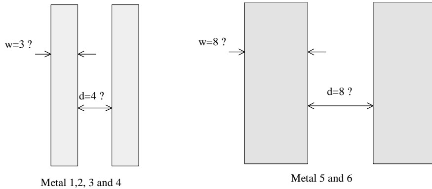
Figure 5-11: Minimum width w and distance d between metal layers
