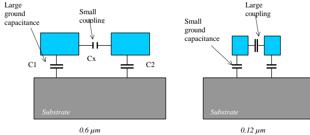
Fig. 5-51 The scale down tends to increase lateral couplings and decrease vertical coupling
