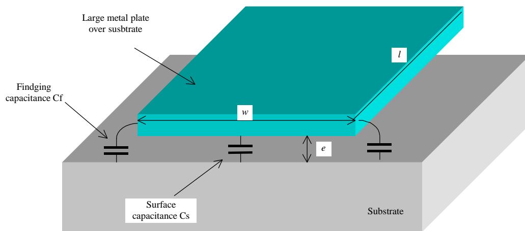
Figure 5-17: Large plate of metal above the substrate
