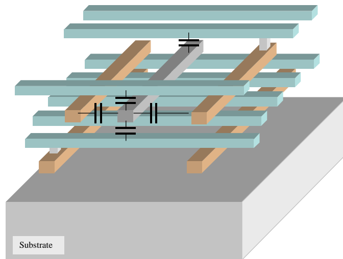
Figure 5-16: One interconnect is coupled to other conductors in several ways, both lateral and vertical
