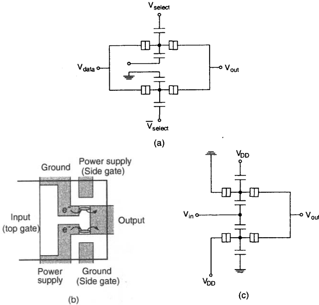
Fig. 3.59 CMOS-type inverter and its equivalent circuit using the SET structure with side gates. (From Ono et al. [37]. ©2000 IEEE.)
