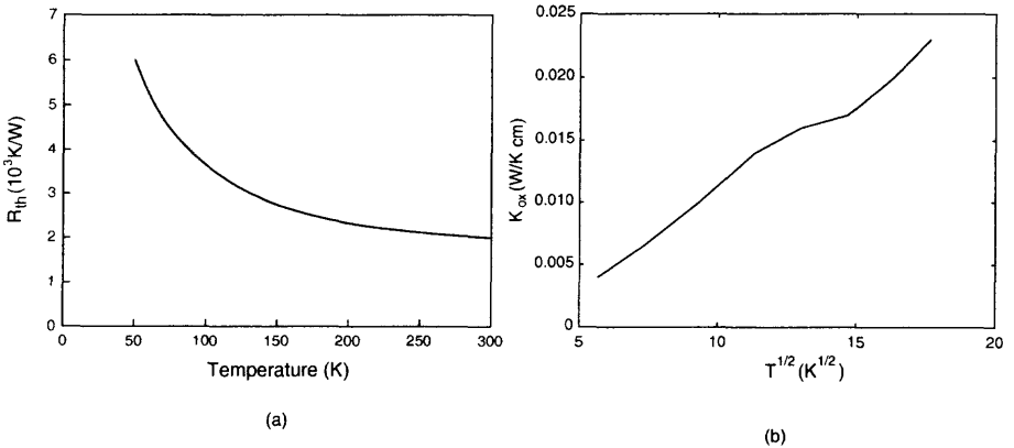
Fig. 2.107 (a) Thermal resistance versus temperature and (b) thermal conductivity versus square root of temperature of the SOI NMOS device with a thin film of 800 \text{ \AA} and a buried oxide of 3800 \text{ \AA} . (Adapted from Jomaah et al. [96].)
