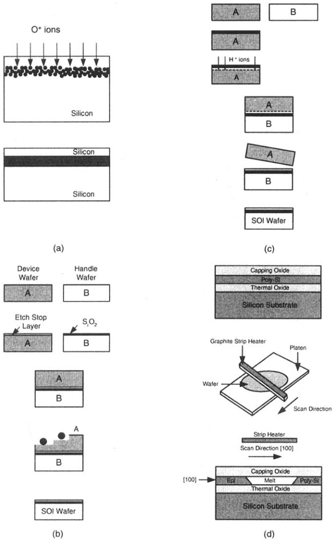
Fig. 2.1 SOI wafer technologies: (a)SIMOX–Synthesis by Implanted Oxygen (Adapted from Watanabe and Tooi [1]), (b)BESOI– Bond and Etch Back (Adapted from Godbey et al. [2]), (c) Smart-Cut (Adapted from Bruel et al. [3][4]), and (d) ZMR–Zone Melting Recrystallization (Adapted from Zavracky et al. [5].)
