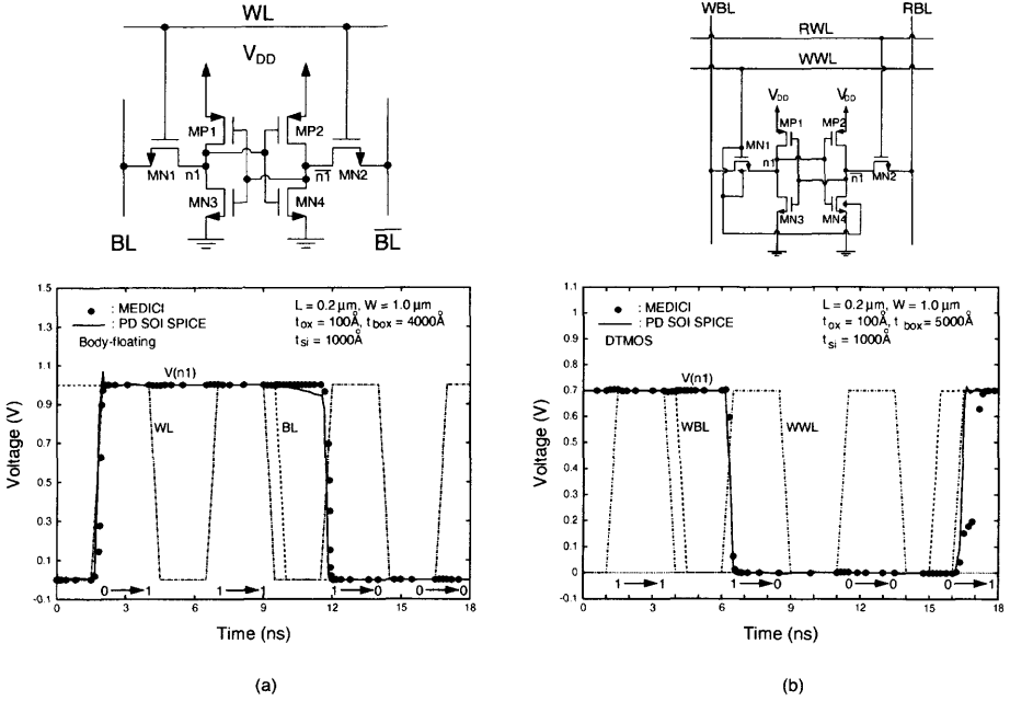
Fig. 7.19 Write transient waveforms for (a) a 6T SRAM memory cell using 0.2 \mu\text{m} body-floating PD SOI CMOS devices with a front gate oxide of 100 \text{\AA} and a thin film of 1000 \text{\AA} and (b) a two-port 6T SRAM memory cell with single-bit-line simultaneous read-and-write access (SBLSRWA) capability using DTMOS PD SOI CMOS devices with a front gate oxide of 100 \text{\AA} and a thin film of 1000 \text{\AA} [16], based on the PD SOI-Technology SPICE model results and the MEDICI simulation results.
