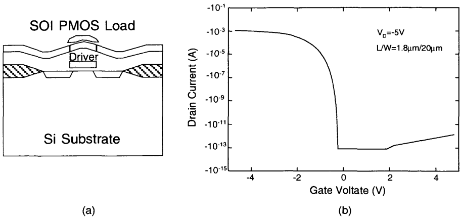
Fig. 5.45 (a) Cross-section of the bulk CMOS technology with SOI PMOS load. (b) Drain current characteristics of the SOI PMOS load with a channel width of 20 \mu\text{m} and a channel length of 1.8 \mu\text{m} , biased at the drain voltage of -5 \text{ V} . (Adapted from Takao et al. [38].)
