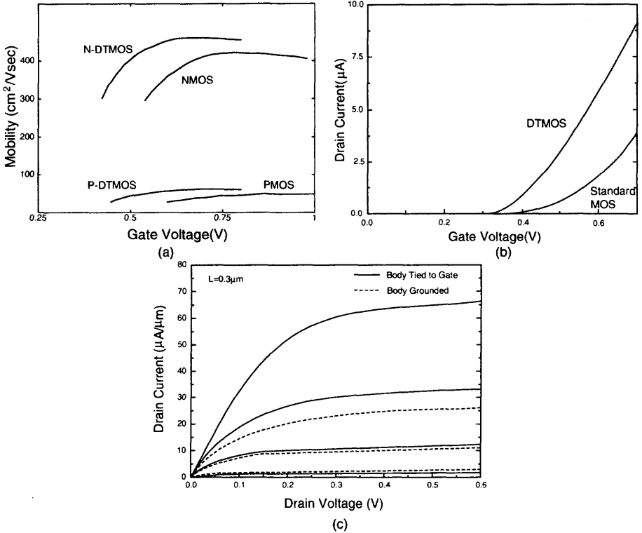
Fig. 3.38 (a) Electron and hole effective mobility versus gate voltage, (b) Drain current versus gate voltage, and (c) Drain current versus drain voltage of the SOI MOS devices in standard MOS configuration with its body grounded and DTMOs configuration. The SOI MOS device has a front gate oxide of 64 Å, a thin film of \sim 1500 Å doped with a density of 3 \times 10^{17} \text{cm}^{-3} . (From Assaderaghi et al. [27]. ©1997 IEEE.)
