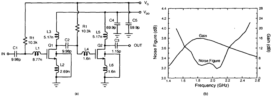
Fig. 6.33 (a) 1.8 GHz two-stage SOI LNA circuit. (b) Gain and noise figure versus frequency of the two-stage SOI LNA circuit. (Adapted from Vorwerk et al. [27].)
