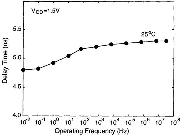
Fig. 2.125 Propagation delay time versus operating frequency of a 64-bit adder implemented by SOI CMOS devices, operating at V_{DD} = 1.5 V. (Adapted from Ueda et al. [110].)
