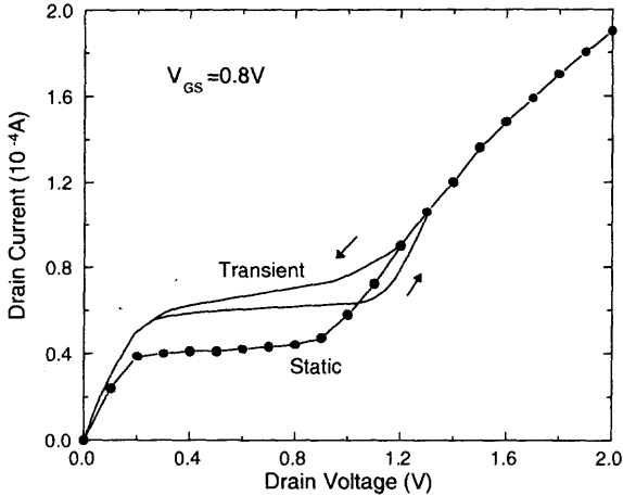
Fig. 2.102 Drain current versus drain voltage of the PD NMOS device with a front gate oxide of 70 \text{ \AA} , a 1000 \text{ \AA} thin film doped with a p-type density of 5 \times 10^{17} \text{ cm}^{-3} , a buried oxide of 4000 \text{ \AA} , a channel length of 1 \mu\text{m} and a channel width of 10 \mu\text{m} , biased at the gate voltage of 0.8 \text{ V} , and with its drain voltage changing from negative to positive and from positive to negative with a scan time of 1 \text{ s} . (Adapted from Perron et al. [92].)
