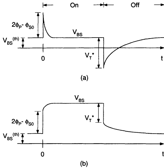
Fig. 2.117 Schematical transient of the body voltage of a PD SOI NMOS device during the turn-on and the turn-off voltage steps applied to the gate with its drain voltage biased (a) below the kink effect region and (b) well above the kink effect region. (Adapted from Perron et al. [104].)
