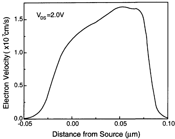
Fig. 2.44 Distribution of the electron velocity in the lateral channel region of an SOI NMOS device with a front gate oxide of 40 Å, a thin film of 300 Å, a buried oxide of 800 Å, and a channel length of 500 Å, biased at a drain voltage of 2 V. (Adapted from Ohuchi [50].)
