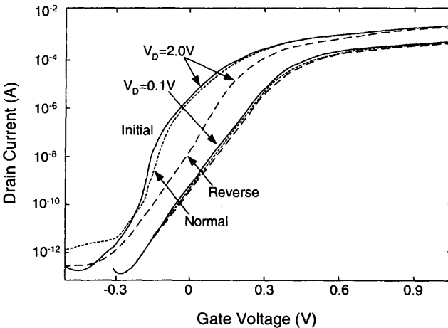
Fig. 3.3 Subthreshold characteristics of the SOI NMOS device with a front gate oxide of 50 Å, a thin film of 500 Å, a buried oxide of 900 Å, a channel width of 10 μm and a channel length of 0.17 μm, before a 3-min stress at the drain voltage of 3 V and the gate voltage of 0.2 V, and after the stress in normal and reverse mode operations. (Adapted from Tsuchiya et al. [3].)
