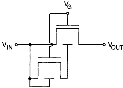
Fig. 5.5 The ADTPT circuit. (Adapted from Wang & Kuo [4].)
