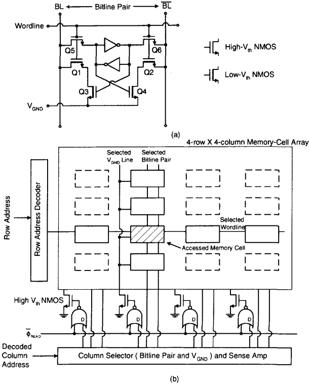
Fig. 5.41 (a) A 10T SRAM cell and (b) architecture of the 1 V 128 K embedded 100-MHz SRAM using SOI MTCMOS techniques. (Adapted from Shibata et al. [36].)
