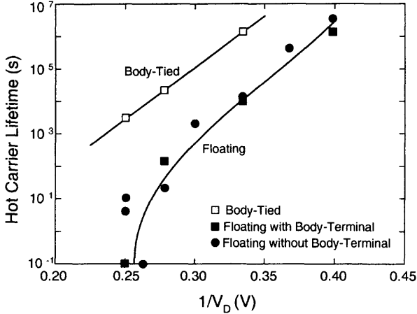
Fig. 3.18 Hot-carrier lifetime to reach the 10% transconductance degradation versus the inverse of the drain voltage of the PD SOI NMOS device with a front gate oxide of 70 Å, a thin film of 2000 Å, a buried oxide of 4000 Å, and a channel length of 0.3 μm, stressed at the gate voltage of 0.7 V, with its body floating and tied. (Adapted from Maeda et al. [15].)
