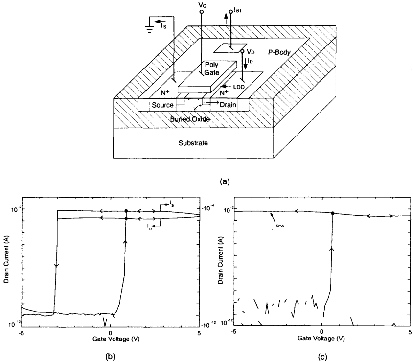
Fig. 2.101 (a) Cross-section of the SOI NMOS device with a front gate oxide of 200 \text{ \AA} , a 3000 \text{ \AA} thin film doped with a p-type density of 10^{17} \text{ cm}^{-3} , a channel width of 10 \text{ \mu m} and a channel length of 1.2 \text{ \mu m} . (b) Drain current versus gate voltage of the device with its body tied to source, biased at the drain voltage of 7.1 \text{ V} . (c) Drain current versus gate voltage of the device with its body floating, biased at the drain voltage of 7.1 \text{ V} . (From Huang et al. [91]. ©1991 IEEE.)
