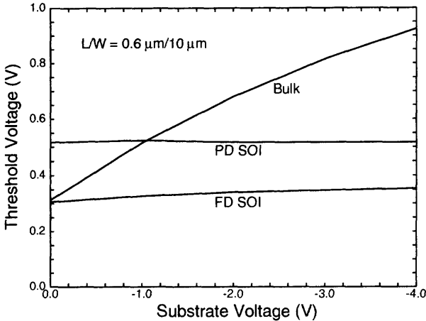
Fig. 2.6 Threshold voltage versus back gate bias of partially depleted (PD), fully depleted (FD) SOI and bulk NMOS devices. (Adapted from Eimori et al. [13].)
