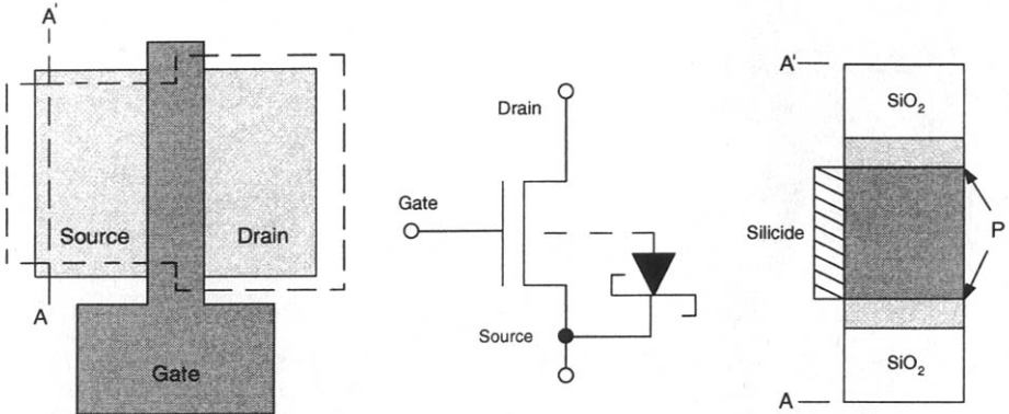
Fig. 2.57 A PD SOI NMOS device with Schottky body contact at the source. The dashed line indicates the n^+ implant mask. (Adapted from Sleight et al. [58].)
