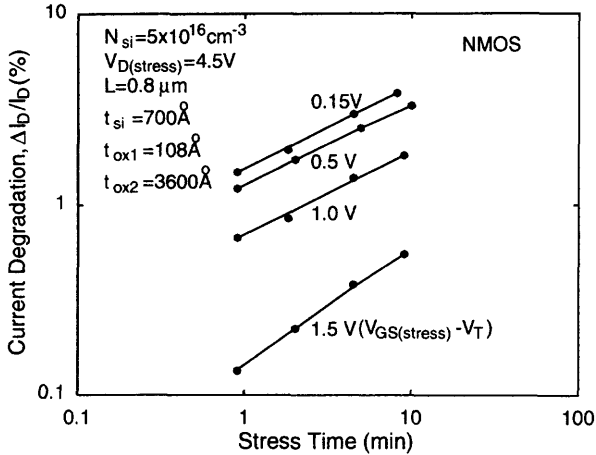
Fig. 3.11 Degradation of drain current versus stress time of the FD SOI NMOS device with a front gate oxide of 108 Å, a thin film of 700 Å doped with a p-type density of 5 \times 10^{16} \text{ cm}^{-3} , a buried oxide of 3600 Å, and a channel length of 0.8 μm, stressed with the drain voltage of 4.5 V and various gate voltages. (Adapted from Su et al. [10].)
