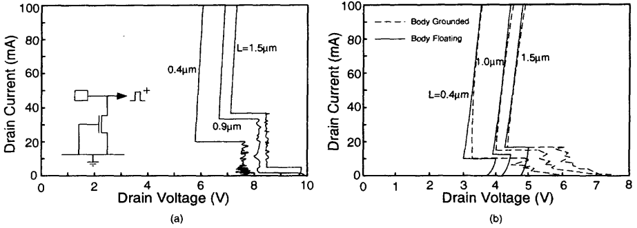
Fig. 4.48 Breakdown/snapback characteristics of (a) bulk and (b) SOI NMOS devices with its body floating and grounded, for various channel lengths. (Adapted from Chan et al. [33].)
