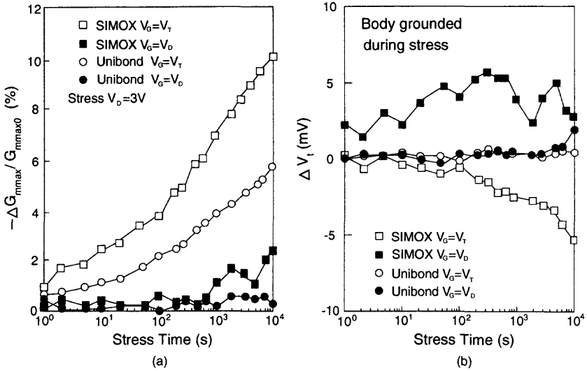
Fig. 3.14 (a) Degradation of transconductance and (b) threshold voltage shift versus stress time of the SOI NMOS device with a front gate oxide of 45 Å, a thin film of 400 Å, and a buried oxide of 3800 Å, based on SIMOX and Unibond wafers, stressed at the drain voltage of 3V and two gate voltages and the body grounded. (From Renn et al. [12]. ©1998 IEEE.)
