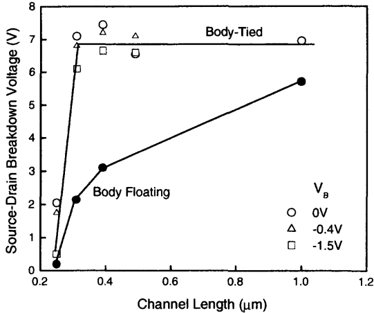
Fig. 2.85 Breakdown voltage versus channel length of the SOI NMOS device with a channel width of 10\ \mu\text{m} , biased with body floating and body tied to various voltages. (Adapted from Maeda et al. [79].)
