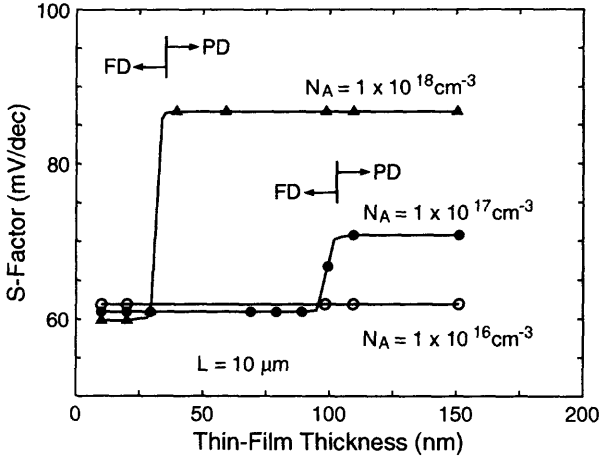
Fig. 2.26 The influence of the thin-film doping density in the inverse subthreshold slope for FD and PD SOI NMOS devices with a front gate oxide of 50 \text{ \AA} and a buried oxide of 5000 \text{ \AA} . (Adapted from Joachim et al. [32].)
