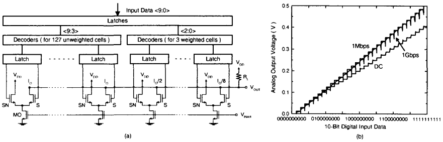
Fig. 6.15 (a) Kink-effect-free 10-bit SOI current-steering DAC using non-FD (NFD) SOI CMOS devices. (b) Its output-input transfer characteristics operating at DC, 1Mbps, and 1Gbps. (Adapted from Chang et al. [13].)
