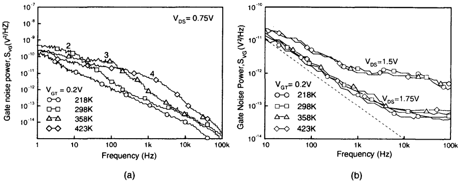
Fig. 3.87 Gate noise power versus frequency of the PD SOI NMOS device with a front gate oxide of 105 Å, a thin film of 1000 Å, and a buried oxide of 3600 Å, with its body floating, biased at the drain voltages of (a) 0.75 V and (b) 1.5 and 1.75 V, and the gate overdrive voltage of 0.2 V, for various temperatures. (From Tseng et al. [60]. ©2000 IEEE.)
