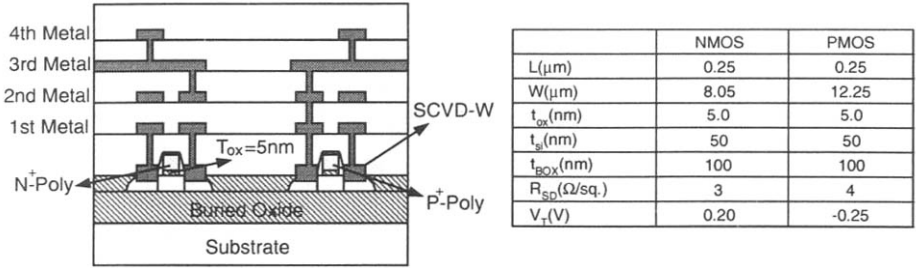
Fig. 5.48 Cross-section of a 0.25 \mu\text{m} FD SOI CMOS technology for implementing a 300 kG gate array. (Adapted from Sato et al. [43].)
