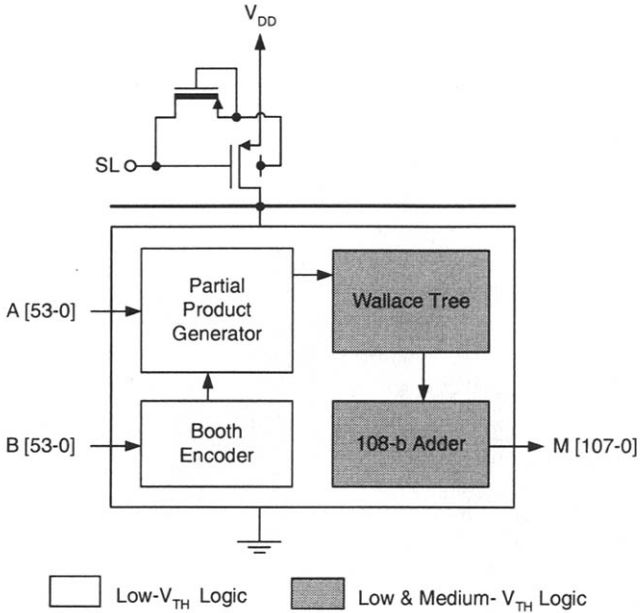
Fig. 5.66 Organization of a 0.5V 54b × 54b multiplier using SOI MTCMOS techniques with triple-threshold devices. (Adapted from Fujii et al. [57].)
