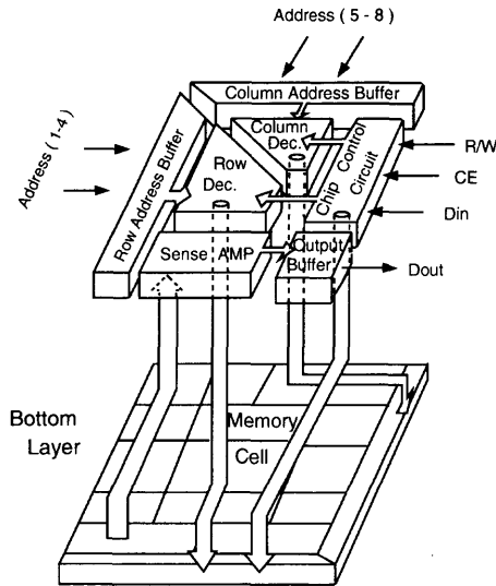
Fig. 5.46 3D SRAM structure. (Adapted from Nishimura et al. [39].)
