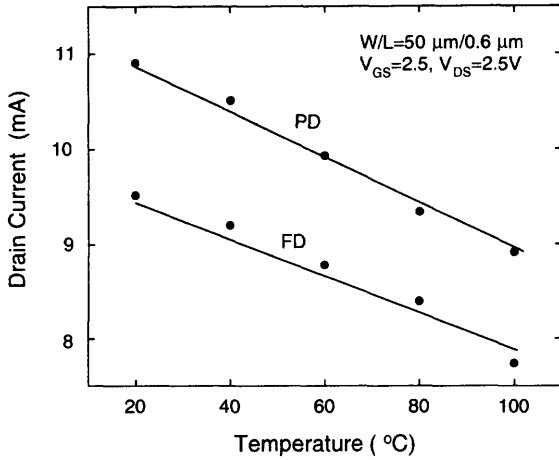
Fig. 3.80 Drain current versus temperature of PD and FD SOI NMOS devices with a channel width of 50 μm and a channel length of 0.6 μm, biased at the drain voltage of 2.5 V and the gate voltage of 2.5 V. (Adapted from Jin et al. [53].)
