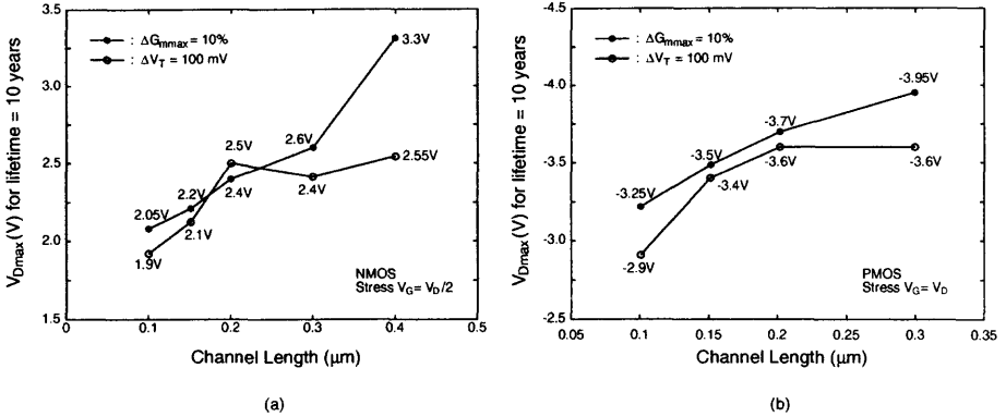
Fig. 3.16 Maximal drain voltage to obtain a lifetime of 10 years versus channel length of the SOI (a) NMOS and (b) PMOS devices with conditions and results extrapolated from Fig. 3.15. (Adapted from Renn et al. [13].)
