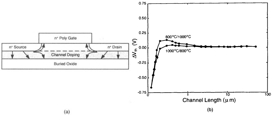
Fig. 2.23 (a) Schematic of excess interstitial flux due to implant damage or arsenic deactivation causing enhanced channel dopant diffusion in an SOI device. (b) Threshold voltage change versus channel length of an SOI NMOS device having a 1000°C rapid thermal anneal and a 800°C furnace anneal and in an opposite order after the source/drain implant. (Adapted from Crowder et al. [29].)
