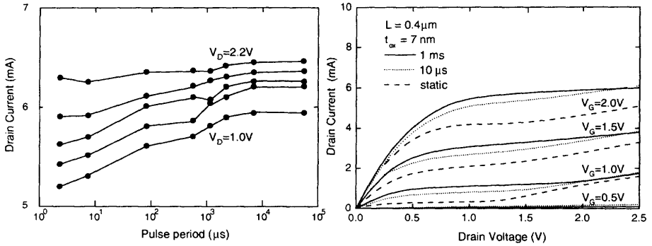
Fig. 2.120 Drain current characteristics of the PD SOI NMOS device with a front gate oxide of 70 Å, a 1400 Å thin film doped with a p-type density of 4 \times 10^{17} \text{ cm}^{-3} , biased at various drain voltages, using pulse measurement by imposing periodic pulses from low to high with a pulse width of 7 ns and periods of 1 ms and 10 μs. (Adapted from Jenkins et al. [106].)
