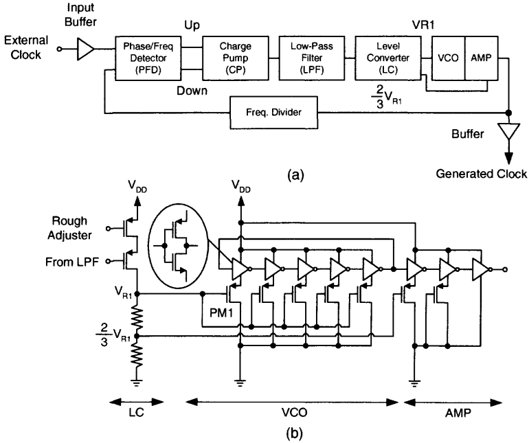
Fig. 6.40 (a)Block diagram of a PLL. (b) VCO used in a 2 V 3.5 Gbps optical transceiver using a 0.2 \mu\text{m} FD SOI CMOS technology. (Adapted from Ohtomo et al. [33].)
