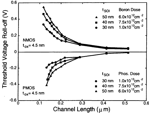
Fig. 2.15 Threshold voltage roll-off of FD SOI NMOS device with a front gate oxide of 45 Å and various thin-film thicknesses. (Adapted from Imai et al. [21].)
