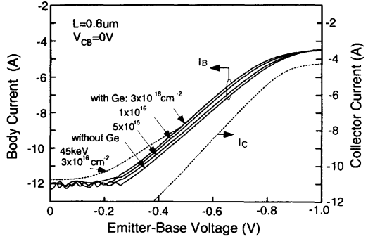
Fig. 2.60 Gummel plot of the parasitic bipolar device in the PD SOI NMOS device with and without the Ge-implanted source/drain. The width of the bipolar device is 6 \mu\text{m} . The dose of the germanium implant is 3 \times 10^{16} \text{cm}^{-3} . Two implant energies of 25 and 45 KeV have been used. (Adapted from Nishiyama et al. [60].)
