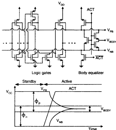
Fig. 5.31 Equalized body circuit architecture used in the DRAM. (Adapted from Yamauchi et al. [28].)
