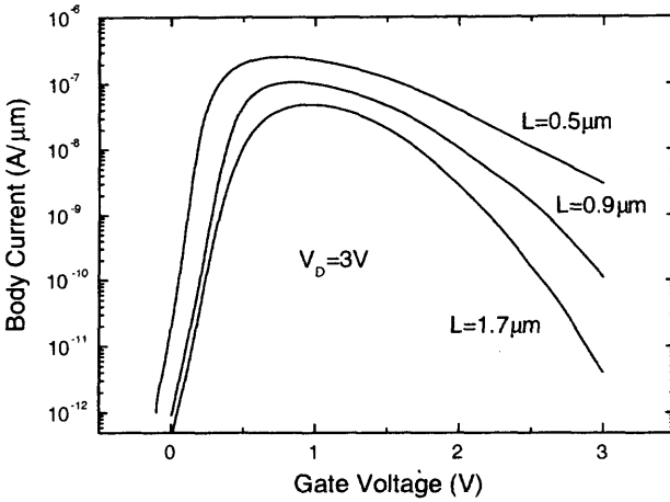
Fig. 3.7 Body current versus gate voltage of an SOI NMOS device with a front gate oxide of 90 Å, a thin film of 760 Å, and various channel lengths, biased at the drain voltage of 3 V. (Adapted from Wann et al. [7].)
