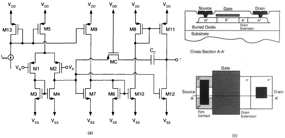
Fig. 6.6 (a) Two-stage SOI CMOS op amp. (b) Body-tied-to-source SOI device. (Adapted from Verbeck et al. [5].)
