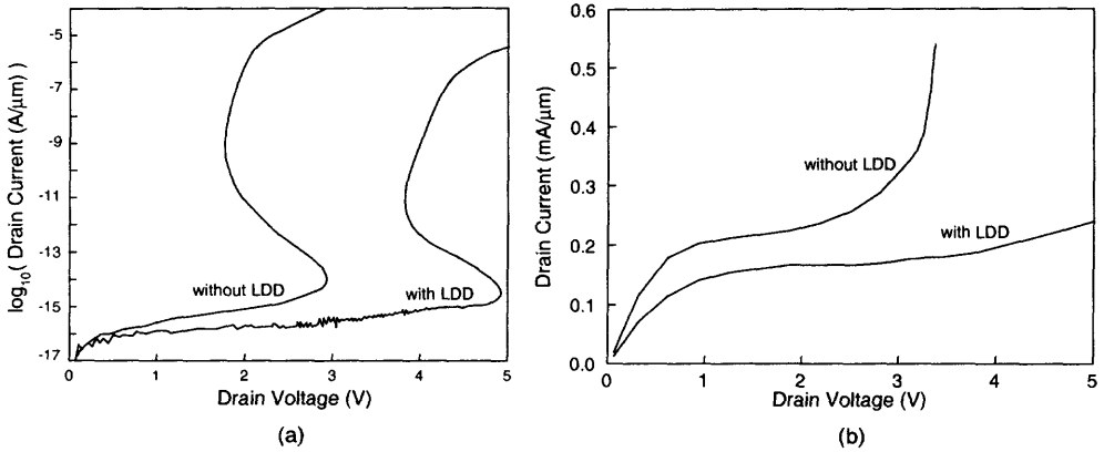
Fig. 2.91 Drain current characteristics of the FD SOI NMOS device with and without the LDD structure (a) at off-state with the gate voltage of -3\text{ V} and (b) at on-state with the gate voltage of V_T + 2\text{ V} . (Adapted from Choi & Fossum [84].)
