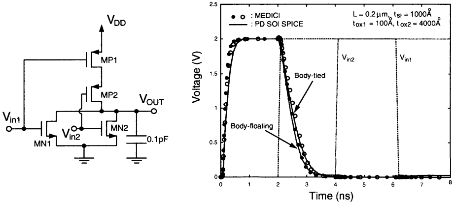
Fig. 7.17 Transient waveforms of a NOR circuit using body-floating and body-tied PD SOI CMOS devices with a front gate oxide of 100 \text{ \AA} , a thin film of 1000 \text{ \AA} , a buried oxide of 4000 \text{ \AA} , and a channel length of 0.2 \text{ }\mu\text{m} , based on the PD SOI-Technology SPICE model results and the MEDICI simulation results.
