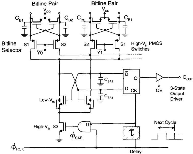
Fig. 5.42 Selector-merged MTCMOS sense amp in the readout circuit with the cross-coupled pullup pairs at the bitlines in the 1 V 128 K embedded 100-MHz SRAM. (From Shibata et al. [36]. ©2000 IEEE.)
