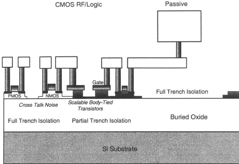
Fig. 4.57 Cross-section of the 0.18 \mu\text{m} SOI CMOS technology with digital, embedded RF/analog, and SOC capabilities. (Adapted from Maeda et al. [42].)
