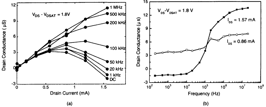
Fig. 2.112 Small signal drain conductance of the PD SOI NMOS device with a front gate oxide of 250 Å, a thin film of 1780 Å, a buried oxide of 4150 Å, a channel width of 20 μm, and a channel length of 5 μm, biased in the saturation ( V_{DS} - V_{DSAT} = 1.8 V ), with the body tied to the source, plotted (a) versus the drain current and (b) versus the frequency. (Adapted from Tenbroek et al. [101].)
