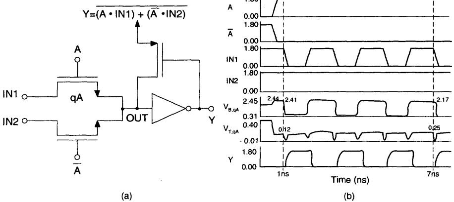
Fig. 4.11 (a) A single-ended LEAP circuit using SOI NMOS devices. (b) Waveforms of the body potential and the threshold voltage of the device qA and the output signal (Y) of the LEAP circuit with the gate signals (A, \bar{A} ) and the input signals (IN1, IN2) imposed to the SOI NMOS devices. (Adapted from Puri & Chuang [8].)
