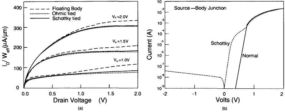
Fig. 2.58 (a) Drain current characteristics of a PD SOI NMOS device with a thin film of 1500 Å, a buried oxide of 2000 Å, and a channel length of 0.3 \mu m , with a floating body and a Schottky body contact and (b) the current characteristics of the source-body junction using the Schottky body contact approach and the conventional p - n^+ approach. (Adapted from Sleight et al. [58].)
