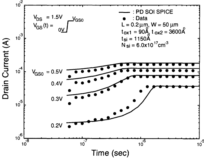
Fig. 7.12 Drain current waveforms during the turn-on transient of the PD SOI NMOS device with a front gate oxide of 90 Å, a buried oxide of 3600 Å, a thin film of 1150 Å doped with a p-type density of 6 \times 10^{17} \text{ cm}^{-3} , a channel length of 0.2 μm, and a channel width of 50 μm, biased at various gate voltage and with its body floating, based on the PD SOI-Technology SPICE model results and the experimental data [12].
