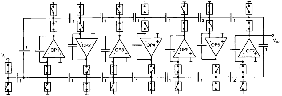
Fig. 6.10 SOI switched-capacitor seventh-order low-pass ladder filter. (From Verbeck et al. [5]. ©1996 IEEE.)
