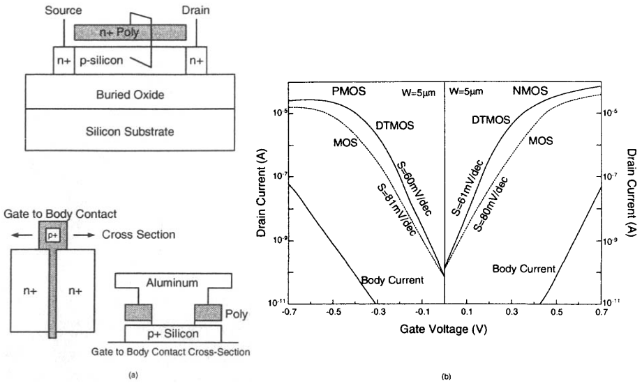
Fig. 3.37 (a) Cross-section and layout of an SOI NMOS device with body and gate tied together. (b) Subthreshold characteristics of SOI NMOS and PMOS devices operating in DTMOS configuration. (From Assaderaghi et al. [27]. ©1997 IEEE.)
