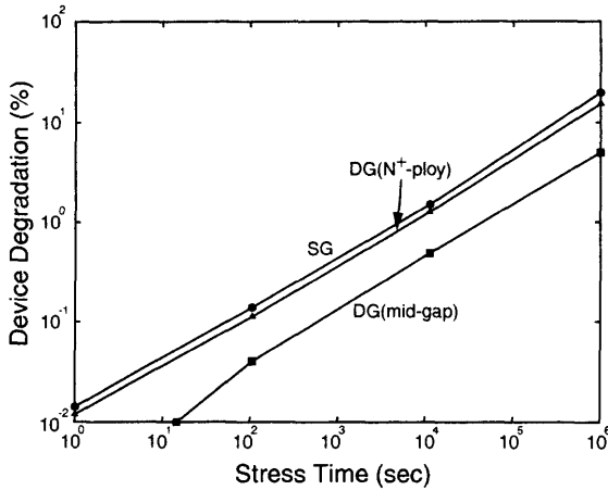
Fig. 3.36 Drain current degradation versus stress time of double-gate and single-gate SOI NMOS devices with a front gate oxide of 40 Å, a 250 Å thin film doped with a buried oxide of 1000 Å, a channel length of 0.08 μm, after hot-carrier stress at V_{GS} = 1.2 V and V_{DS} = 0.05 V [26]. The single-gate device has the gate made of a mid-gap material and the thin-film doping density of 10^{16} cm -3 . One double-gate device has the N + polysilicon gate and the thin-film doping density of 10^{18} cm -3 . The other double-gate device has the gate made of the mid-gap material and the thin-film doping density of 10^{16} cm -3 (Adapted from Williams et al. [26].)
