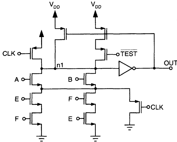
Fig. 5.10 SOI dynamic logic circuit. (Adapted from Aipperspach [15].)
