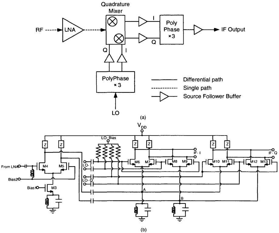
Fig. 6.37 (a) Block diagram of an RF receiver. (b) 1 V SOI CMOS quadrature mixer. (From Ugajin et al. [30]. ©2001 IEEE.)
