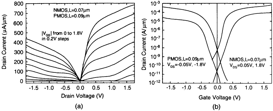
Fig. 3.47 Drain current (a) versus drain voltage and (b) versus gate voltage of the PD SOI CMOS devices with a front gate oxide of 35\text{ \AA} . (Adapted from Assaderaghi et al. [31].)
