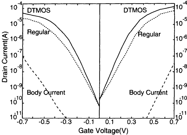
Fig. 4.23 Subthreshold characteristics of SOI NMOS and PMOS devices with body grounded and body tied to the gate (DTMOS). (Adapted from Assaderaghi et al. [16].)
