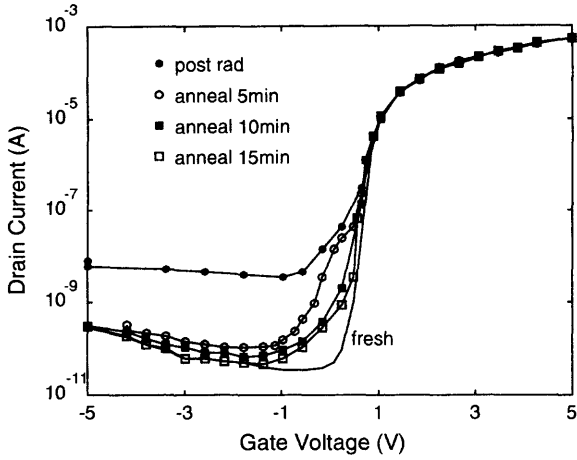
Fig. 3.98 Drain current versus gate voltage of an SOS NMOS device with various annealing times at 140°C after Co 60 irradiation of 100 krad. (Adapted from Chao et al. [67].)
