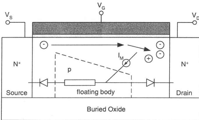
Fig. 2.49 Cross-section of an SOI NMOS device showing the current conduction path.
