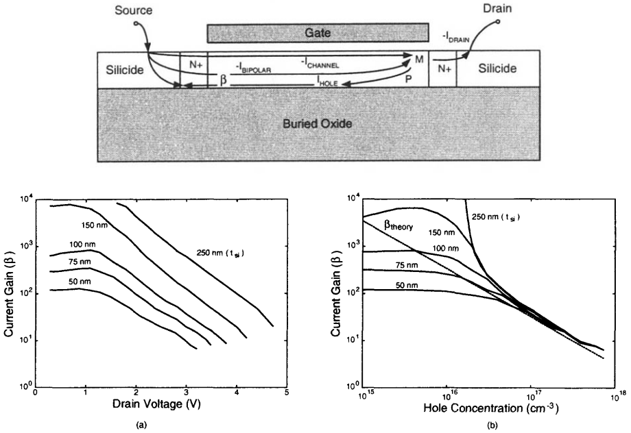
Fig. 2.81 Current gain of the parasitic bipolar device versus (a) drain voltage and (b) hole concentration of the FD SOI NMOS device with a channel length of 1 \mu\text{m} , a thin-film doping density of 10^{16} \text{cm}^{-3} , and various thin-film thicknesses, biased at the gate voltage of the threshold voltage. (From Ver Ploeg [76]. ©1994 IEEE.)
