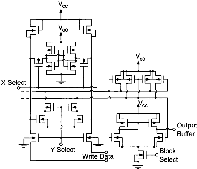
Fig. 5.36 Memory cell and sense amp in an early-stage SOI SRAM circuit. (Adapted from Isobe et al. [31].)
