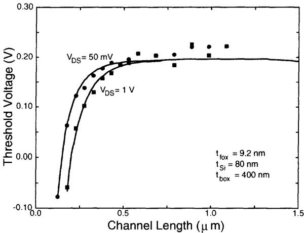
Fig. 2.14 Short channel effect of a FD SOI NMOS device with a front gate oxide of 92\text{ \AA} , a buried oxide of 4000\text{ \AA} , and a thin film of 800\text{ \AA} , biased at V_{\text{DS}} = 0.05 and 1\text{ V} . (Adapted from Banna et al. [20].)
