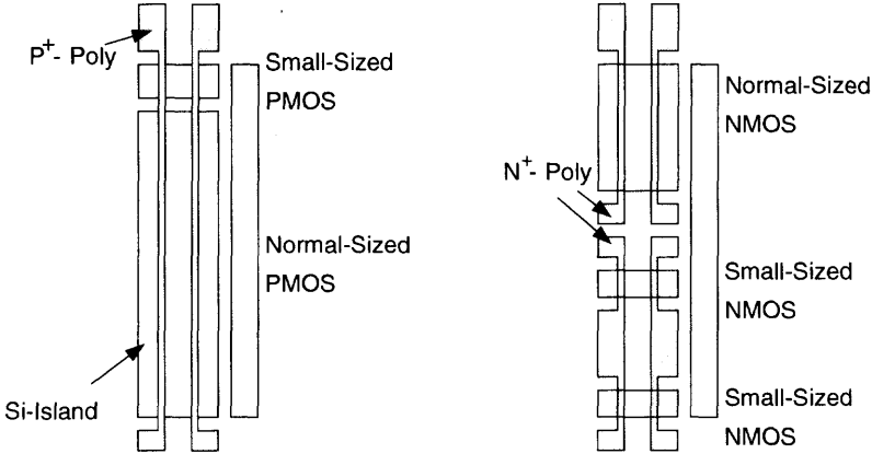
Fig. 5.49 Layout of the cell of a typical gate array using the 0.25 μm FD SOI CMOS technology. (Adapted from Kado et al. [44].)
