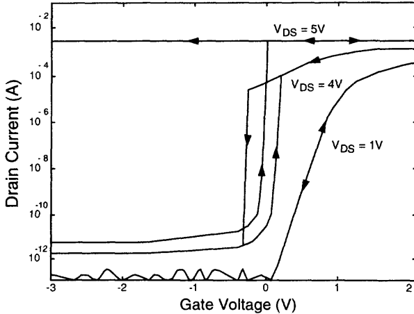
Fig. 2.100 Drain current versus gate voltage of the SOI NMOS device with a front gate oxide of 260 Å, a thin film doped with a p-type density of 10^{17} \text{ cm}^{-3} , biased at the drain voltages of 1, 4, and 5 V, and its gate voltage first changing from negative to positive, then back to negative. (Adapted from Chen et al. [90].)
