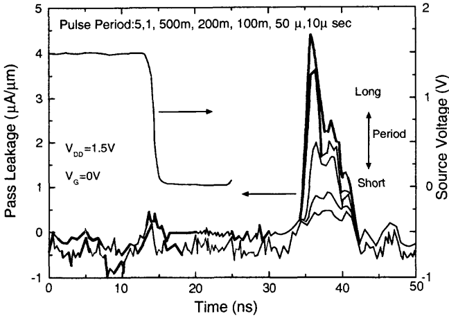
Fig. 2.97 Transient leakage current of the PD SOI NMOS pass transistor with a front gate oxide of 80 \text{ \AA} , a thin film of 1600 \text{ \AA} , and a buried oxide of 5000 \text{ \AA} , biased at the drain voltage of V_{DD} = 1.5 \text{ V} , and the gate voltage of 0 \text{ V} , with its source driven by periodic inverse pulses from 1.5 to 0 \text{ V} with a pulse width of 100 \text{ ns} , a rise/fall time of 2 \text{ ns} , and various pulse periods from 10 \text{ }\mu\text{s} to 5 \text{ s} . (Adapted from Saraya & Hiramoto [88].)
