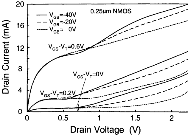
Fig. 2.53 Drain current characteristics of a 0.25\ \mu\text{m} PD SOI NMOS device with a front gate oxide of 45\ \text{\AA} , a thin film of 400\ \text{\AA} , and a buried oxide of 3800\ \text{\AA} , biased at various back gate biases. (Adapted from Rozean et al. [55].)
