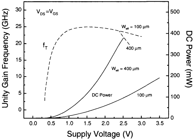
Fig. 6.22 Unity gain frequency ( f_T ) and DC power consumption versus supply voltage ( V_{DS} = V_{GS} ) of the SOI NMOS device with a front gate oxide of 100 Å and a channel length of 0.2 μm. (Adapted from Eggert et al. [18].)
