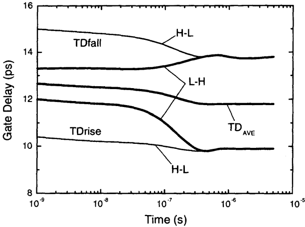
Fig. 2.104 Gate delay versus time of the inverter using PD SOI CMOS devices with a front gate oxide of 45 Å, a thin film of 1500 Å, a buried oxide of 4000 Å, and a channel length of 0.145 \mu\text{m} , biased at V_{DD} = 1.8 V, with its input driven by a clock with a period of 1 ns and a 50% duty cycle [93]. A 2:1 aspect ratio difference between the PMOS and the NMOS devices has been adopted. (Adapted from Pelella et al. [93].)
