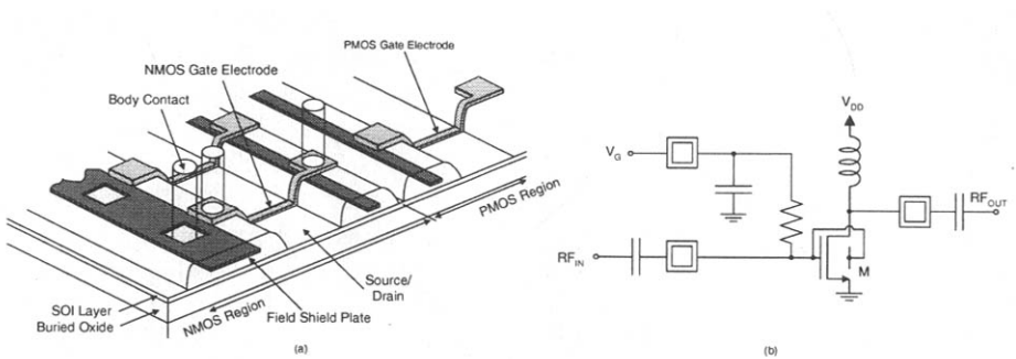
Fig. 6.26 (a) Field-shielded PD SOI CMOS devices. (b) SOI LNA circuit with the active-body PD SOI NMOS device operating at a supply voltage 1 V. (From Komurasaki et al. [22]. ©1998 IEEE.)
