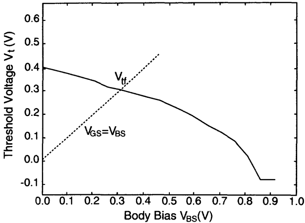
Fig. 4.22 Threshold voltage versus body-source voltage of an SOI NMOS device with a front gate oxide of 64 Å and a p-type thin-film doping density of 3 \times 10^{17} \text{cm}^{-3} . (Adapted from Assaderaghi et al. [15].)
