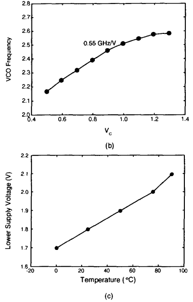
Fig. 6.41 (a) 2.5 GHz SOI VCO using a 0.18 \mu\text{m} SOI CMOS technology. (b) Operating frequency versus control voltage of the SOI VCO. (c) Lower-limit supply voltage versus temperature of the SOI VCO operating at 2.5 GHz. (From Yoshimura et al. [34]. ©1999 IEEE.)
