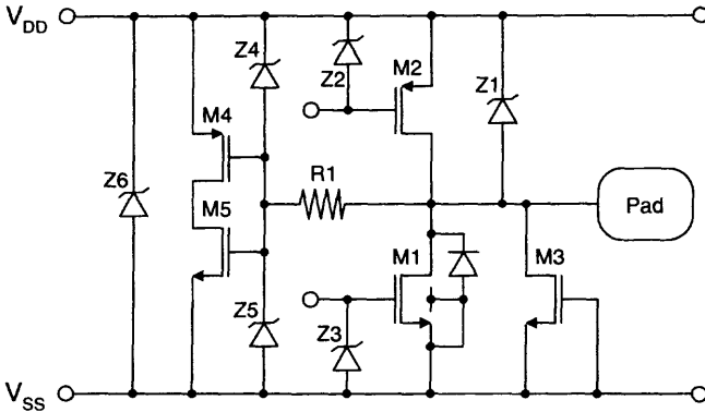
Fig. 4.51 SOI ESD protection circuit. (Adapted from Smith et al. [37].)
