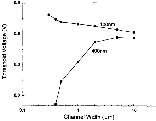
Fig. 2.39 Threshold voltage versus channel width of LOCOS isolated SOI NMOS device with a front gate oxide of 60 Å, a thin film of 1000 Å, and buried oxide thicknesses of 1000 and 4000 Å. (Adapted from Lee et al. [45].)
