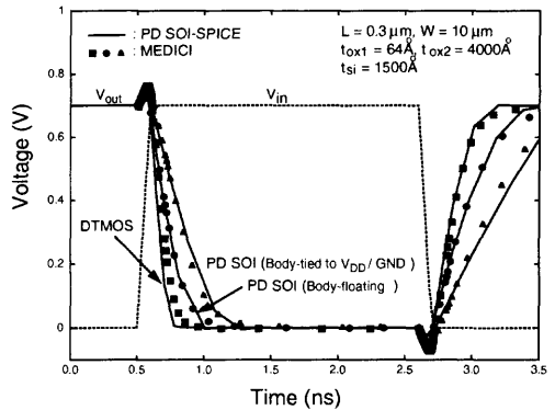
Fig. 7.16 Output transient waveforms of an inverter circuit using body-floating PD, body-tied PD and DTMOS PD SOI CMOS devices with a front gate oxide of 64 Å, a thin film of 1500 Å, a buried oxide of 4000 Å, a channel length of 0.3 μm, and a channel width of 10 μm, biased at V_{DD} = 0.7 \text{ V} , based on the PD SOI-Technology SPICE model results and the MEDICI simulation results.
