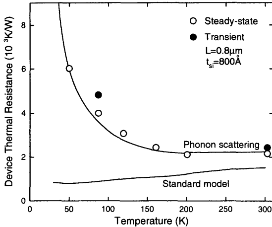
Fig. 3.82 Thermal resistance versus temperature of the SOI NMOS device with a thin film of 800 Å and a buried oxide of 3800 Å. (Adapted from Asheghi et al. [55].)
