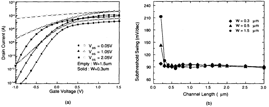
Fig. 2.35 (a) Subthreshold characteristics with an SOI NMOS device with channel widths of 0.3 and 1.5 \mu m , a front gate oxide of 101 \text{\AA} , and a thin film of 779 \text{\AA} . (b) Inverse subthreshold slope versus channel length of the SOI NMOS device with various channel widths. (Adapted from Hwang et al. [14].)
