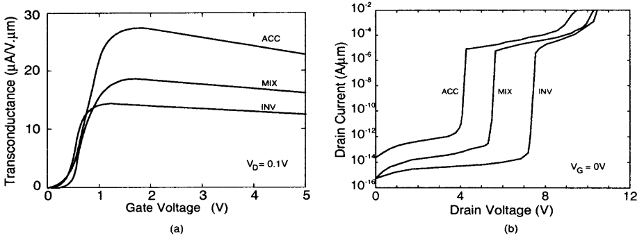
Fig. 3.28 (a) Transconductance versus gate voltage ( V_D = 0.1\text{ V} ), (b) Drain current versus drain voltage (with both front and back gates grounded) of the accumulation-mode FD SOI NMOS device with a front gate oxide of 200\text{ \AA} , a 1000\text{ \AA} thin film doped with an n-type density of 10^{15}\text{ cm}^{-3} , a buried oxide of 4000\text{ \AA} , and a channel length of 0.8\text{ }\mu\text{m} . For the inversion mode device, the thin-film doping density is 2 \times 10^{16}\text{ cm}^{-3} . (Adapted from Duan & Ioannou [20].)
