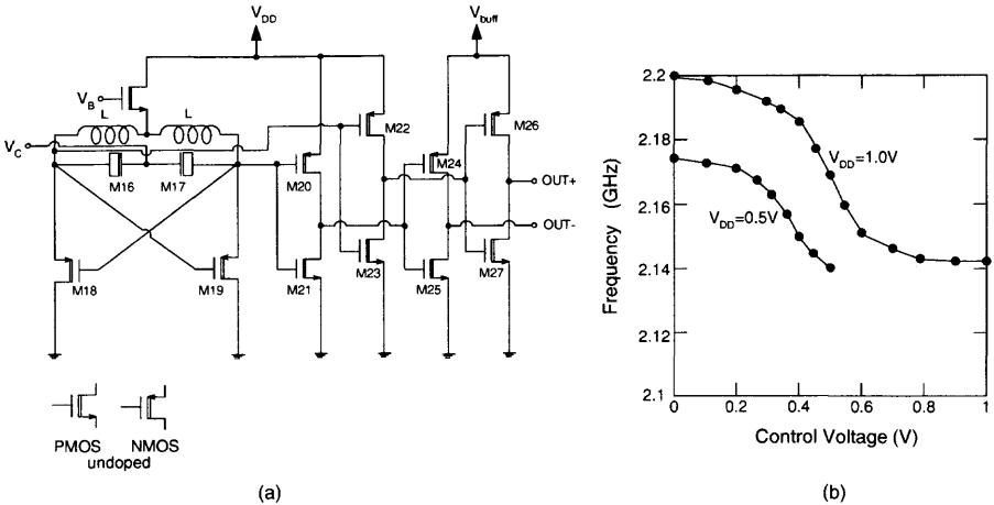
Fig. 6.42 (a) 0.5 V 2 GHz SOI VCO based on integrated inductors using a 0.2 \mu\text{m} FD SOI CMOS technology. (b) Output frequency versus control voltage of the SOI VCO for supply voltages of 1 and 0.5 V. (Adapted from Harada et al. [21].)
