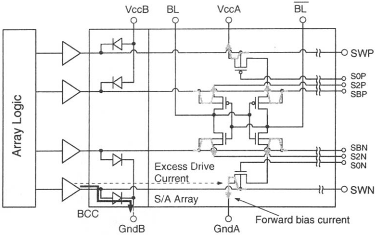
Fig. 5.28 Body current clamber (BCC) used in a 16-Mb SOI DRAM which is based on stabilizing the body voltages of devices used in the sense amp. (Adapted from Shimomura et al. [27].)
