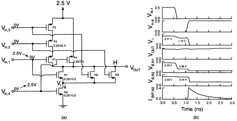
Fig. 4.8 (a) The three-way OR-AND circuit using SOI CMOS devices with a channel length of 0.25 \mu\text{m} , a front gate oxide of 50 \text{\AA} , a buried oxide of 3500 \text{\AA} , and a thin film of 1400 \text{\AA} . (b) Waveforms at the output node, the internal node V_1 , and the body nodes of devices N1 and N2 during the transient after the input waveforms are imposed at V_{in,1} and V_{in,4} . Also shown in this figure is the transient current of the parasitic bipolar device in device N2. (Adapted from Lu et al. [7].)
