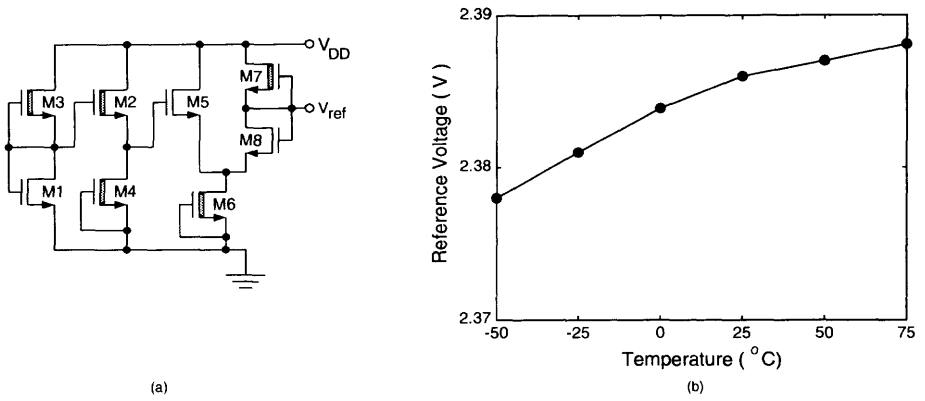
Fig. 6.45 (a) SOI reference voltage generator using SOI accumulation- and inversion-mode devices with a front gate oxide of 350 Å and a thin film of 700 Å doped with a p-/n-type doping density of 10^{17} \text{ cm}^{-3} for the inversion-/accumulation-mode device. (b) Reference voltage versus temperature. (Adapted from Song & Kim [37].)
