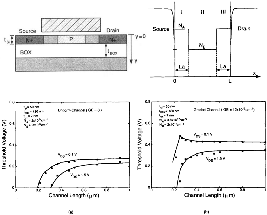
Fig. 2.21 Threshold voltage versus channel length of the FD SOI NMOS device with a front gate oxide of 70 \text{ \AA} , a thin film of 500 \text{ \AA} , a buried oxide of 1200 \text{ \AA} , and (a) a uniformly doped channel and (b) a graded channel. (From Adan et al. [27]. ©1999 IEEE.)
