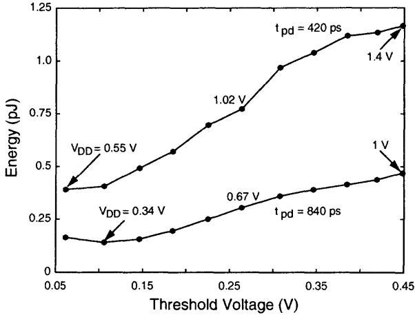
Fig. 3.56 Energy of a 101-stage ring oscillator versus threshold voltage of the dual-gate SOI CMOS device. (Adapted from Dancy & Chandrakasan [36].)
