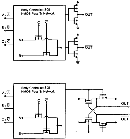
Fig. 5.61 Body bias-controlled (BC) SOI pass gate logic using PD SOI DTMOS techniques. (Adapted from Fuse et al. [56].)
