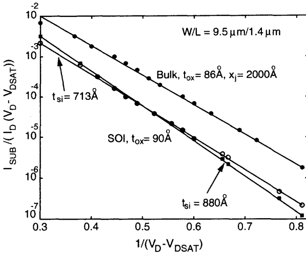
Fig. 2.79 Ratio of the body current to the drain current ( I_{\text{sub}}/I_{\text{D}} ) versus the inverse of the difference between the drain voltage and the saturation voltage [ 1/(V_{\text{D}} - V_{\text{DSAT}}) ] of the SOI NMOS device with a front gate oxide of 90 \text{ \AA} and the bulk NMOS device with a front gate oxide of 86 \text{ \AA} , with a channel length of 1.4 \mu\text{m} , and a channel width of 9.5 \mu\text{m} . (Adapted from Ma et al. [75].)
