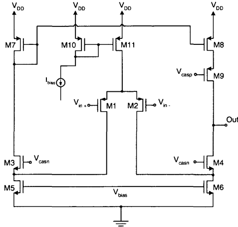
Fig. 6.3 SOI CMOS folded-cascode op amp with a symmetrical topology. (Adapted from Eggermont et al. [3].)
