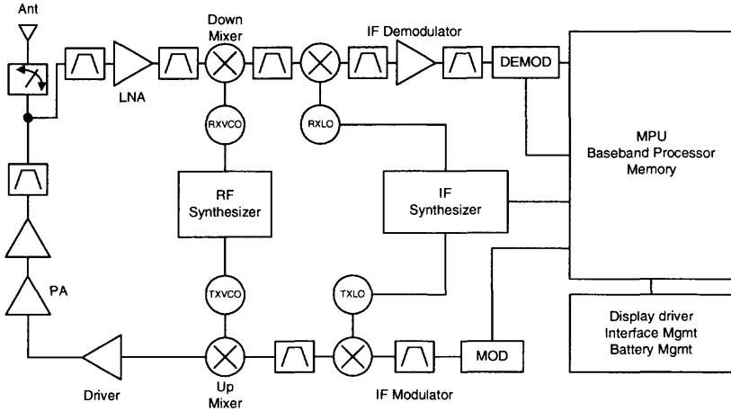
Fig. 6.19 Typical radio frequency (RF) circuit in a wireless communication system. (Adapted from Huang et al. [16].)
