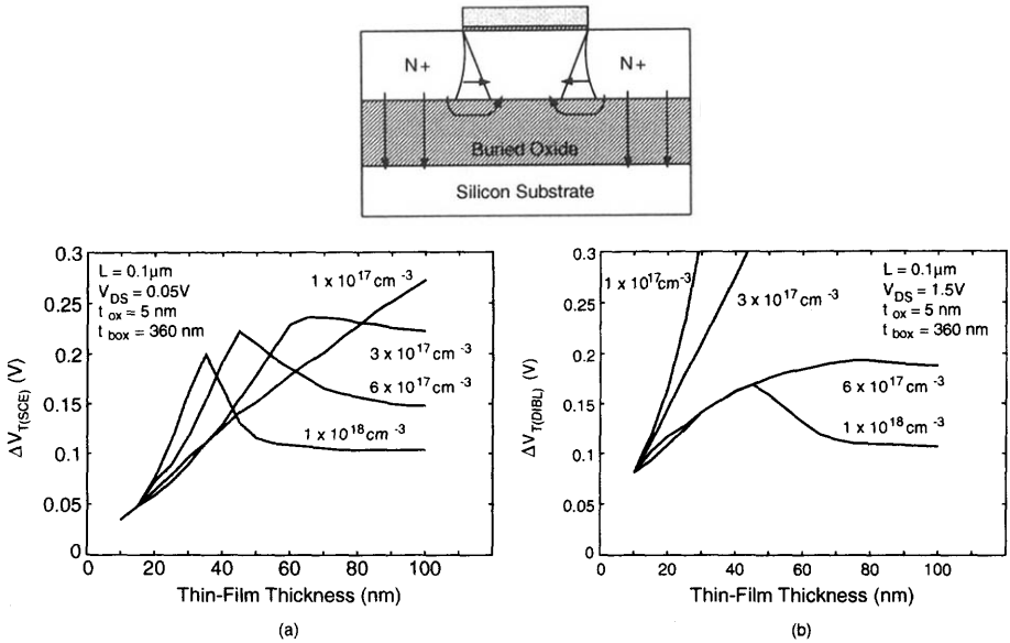
Fig. 2.16 Threshold voltage shift versus thin-film thickness of an SOI NMOS device with a front gate oxide of 50 \text{ \AA} and a buried oxide of 3600 \text{ \AA} , for various channel doping densities, biased at (a) V_{DS} = 0.05 \text{ V} , and (b) 1.5 \text{ V} . (Adapted from Su et al. [22].)
