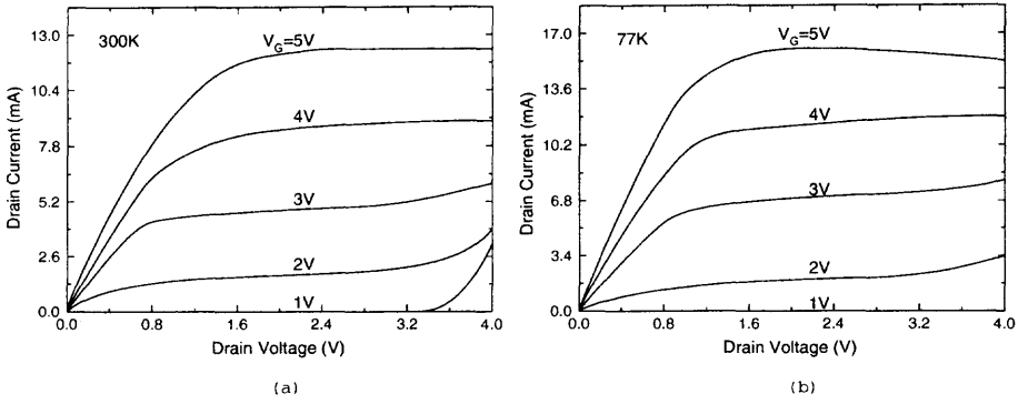
Fig. 2.106 Drain current versus drain voltage of an SOI NMOS device with a front gate oxide of 175 \text{ \AA} , a thin film of 800 \text{ \AA} , and a buried oxide of 3800 \text{ \AA} , operating at (a) 300 K and (b) 77 K. (Adapted from Jomaah et al. [95].)
