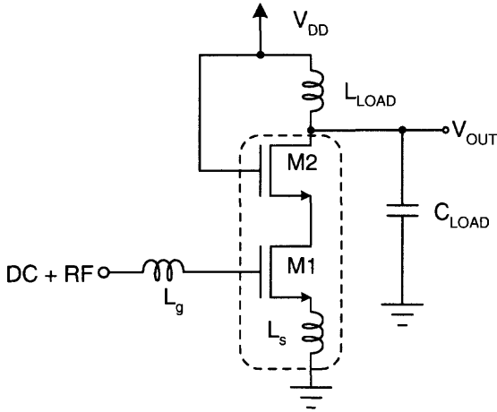
Fig. 6.31 1.5 V 1.8 GHz single-stage cascoded LNA circuit using a PD SOI CMOS technology. (Adapted from Jin et al. [26].)
