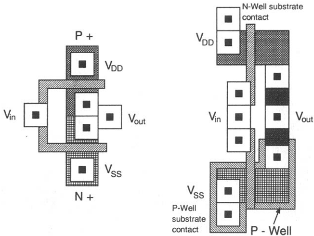
Fig. 4.1 Layout of a CMOS inverter circuit using SOI and bulk technologies. (Adapted from Stern et al. [1].)
