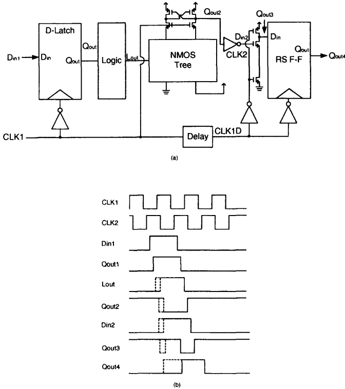
Fig. 5.15 SOI dynamic logic circuit illustrating the race problem. (From Park et al. [17]. ©1999 IEEE.)
