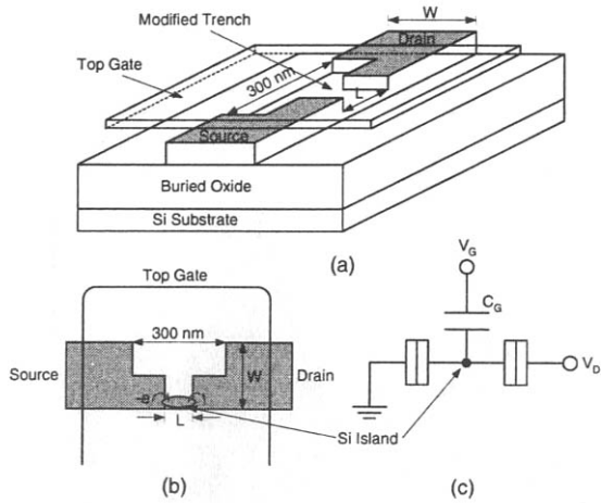
Fig. 3.57 Structure of an SET with its equivalent circuit. (From Ono et al. [37]. ©2000 IEEE.)
