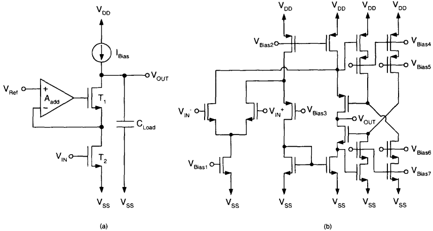
Fig. 6.7 (a) Principle of the gain boosting scheme. (b) SOI folded cascode op amp with the p and n cascoded gain-boosting stages. (From Gentinne et al. [6]. ©1993 IEEE.)
