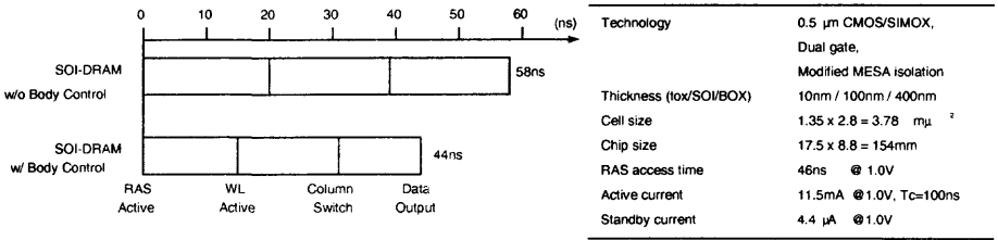
Fig. 5.30 Access time and performance of the 16-Mb SOI DRAM with the body control techniques using a 0.5 \mu\text{m} SOI CMOS technology. (Adapted from Shimomura et al. [27].)
