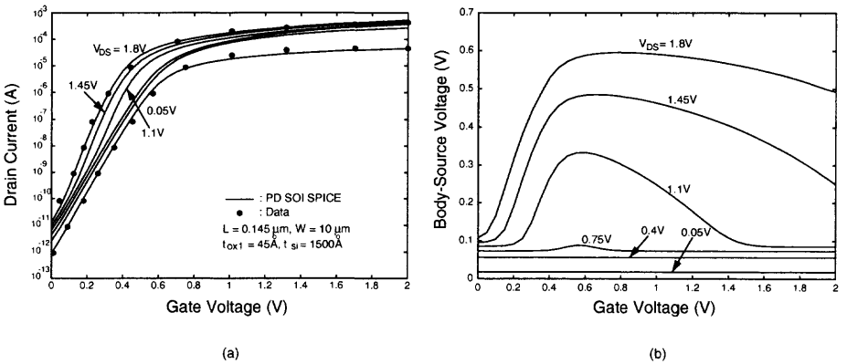
Fig. 7.6 (a) Drain current (b) body-source voltage characteristics of a PD SOI NMOS device with a front gate oxide of 45 \text{ \AA} , a thin film of 1500 \text{ \AA} , a channel length of 0.145 \mu\text{m} , and a channel width of 10 \mu\text{m} , biased in the subthreshold region, with its body node floating, based on the PD SOI-Technology SPICE model results, and the experimental data [7].
