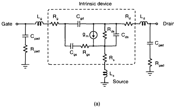
Fig. 6.21 (a) Small-signal equivalent circuit of an SOI CMOS device used in RF circuits. (b) Extracted parameters of the SOI CMOS devices for RF circuits, biased at V_{DS} = 2\text{ V}/V_{GS} = 1\text{ V} (NMOS) and V_{DS} = -2\text{ V}/V_{GS} = -1.5\text{ V} (PMOS). (Adapted from Eggert et al. [18].)
