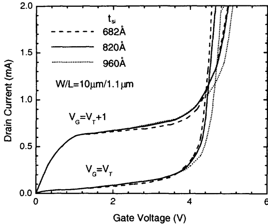
Fig. 2.83 Drain current characteristics of an SOI NMOS device with a channel width of 10 \mu\text{m} , a channel length of 1.1 \mu\text{m} , and with various thicknesses of the thin-film doped with a p-type density of 10^{17} \text{cm}^{-3} . (Adapted from Chen et al. [78].)
