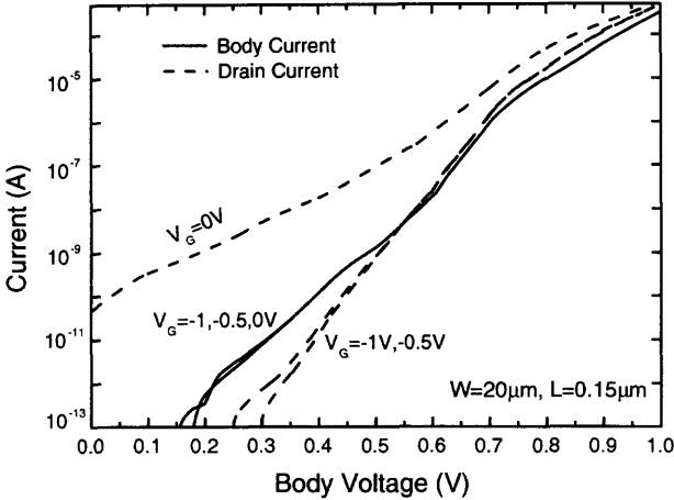
Fig. 2.94 Drain and body currents of the SOI NMOS pass transistor with a front gate oxide of 45 Å, a thin film of 1800 Å, a buried oxide of 3700 Å, a channel width of 20 μm, and a channel length of 0.15 μm, biased at gate voltages of 0, -0.5, and -1 V. (Adapted from Assaderaghi et al. [86].)
