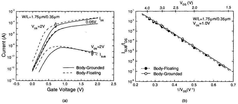
Fig. 3.5 (a) Drain and body currents versus gate voltage and (b) the ratio of the body current to the drain current versus the inverse of the drain voltage of the SOI NMOS device with a front gate oxide of 60 \text{ \AA} , a 2000 \text{ \AA} thin film doped with a p-type density of 2 \times 10^{17} \text{ cm}^{-3} , a buried oxide of 2000 \text{ \AA} , and a channel length of 0.35 \mu\text{m} . (Adapted from Sherony et al. [5].)
