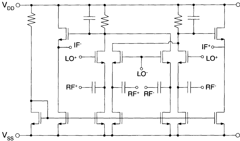
Fig. 6.38 SOS CMOS RF mixer using Gilbert's cell. (Adapted from Johnson et al. [25].)
