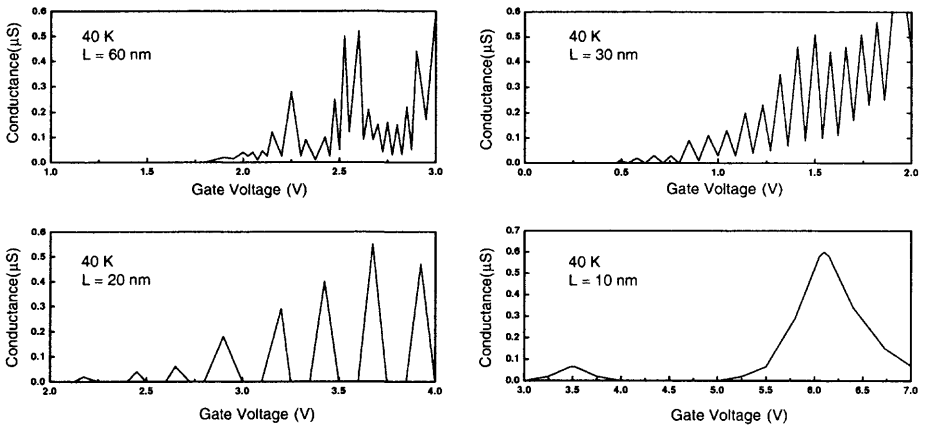
Fig. 3.58 Conductance versus gate voltage of the SET for various channel lengths operating at 40 K. (From Ono et al. [37]. ©2000 IEEE.)
