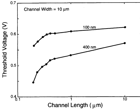
Fig. 2.17 Threshold voltage versus channel length of an SOI NMOS device with a front gate oxide of 60 \text{ \AA} and a thin film of 1000 \text{ \AA} , and a buried oxide of 1000 and 4000 \text{ \AA} . (Adapted from Lee et al. [23].)
