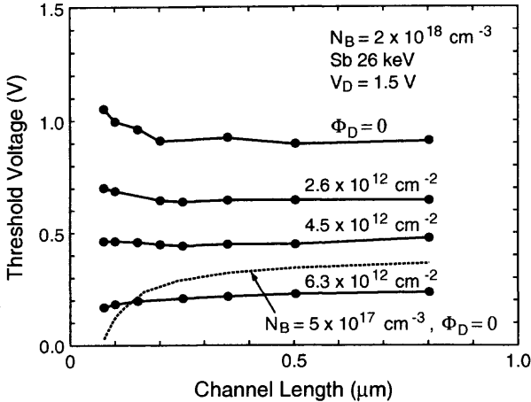
Fig. 2.22 Threshold voltage versus channel length of a PD SOI NMOS device with a front gate oxide of 40 \text{ \AA} and a nonuniformly doped thin film of 1000 \text{ \AA} with a counter-doped thin film using a n-type implant with various doses. (Adapted from Suzuki et al. [28].)
