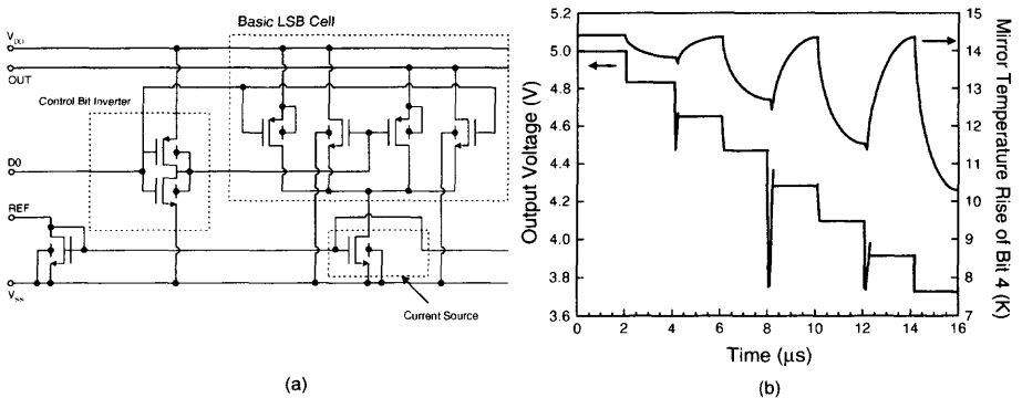
Fig. 6.14 (a) 7-bit SOI current-steering DAC using a 0.7 \mu m SOI CMOS technology. (b) Output waveforms of the DAC. (Adapted from Tenbroek et al. [12].)
