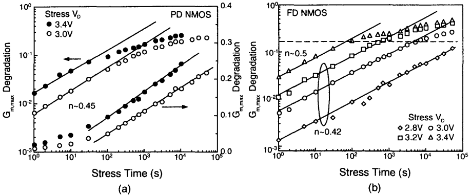
Fig. 3.9 Degradation of maximum transconductance versus stress time of (a) the PD SOI NMOS device with a front gate oxide of 45 Å, a buried oxide of 800 Å, a thin film of 1000 Å, and a channel length of 0.2 μm, stressed with the gate voltage at the threshold voltage and at the drain voltages of 3 and 3.4 V, and (b) the FD SOI NMOS device with a front gate oxide of 45 Å, a thin film of 400 Å, and a buried oxide of 3800 Å, stressed with the gate voltage at the threshold voltage and at various drain voltages. (From Renn et al. [9]. ©1998 IEEE.)
