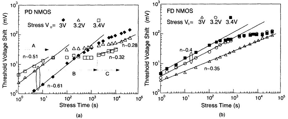
Fig. 3.10 Threshold voltage shift versus stress time of (a) the PD SOI NMOS device with a front gate oxide of 45 \text{ \AA} , a buried oxide of 800 \text{ \AA} , a thin film of 1000 \text{ \AA} and a channel length of 0.2 \mu\text{m} , stressed with the gate voltage at the threshold voltage and at various drain voltages, and (b) the FD SOI NMOS device with a front gate oxide of 45 \text{ \AA} , a thin film of 400 \text{ \AA} , and a buried oxide of 3800 \text{ \AA} , stressed with the gate voltage at the threshold voltage and at various drain voltages. (From Renn et al. [9]. ©1998 IEEE.)
