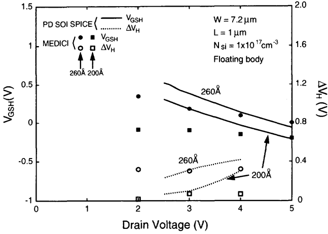
Fig. 7.9 V_{GS} at the onset of hysteresis during the positive scan ( V_{GSH} ) and the width of hysteresis ( \Delta V_H ) vs V_{DS} of the PD SOI NMOS device with a thin film doped with a p-type density of 10^{17} \text{ cm}^{-3} , a channel length of 1 \mu\text{m} , a channel width of 7.2 \mu\text{m} , and front gate oxide thicknesses of 260 and 200 \text{ \AA} , biased with its body floating.
