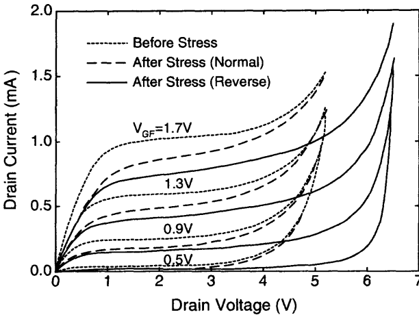
Fig. 3.2 Drain current characteristics of the SOI NMOS device with a front gate oxide of 250 Å, a thin film of 850 Å, and a buried oxide of 3600 Å, before and after a stress of 1500 s with the gate voltage of 1 V, the drain voltage of 6.5 V, the source voltage of 0 V, and the back gate voltage of 0 V, in normal and reverse mode operations. (Adapted from Zhang & Ma [2].)
