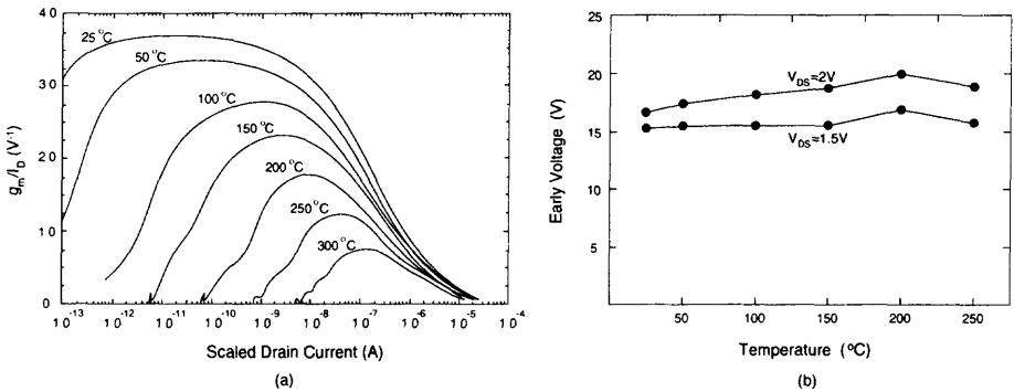
Fig. 3.81 (a) g_m/I_D versus scaled drain current of the SOI NMOS device with a front gate oxide of 300 Å, a thin film of 800 Å, doped with a p-type density of 10^{17} \text{ cm}^{-3} , a buried oxide of 4000 Å, and a channel length/width of 20 μm, for various temperatures. (b) Early voltage versus temperature of the SOI NMOS device with a channel width of 50 μm and a channel length of 2 μm, biased at the drain current of 50 μA. (Adapted from Eggermont et al. [54].)
