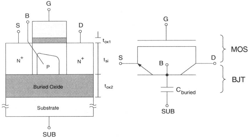
Fig. 7.1 Cross-section of the partially depleted (PD) SOI NMOS device under study and the PD SOI model used in the PD SOI-Technology SPICE models using a concise BiCMOS approach.
