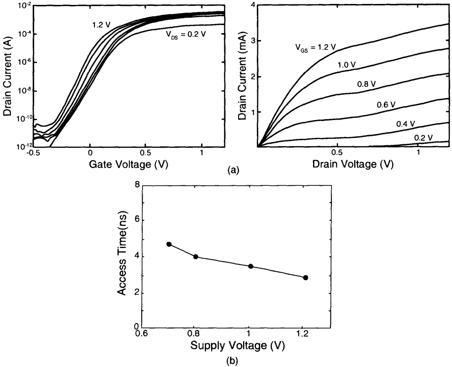
Fig. 5.35 (a) Characteristics of a 0.1 \mu\text{m} PD SOI NMOS device with a front gate oxide of 42 \text{ \AA} . (b) Access time versus supply voltage of the 512 K SRAM using a 0.2 \mu\text{m} SOI CMOS technology. (From Shahidi et al. [30]. ©1993 IEEE.)
