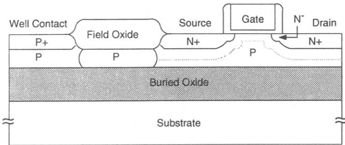
Fig. 5.22 (a) Cross-section of body-contacted (BC) SOI CMOS Devices. (Adapted from Koh et al. [24].)
