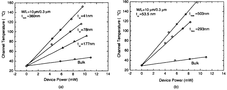
Fig. 2.108 Channel temperature versus power of the SOI NMOS device with a channel length of 0.3\ \mu\text{m} , a channel width of 10\ \mu\text{m} , (a) with a buried oxide of 3600\ \text{\AA} and various thin-film thicknesses, and (b) with a thin film of 535\ \text{\AA} and two buried-oxide thicknesses. (Adapted from Su et al. [97].)
