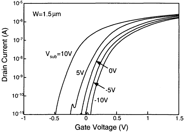
Fig. 2.7 Subthreshold characteristics of an SOI NMOS device with a channel length of 2\ \mu\text{m} , a front gate oxide of 101\ \text{\AA} , a buried oxide of 3800\ \text{\AA} , and a thin film of 791\ \text{\AA} implanted with p-type dopants with a dose of 4 \times 10^{12}\ \text{cm}^{-2} , biased at various back gate biases. (Adapted from Wang et al. [14].)
