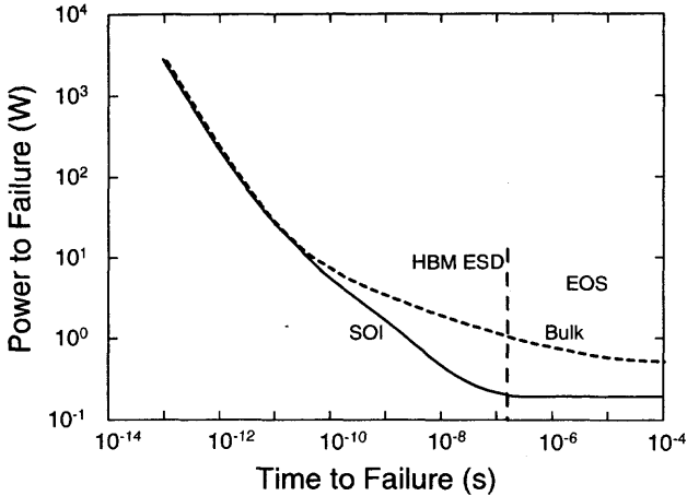
Fig. 3.68 Power to failure versus time to failure of an SOI NMOS device with a front gate oxide of 60 Å, a thin film of 500 Å doped with a p-type density of 4 \times 10^{17} \text{cm}^{-3} , a buried oxide of 800 Å, a channel length of 0.4 \mu\text{m} , a channel width of 30 \mu\text{m} , and a contact-to-gate spacing of 2 \mu\text{m} . (Adapted from Ramaswamy et al. [44].)
