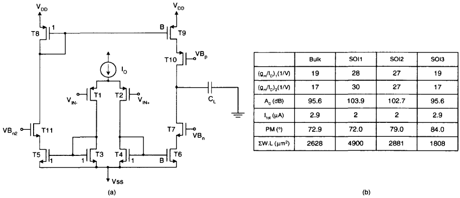
Fig. 6.5 (a) Single-stage op amp with the symmetric topography. (b) Comparison of the performance of the single-stage op amp with an identical transition frequency, using bulk and SOI CMOS devices for various op amp designs with an identical channel length. (Adapted from Silveria et al. [4].)
