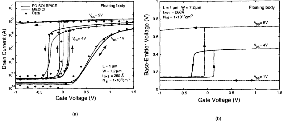
Fig. 7.7 (a) Subthreshold drain current ( I_D ) and (b) base-emitter voltage ( V_{BE} ) versus gate-source voltage ( V_{GS} ) of the parasitic bipolar device in the PD SOI NMOS device with a front gate oxide of 260 Å, a thin film doped with a p-type density of 10^{17} \text{ cm}^{-3} , a channel length of 1 \mu\text{m} , and a channel width of 7.2 \mu\text{m} , biased at V_{DS} = 1, 4, 5 \text{ V} , with its body node floating, based on the PD SOI-Technology SPICE model results, MEDICI [9] simulation results, and the experimental data [8]. (a) I_D vs V_{GS} .
