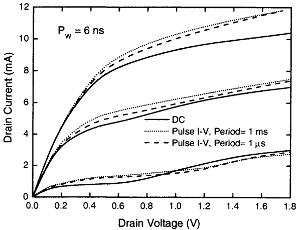
Fig. 2.113 Drain current versus drain voltage of an SOI NMOS device by pulse measurement with a 6 ns pulse width and periods of 1 ms and 1 μs. (Adapted from Shahidi et al. [12].)
