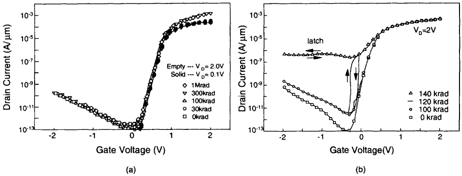
Fig. 3.95 Drain current versus gate voltage of the PD SOI NMOS device with a front gate oxide of 45 \text{ \AA} and a thin film of 1000 \text{ \AA} , under various irradiation doses. (a) with a channel length of 0.2 \text{ }\mu\text{m} and with both body and substrate grounded. (b) with a channel length of 0.1 \text{ }\mu\text{m} and with substrate grounded under various irradiation doses. (From Ferlet-Cavrois et al. [65]. ©1998 IEEE.)
