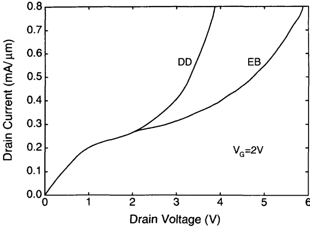
Fig. 2.78 Drain current versus drain voltage of the SOI NMOS device with a front gate oxide of 85 Å, a thin film of 420 Å doped with a density of 5 \times 10^{17} \text{ cm}^{-3} , and a buried oxide of 3000 Å, biased at a gate voltage of 2 V based on the conventional drift-diffusion (local) model and the energy balance (nonlocal) model. (Adapted from Apanovich [74].)
