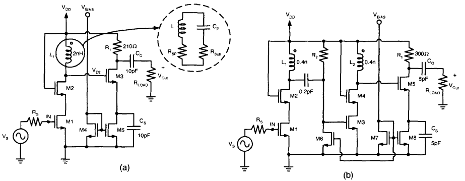
Fig. 6.34 (a) 4 GHz and (b) 13 GHz tuned amplifiers using SOI and SOS technologies. (Adapted from Ho et al. [28].)
