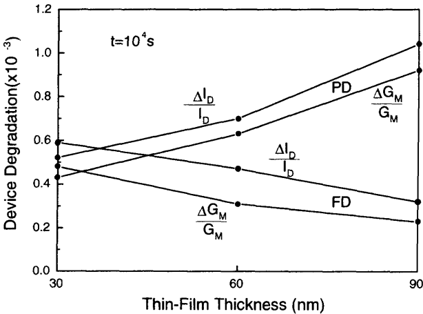
Fig. 3.8 Degradation of the drain current and transconductance versus the thin-film thickness of the SOI NMOS devices with a front gate oxide of 40 Å, a channel length of 0.1 μm, a buried oxide of 800 Å after a 10000-s stress at V_G = V_T + 0.35 V and V_D = 1.5 V, based on Monte Carlo simulation results. The PD device is with an N^+ polysilicon gate and a thin-film doping density of 10^{18} cm ^{-3} and the FD device is with a mid-gate workfunction gate and a thin-film doping density of 10^{16} cm ^{-3} . (Adapted from Hulfachor et al. [8]).
