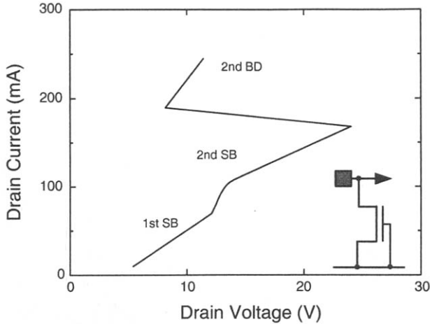
Fig. 3.67 The snapback characteristics of an SOI NMOS device with a front gate oxide of 190 Å, a thin film of 1800 Å doped with a p-type density of 10^{17} \text{cm}^{-3} , a channel length of 2 \mu\text{m} , and a channel width of 20 \mu\text{m} , measured by transmission-line pulsing techniques. (Adapted from Verhaege et al. [43].)
