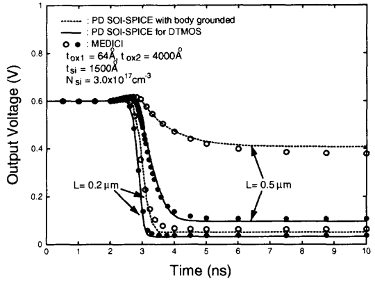
Fig. 7.15 Output transient waveforms of a body-grounded PD SOI NMOS device and an n-channel DTMOS device with a front gate oxide of 64 Å, a thin film of 1500 Å doped with a p-type density of 3 \times 10^{17} \text{ cm}^{-3} , a buried oxide of 4000 Å, and channel lengths of 0.2 and 0.5 μm, based on the PD SOI-Technology SPICE model results and the MEDICI simulation results.
