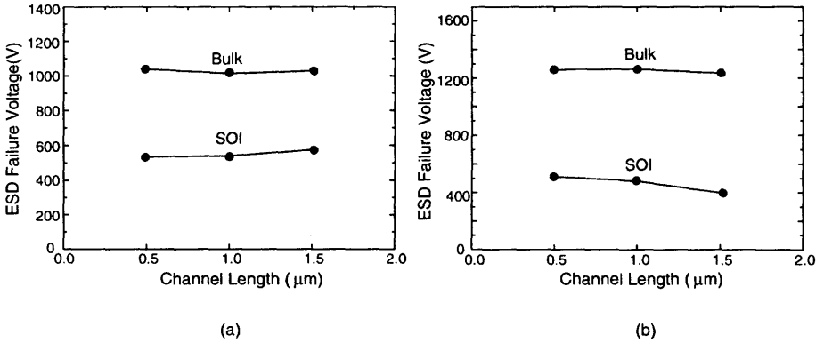
Fig. 3.69 HBM failure voltage versus channel length of the SOI and the bulk NMOS devices with their gates grounded (a) under a positive ESD HBM stress and (b) under a negative ESD HBM stress. (Adapted from Chan et al. [45].)
