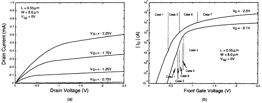
Fig. 3.22 (a) Drain current versus drain voltage and (b) drain current versus front gate voltage of the accumulation-mode SOI PMOS device with a front gate oxide of 125 \text{ \AA} , a 1000 \text{ \AA} thin film doped with a p-type density of 2 \times 10^{16} \text{ cm}^{-3} , a buried oxide of 3500 \text{ \AA} , with a channel length of 0.55 \mu\text{m} , and a channel width of 8 \mu\text{m} . (Adapted from Su & Kuo [17].)
