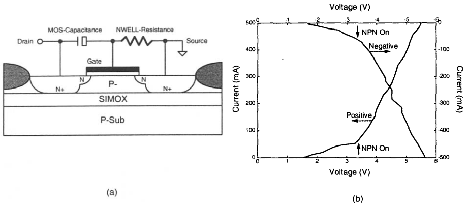
Fig. 3.72 (a) Gate-biased SOI NMOS ESD protection design. (b) Drain current versus drain voltage of the SOI NMOS device. (Adapted from Duvvury et al. [46].)
