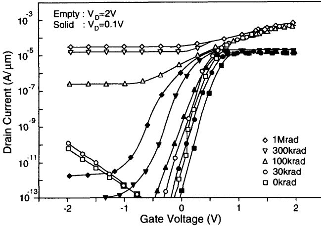
Fig. 3.94 Drain current versus gate voltage of the FD SOI NMOS device with a front gate oxide of 45 \text{ \AA} and a thin film of 400 \text{ \AA} , and a channel length of 0.2 \text{ }\mu\text{m} , biased with the substrate grounded and the drain voltages of 0.1 and 2 \text{ V} , for various irradiation doses. (Adapted from Ferlet-Cavrois et al. [65].)
