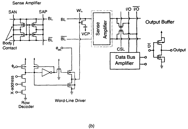
Fig. 5.25 (a) Cross-section of the 0.5 \mu\text{m} PD SOI NMOS device with a body contact via a polysilicon pad. (b) Critical path during the read operation of the DRAM. (From Suma et al. [26]. ©1994 IEEE.)
