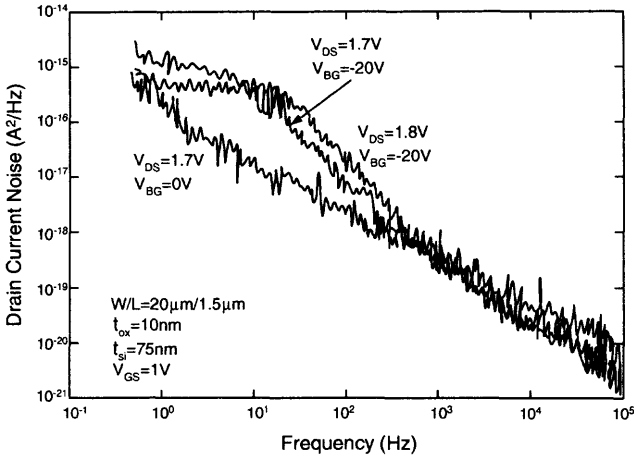
Fig. 4.38 Drain current noise spectral density versus frequency of the FD SOI NMOS device with a front gate oxide of 100 \text{ \AA} , a thin film of 750 \text{ \AA} , a channel width of 20 \mu\text{m} , and a channel length of 1.5 \mu\text{m} , biased at the gate-source voltage of 1 \text{ V} and (1) the drain-source voltage of V_{DS} = 1.7 \text{ V} and the back gate voltage of V_{BG} = -20 \text{ V} , (2) the drain-source of voltage V_{DS} = 1.8 \text{ V} and the back gate voltage of V_{BG} = -20 \text{ V} , and (3) the drain-source voltage of V_{DS} = 1.7 \text{ V} and the back gate voltage of V_{BG} = 0 \text{ V} . (Adapted from Jin et al. [26].)
