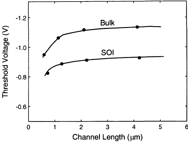
Fig. 2.12 Threshold voltage versus channel length of SOI and bulk PMOS devices. The SOI device has a front gate oxide of 150 Å, a thin film of 2200 Å, and a buried oxide of 4000 Å. The doping density of the n-type silicon is 8 \times 10^{15} \text{ cm}^{-3} . (Adapted from Hashimoto et al. [19].)
