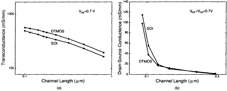
Fig. 3.43 (a) Transconductance and (b) output conductance versus channel length of the SOI NMOS device with a nitride front gate oxide of 27 Å and a thin film of 1200 Å, in DTMOS and conventional configurations, biased at the drain voltage of 0.7 V. (Adapted from Tanaka et al. [29].)
