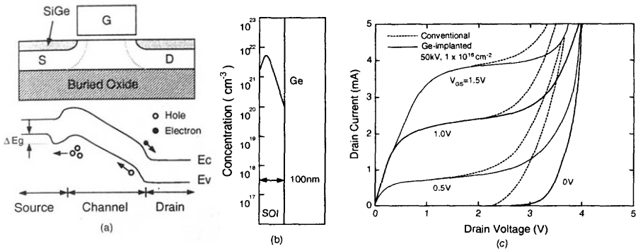
Fig. 2.59 (a) Structure and bandgap diagram of a PD SOI NMOS device with Ge-implanted source/drain. (b) Ge profile in the source/drain region. (c) Drain current characteristics of the Ge-implanted PD SOI NMOS device with a channel length of 0.15\ \mu\text{m} and a channel width of 10\ \mu\text{m} , a front gate oxide of 50\ \text{\AA} , and a thin film of 1000\ \text{\AA} . (Adapted from Yoshimi et al. [59].)
