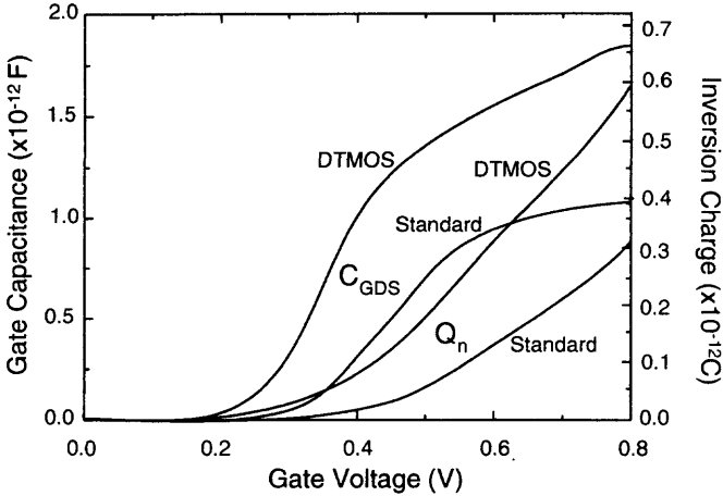
Fig. 3.39 Gate capacitance and inversion charge versus gate voltage of SOI NMOS device with a front gate oxide of 64 Å, a thin film of \sim 1500 Å doped with a p-type density of 3 \times 10^{17} \text{ cm}^{-3} , channel width and length of 20 \mu\text{m} , in standard MOS configuration with body grounded and in the DTMOS configuration. (Adapted from Assaderaghi et al. [27].)
