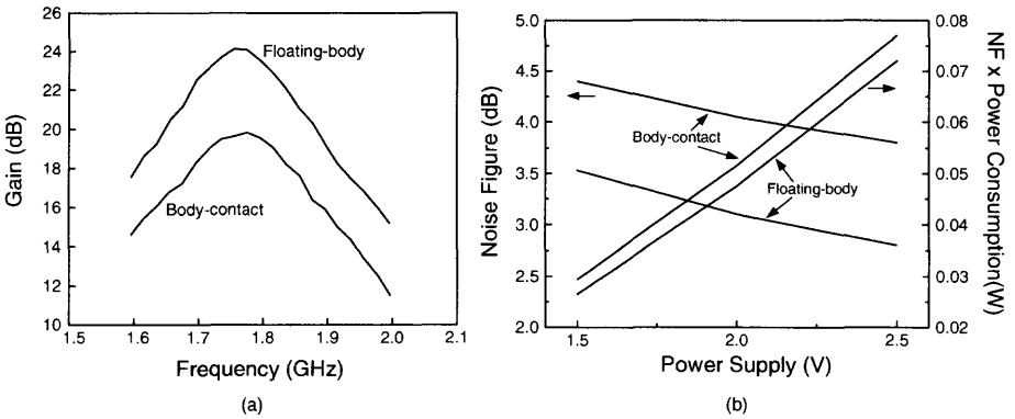
Fig. 6.32 (a) Gain versus frequency and (b) noise figure versus power supply voltage of this cascoded SOI LNA circuit. (Adapted from Jin et al. [26].)
