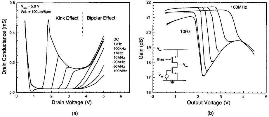
Fig. 4.16 (a) Drain conductance versus drain voltage of an SOI NMOS device at various operating frequencies. (b) Gain versus output voltage of an amplifier stage using an SOI NMOS device as the input device for various operating frequencies. (Adapted from Assaderaghi et al. [11].)
