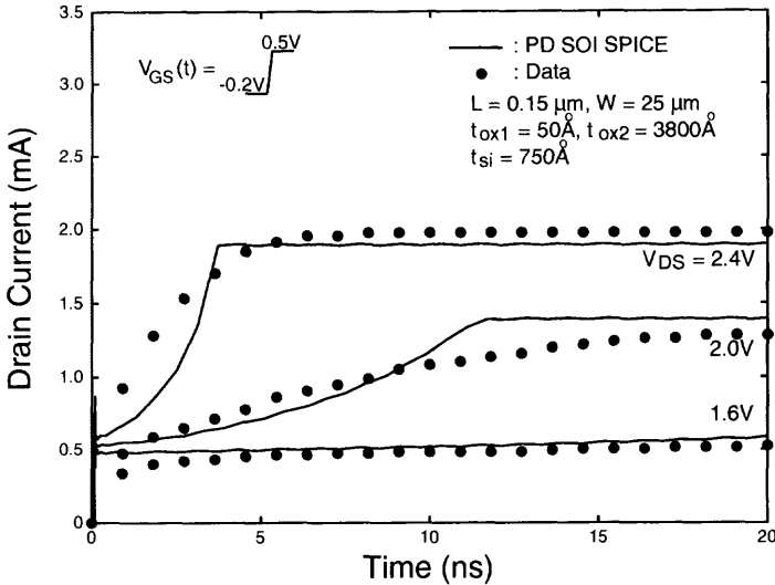
Fig. 7.11 Drain current characteristics during the turn-on transient of the PD SOI NMOS device with a front gate oxide of 50 \text{ \AA} , a thin film of 750 \text{ \AA} , a buried oxide of 3800 \text{ \AA} , a channel length of 0.15 \text{ }\mu\text{m} , and a channel width of 25 \text{ }\mu\text{m} , with its body node floating for various drain voltages, by imposing an input step from -0.2 to 0.5 \text{ V} at its gate, based on SOI-technology SPICE model results and the experimental data [10].
