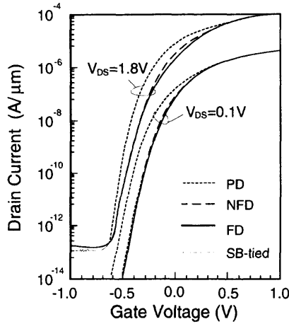
Fig. 2.63 Subthreshold drain current characteristics of PD and FD SOI NMOS devices biased at V_D = 0.1 V and 1.8 V. (Adapted from Tseng et al. [63].)
