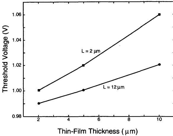
Fig. 2.24 Threshold voltage versus thin-film thickness of an SOI NMOS device with a front gate oxide of 190 Å and a channel length of 12 and 2 μm showing the reduced reverse SCE after anneal. (Adapted from Tsoukalas [30].)
