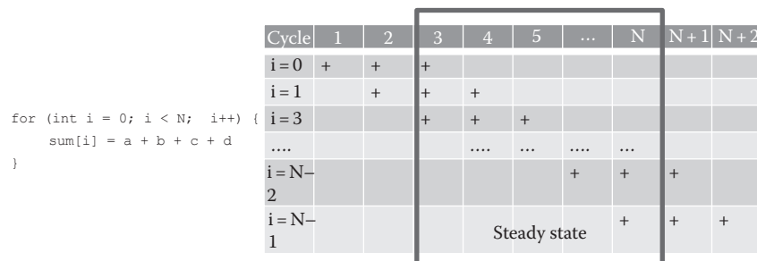
FIGURE 16.7 Polyhedral loop model.
