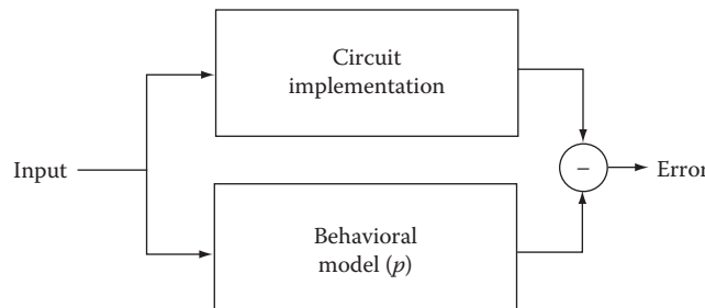
FIGURE 18.14 Basic flow of fitting or regression approach for analog behavioral model generation.
