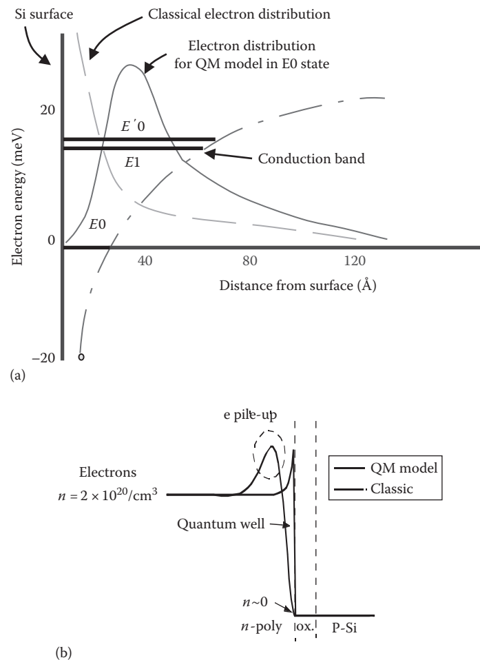
FIGURE 28.11 (a) Surface region of bulk MOS device that shows well potential created by the conduction band energy (-); discrete energy levels imposed by QM ( E_0, E_1 ); electron distribution based on classical theory (- - -). (b) Electron distribution in the n-type poly-silicon gate of an NMOS transistor, comparing charge buildup based on classical theory vs. that for a quantum-based (QM) solution for charge. The peak region shows a “QM depletion” resulting in V_{th} and C-V shifts.
