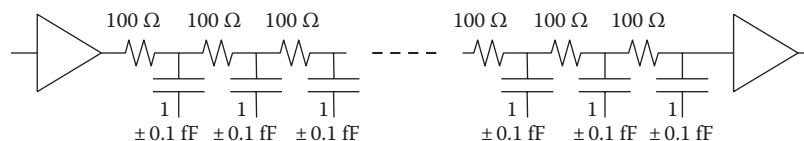
FIGURE 29.12 Statistical error cancellation occurs in resistance and capacitance (RC) networks. The total Elmore delay time due to 25 RC stages here is 32.5 \pm 7.4 ps ( \pm 2.3\% ).
