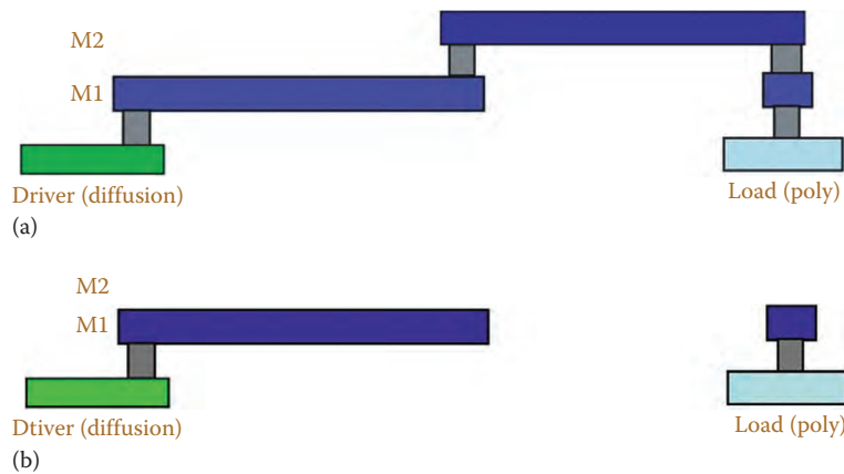
FIGURE 8.22 (a) The routing solution avoids connecting the long Metal1 wire to the gate of the load during fabrication. (b) The routing solution in (a) prevents the antenna effect.
