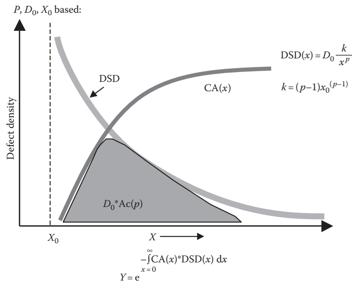
FIGURE 22.5 Random defect limited yield model.
