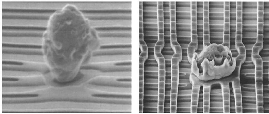
FIGURE 22.2 Random defects causing metal opens and shorts.
