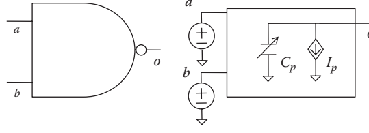
FIGURE 6.2 Example of a current source model: the output port is modeled as a nonlinear voltage-controlled current source dependent on all input port voltages, in parallel with a nonlinear capacitance.
