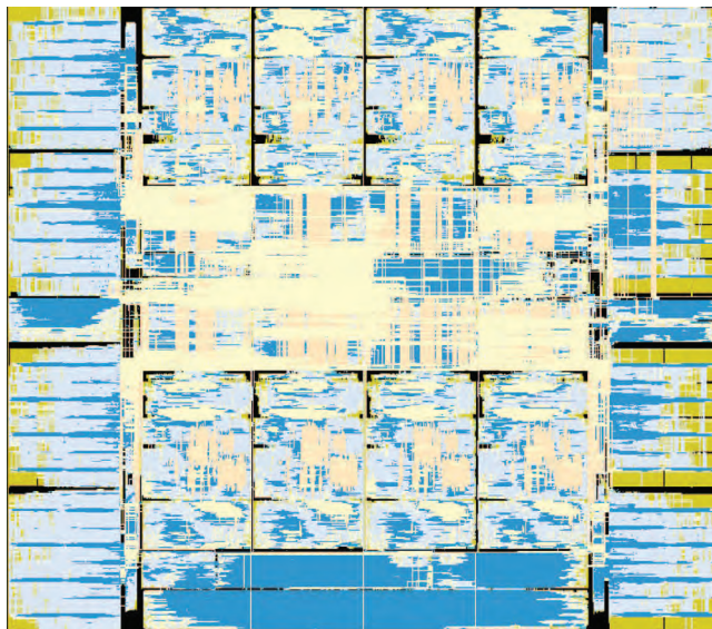
FIGURE 9.10 GDSII layouts of OpenSPARC T2 (full chip): 2D IC design ( 9 \times 7.9 \text{ mm}^2 ). (Image from Jung, M. et al., On enhancing power benefits in 3D ICs: Block folding and bonding styles perspective, in Proceedings of ACM Design Automation Conference , 2014.)
