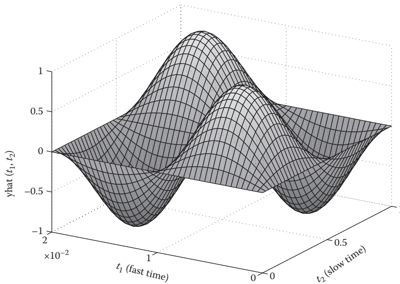
FIGURE 17.10 Corresponding two-periodic bivariate form \hat{y}(t_1, t_2) .
