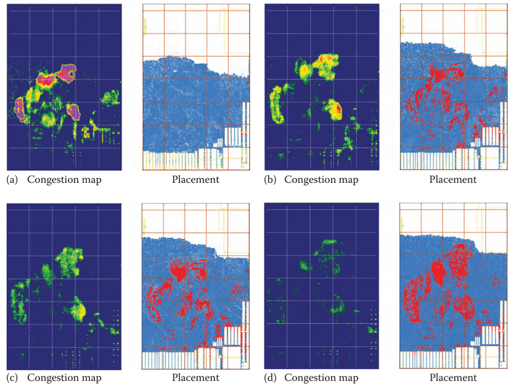
FIGURE 8.11 Progression of routability-driven placement. Red color indicates locations where cell utilization was temporarily decreased. (a) Initial placement (right) with areas of high congestion. (b) Intermediate placement where congestion is reduced. (c) Intermediate placement where congestion is further reduced. (d) Near-final placement where congestion is largely removed.
