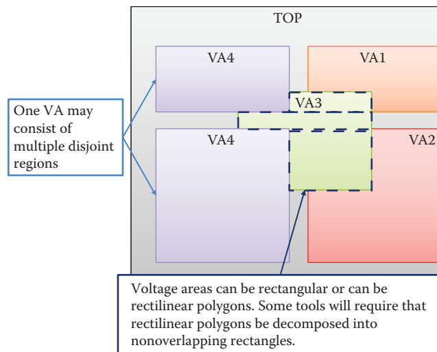
FIGURE 15.5 Voltage areas.
