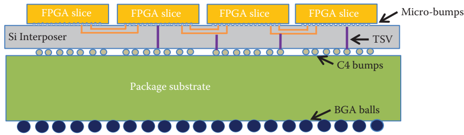
FIGURE 16.26 2.5D Virtex-7 FPGA built with silicon interposer technology.
