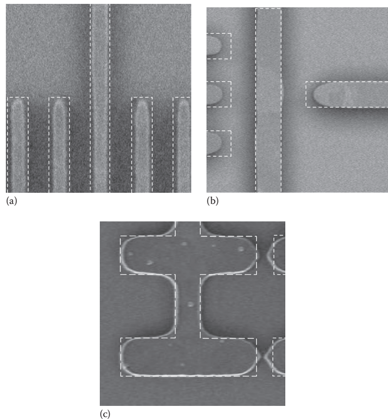
FIGURE 21.4 Typical image fidelity problems that can be corrected through OPC: (a) Iso-dense bias; (b) line-end pullback; and (c) corner rounding. (From Schellenberg, F.M. et al., SEMATECH J111 Project: OPC validation, Optical Microlithography XI, Proceedings of SPIE , Vol. 3334, 1998, pp. 892–911. With permission.)
