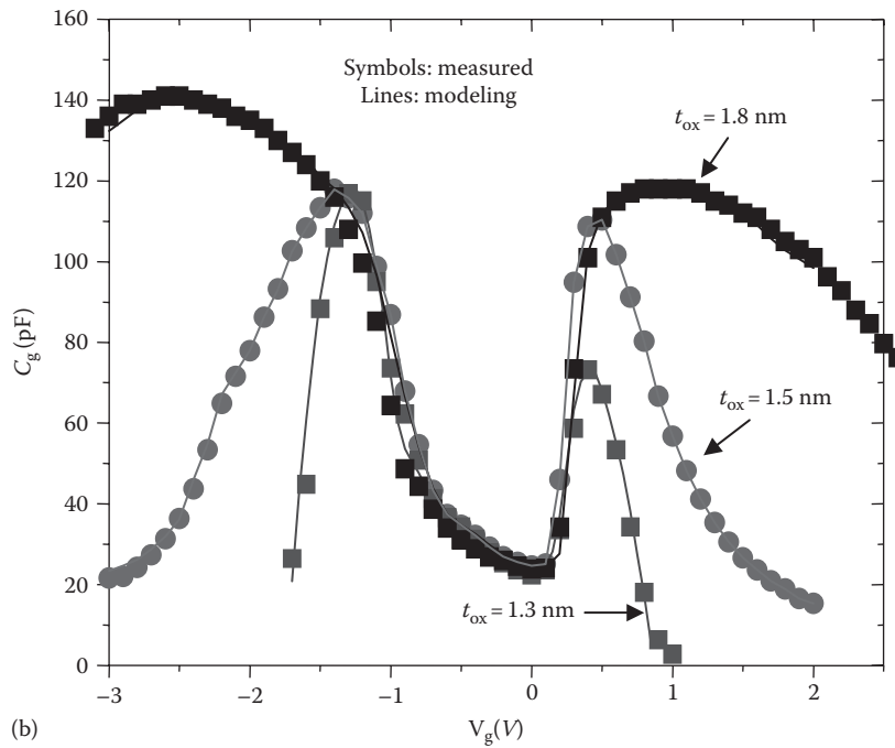
FIGURE 28.10 (a) Equivalent circuit (lumped) model for large area ( 100\ \mu\text{m} \times 100\ \mu\text{m} ) MOS capacitor, S/D grounded showing distributed R - C effects well as dependent generators representing tunneling current. (b) Results comparing measure and equivalent circuit simulations of imaginary component of input admittance for large area MOS capacitors structure with oxide thickness as a parameter.
