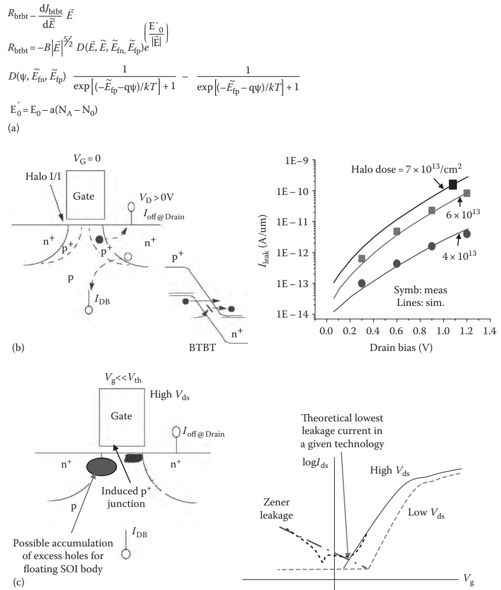
FIGURE 28.15 (a) Rate equation for band-to-band tunneling ( R_{\text{btbt}} ) expressed in terms of the tunneling current density per unit of energy ( dJ/dE ) with supporting equations for the rate equation for the rate equation [32], including a modified term for the doping dependence [33]. (b) Schematic view of the band-to-band tunneling, including trap-assisted tunneling, and plots of the modeling results (Figure 28.15a) along with experimental data for different HALO implant doses [33]. (c) Schematic view of the band-to-band tunneling in the gate-induced drain leakage (GIDL) region. The leakage current has a negative transconductance and determines the lowest possible leakage current in high V_{\text{ds}} .
