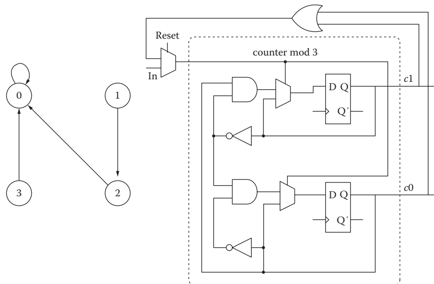
FIGURE 4.19 Extending the counter with reset.
