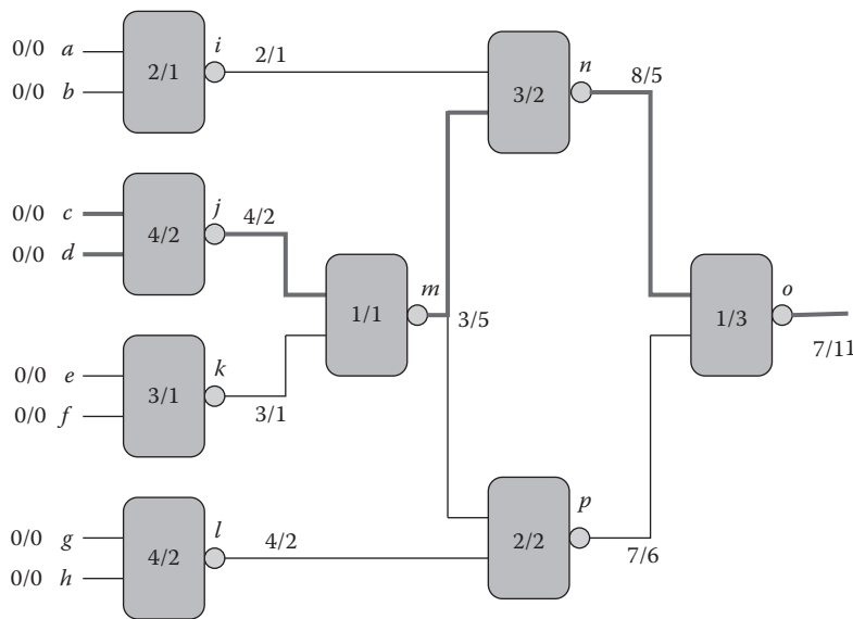
FIGURE 6.5 An example illustrating the application of the critical path method on a circuit with inverting gates. The numbers within the gates correspond to the rise/fall delay of the block, and the italicized bold numbers at each block output represent the rise/fall arrival times at that point. The primary inputs are assumed to have arrival times of zero, as shown. (From Sapatnekar, S.S., Timing , Kluwer Academic Publishers, Boston, MA, 2004.)
