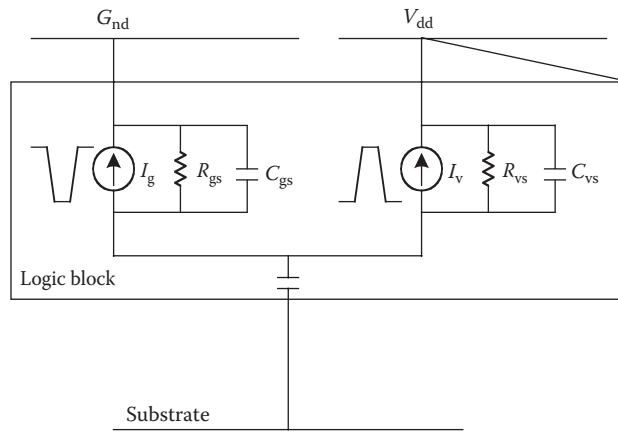
FIGURE 26.18 Simple linear macromodel of logic block for switching noise in power distribution synthesis. (From Stanisic, B.R. et al., Proc. IEEE J. Solid-State Circ. , 321, 1995. With permission.)
