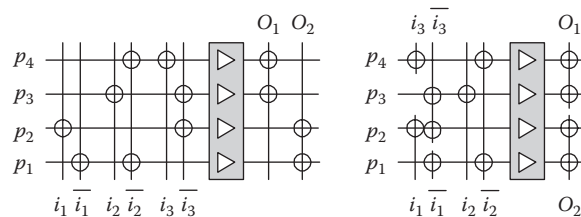
FIGURE 7.16 Programmable logic array folding.
