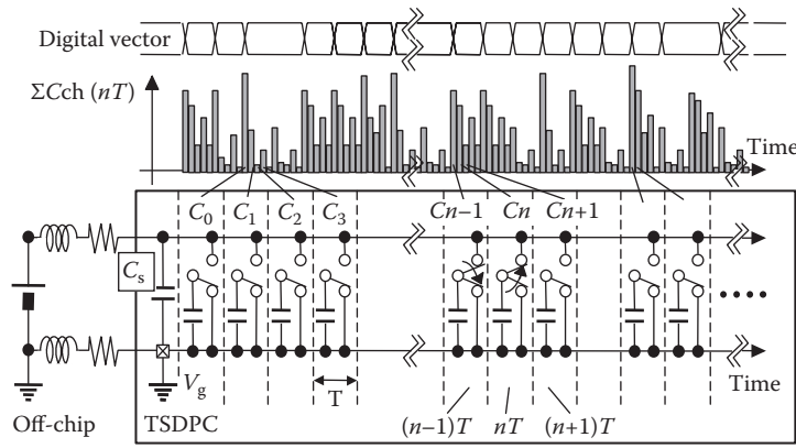
FIGURE 26.5 Time series divided parasitic capacitance (TSDPC) model. (From Nagata, M. et al., Modeling substrate noise generation in CMOS digital integrated circuits, Proceedings of IEEE Custom Integrated Circuits Conference , Orlando, FL, May 12–15, 2002, pp. 501–504.)
