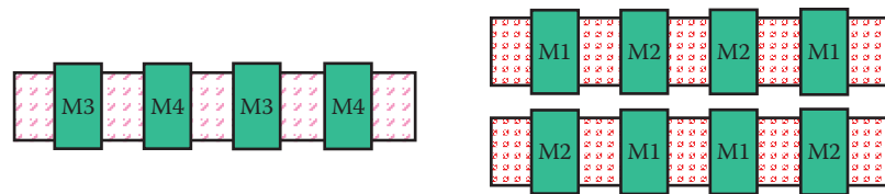
FIGURE 19.1 Device stacking with single-row inter-digitized or multi-row common-centroid placement.
