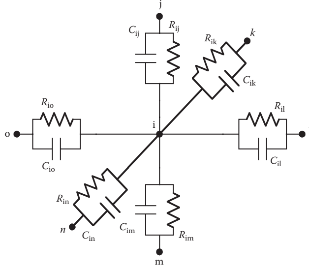
FIGURE 26.7 Resistances and capacitances around a mesh node in the electrical substrate mesh. (From Stanisic, B.R. et al., IEEE J. Solid-State Circ. , 29, 226, 1994. With permission.)
