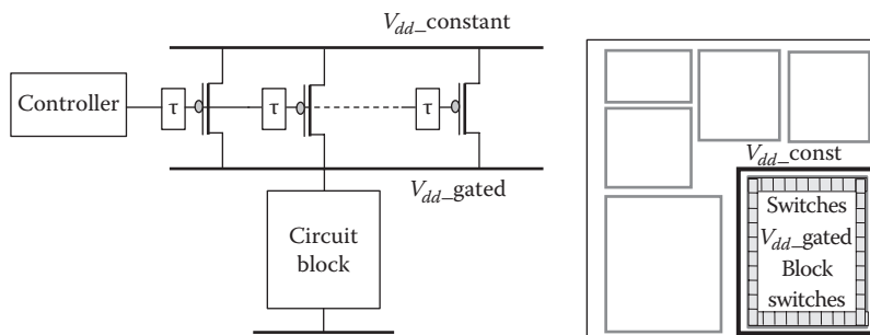
FIGURE 23.11 Coarse-grained power gating.
