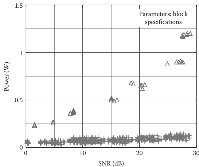
FIGURE 18.7 Power consumption comparison between the all-digital CATV architecture (triangles) and the classical architecture (crosses), as a function of the required SNR. (From Wambacq, P. et al., High-level simulation and power modeling of mixed-signal front-ends for digital telecommunications, Proceedings of the International Conference on Electronics, Circuits and Systems (ICECS) , September 1999, pp. 525–528. With permission.)
