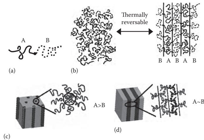
FIGURE 21.13 (a) A single PS- b -PMMA co-polymer strand; (b) polymer phase separation for PS- b -PMMA. When the molecular weights of the two components are (c) unequal, cylinders form; and (d) approximately equal, lamella form. (Adapted from Schellenberg, F.M. and Torres, J.A.R., Contemporary design paradigms applied to novel lithography, SEMATECH 2006 Litho Forum Poster IM06, Slides 3 & 4.)
