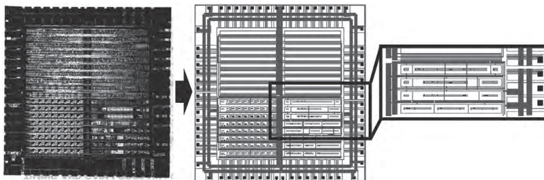
FIGURE 19.6 Example of a mixed-signal power grid from a commercial IBM ASIC, redesigned automatically by the RAIL tool [134,138] to meet strict AC, DC, and transient specifications. (From Stanisic, B.R. et al., Power distribution synthesis for analog and mixed signal ASICs in RAIL, Proceedings of IEEE Custom IC Conference , San Diego, CA, 1993, pp. 174.1–174.5; Stanisic, B.R. et al., Synthesis of Power Distribution to Manage Signal Integrity in Mixed-Signal ICs , Kluwer Academic Publishers, Norwell, MA, 1996.)
