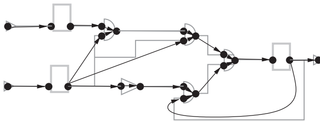
FIGURE 10.1 Example of a timing graph and its underlying netlist.
