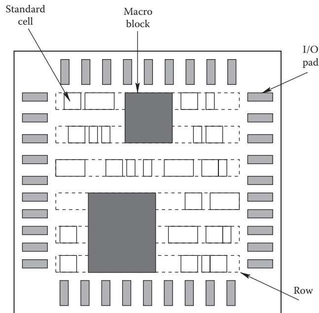
FIGURE 5.2 Placement layout area.
