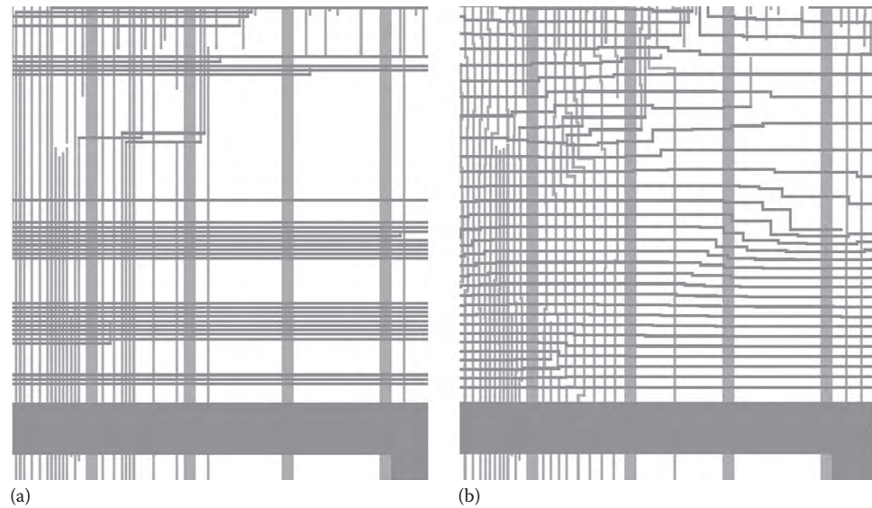
FIGURE 13.21 Before (a) and after (b) wire spreading.
