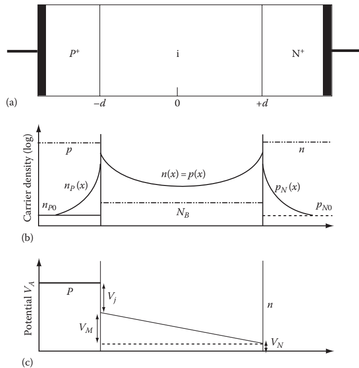
FIGURE 17.4 (a) Cross-sectional diagram of a p- i -n power diode; (b) corresponding carrier distribution profile; and (c) potential distribution for high-level injection conditions.
