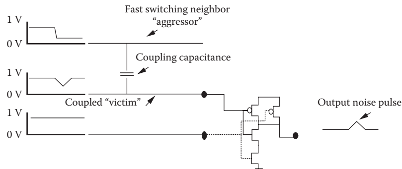
FIGURE 13.5 Coupling-induced logic glitch.
