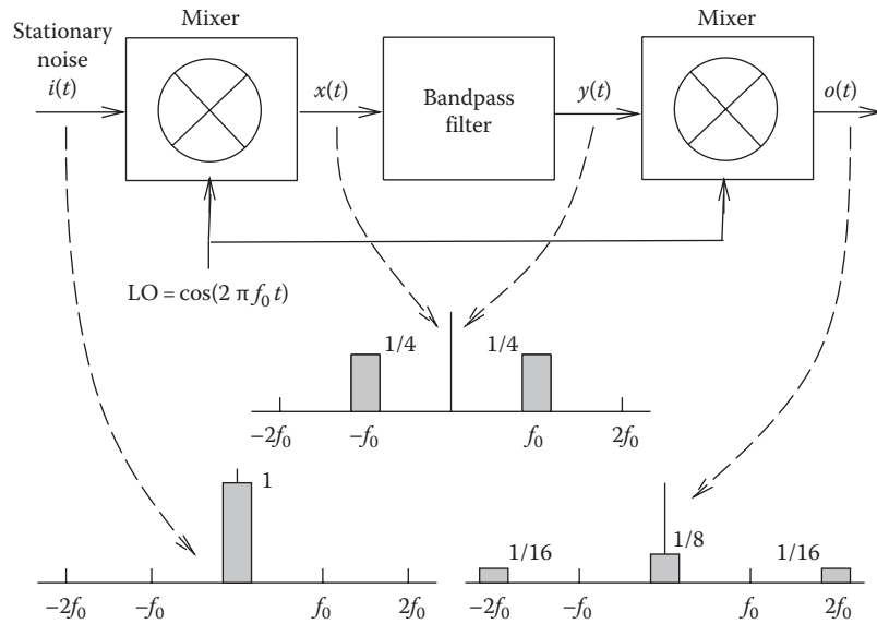
FIGURE 17.22 Mixer–filter–mixer circuit: naïve analysis.
