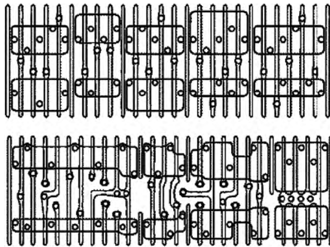
FIGURE 21.36 Diffusion, poly, and contact lithography variability-bands for pdBrix layout (top) and conventional layout (bottom). (From Liebmman, L. et al., Simplify to survive: Prescriptive layouts ensure profitable scaling to 32nm and beyond , Design for Manufacturability through Design-Process Integration III , Proceedings of SPIE , Vol. 7275, 2009. With permission.)
