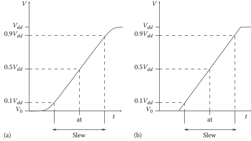
FIGURE 10.2 A (rising) signal transition (a) and its approximation (b).
