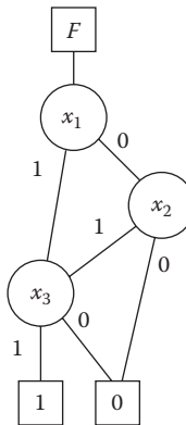
FIGURE 4.3 Binary decision diagram for F = (x_1 \wedge x_3) \vee (x_2 \wedge x_3) .
