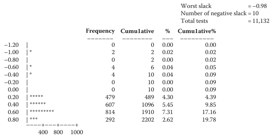
FIGURE 13.14 Timing-slack histogram.
