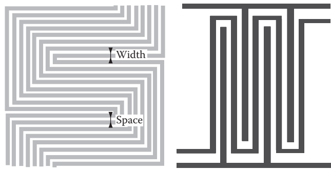
FIGURE 22.9 Nest and snake/comb structures for random defectivity characterization.
