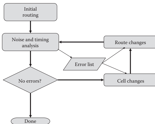
FIGURE 24.22 Noise correction flow.
