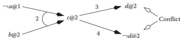
FIGURE 4.5 Implication graph. Each implication is annotated with the ordinal of the clause in Equation 4.5 that caused it.
