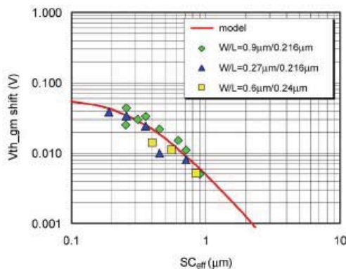
Fig. 2. Change in threshold voltage as a function of MOS channel-to-well distance, SC_{\text{eff}} [2].
