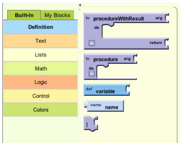
Figure 11-7. Definition blocks
