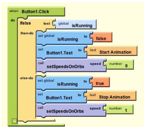
Figure 11–20. Button1.Click procedure
