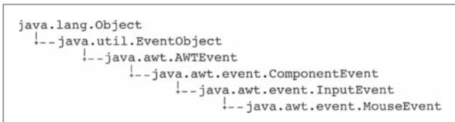
Figure 15-28 The inheritance hierarchy of the MouseEvent class
