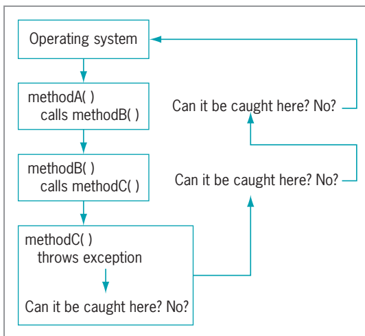
Figure 12-24 Cycling through the call stack
