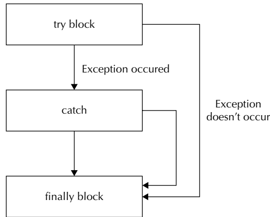
FIGURE 8-2. The try/catch/finally program flow
