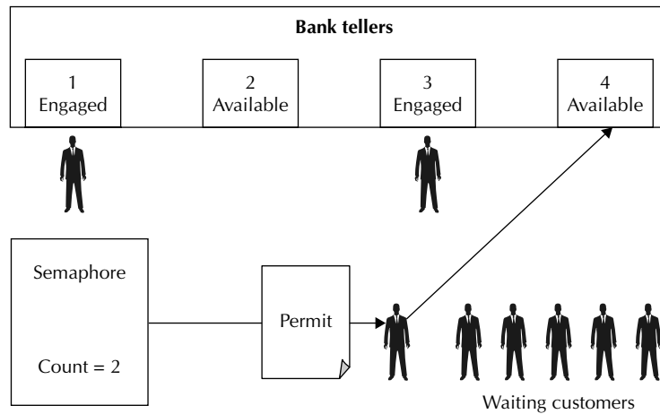
FIGURE 18-3. A banking scenario that implements semaphores
