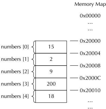
FIGURE 2-4. Displaying the memory map of an integer array
