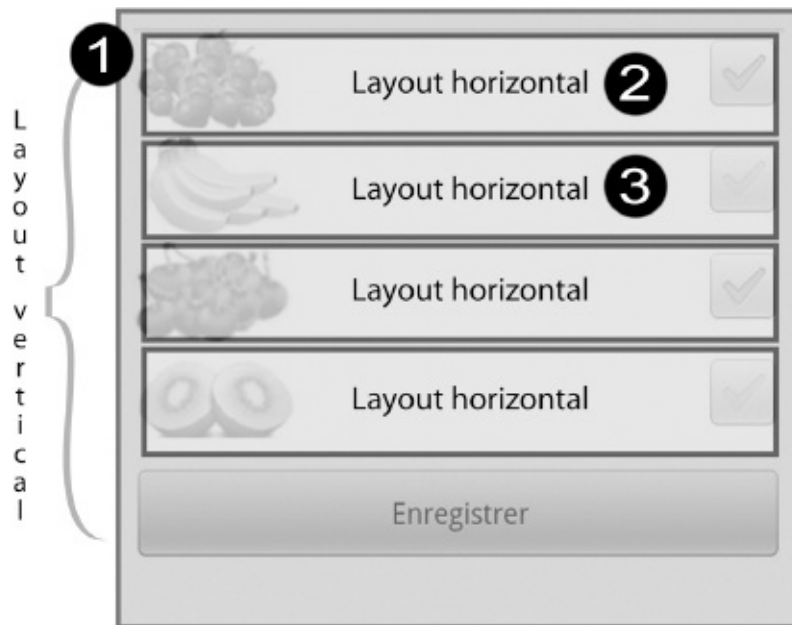
Figure 13-14 Imbrication de layouts
