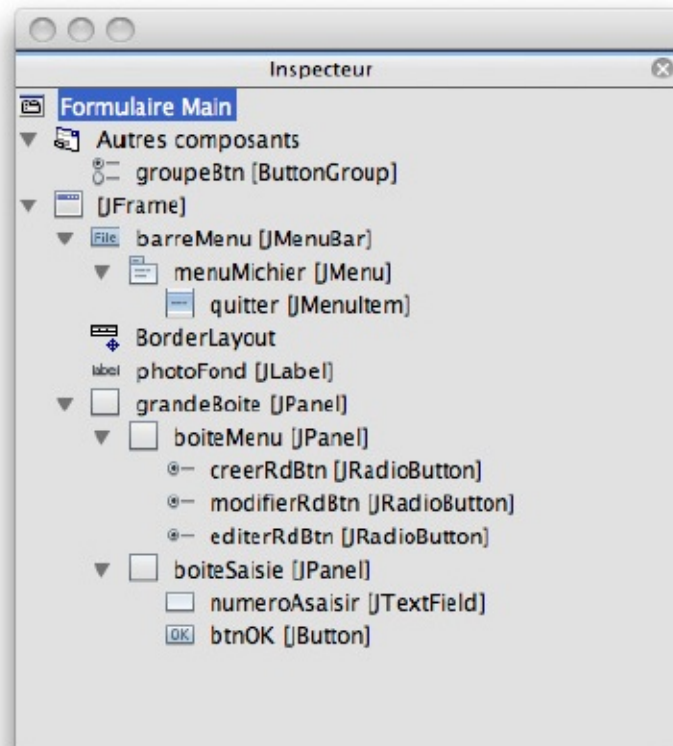
Figure 12-51 Structure de la classe Main
