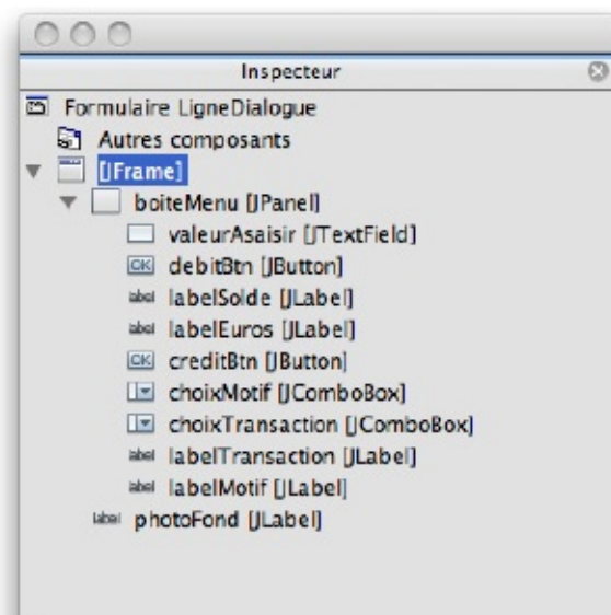
Figure 12-53 Structure de la classe LigneDialogue
