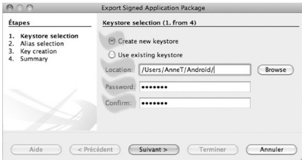
Figure 13-26 Le panneau Export Signed Application Package
