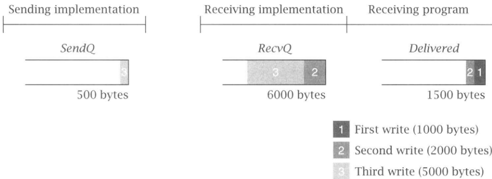
Figure 5.3: After first read().
