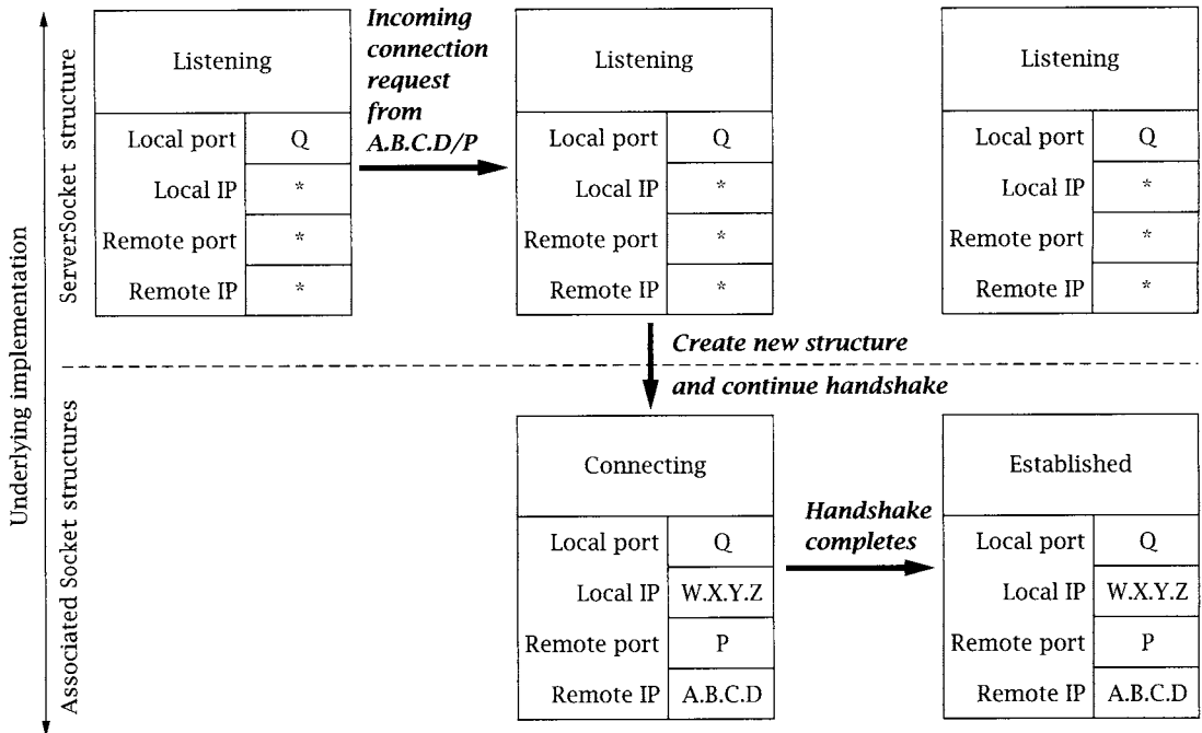
Figure 5.8: Incoming connection request processing.
