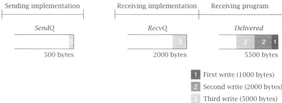
Figure 5.4: After another read().
