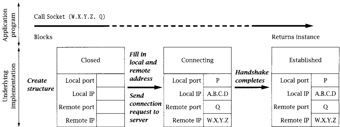
Figure 5.6: Client-side connection establishment.
