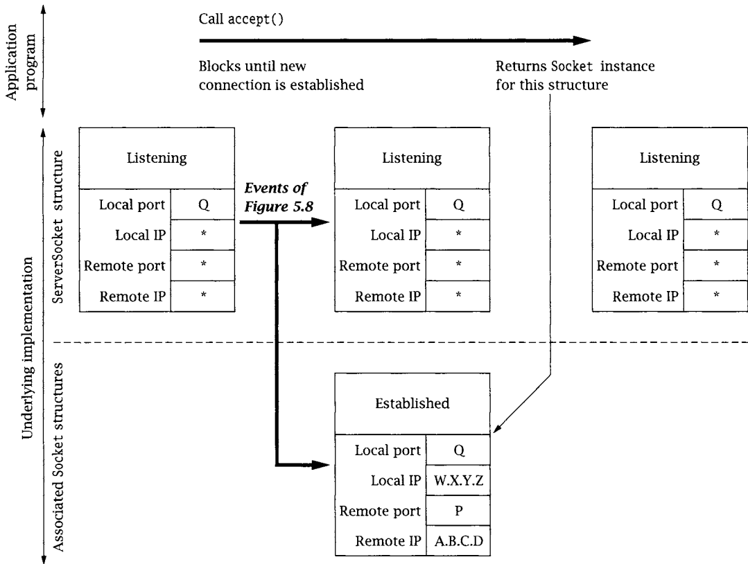
Figure 5.9: accept() processing.
