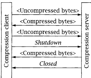
Figure 4.2: Compression protocol termination.
