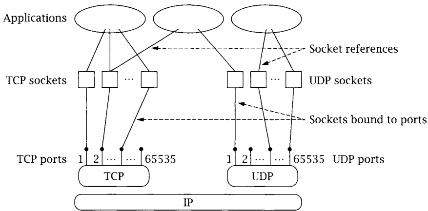
Figure 1.2: Sockets, protocols, and ports.
