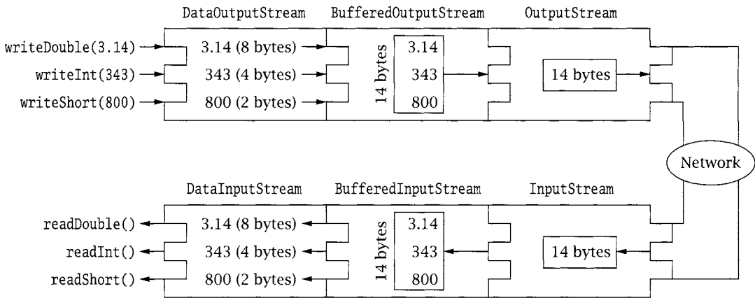
Figure 3.1: Stream composition.
