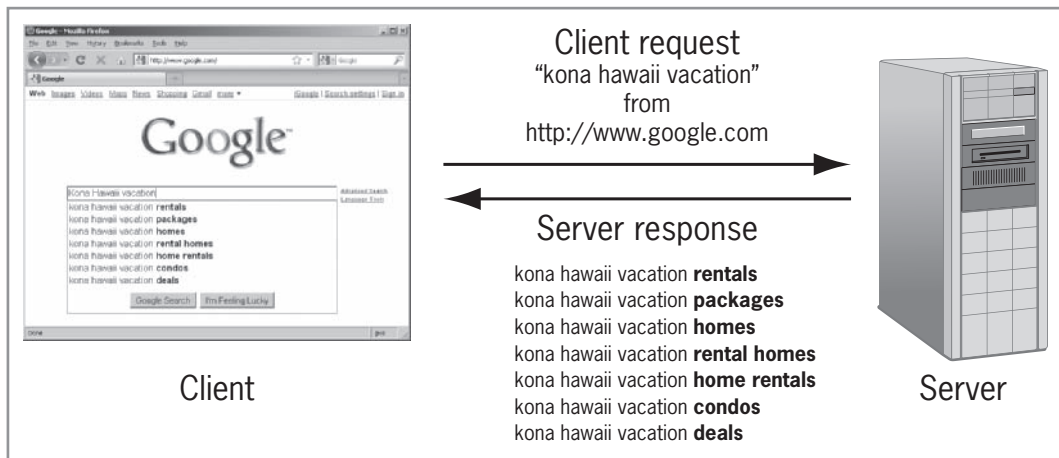
Figure 12-3 HTTP request with the XMLHttpRequest object
