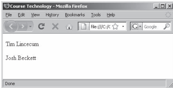
Figure 2-2 Output of a program that contains a global variable and a local variable with the same name
