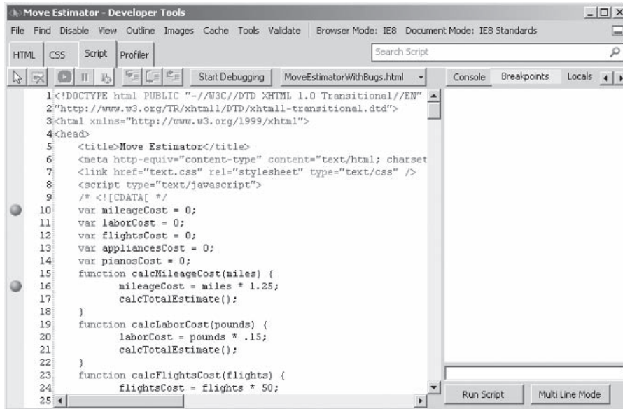
Figure 8-15 Breakpoint in JScript debugger
