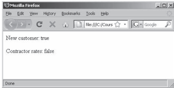
Figure 2-5 Boolean values
