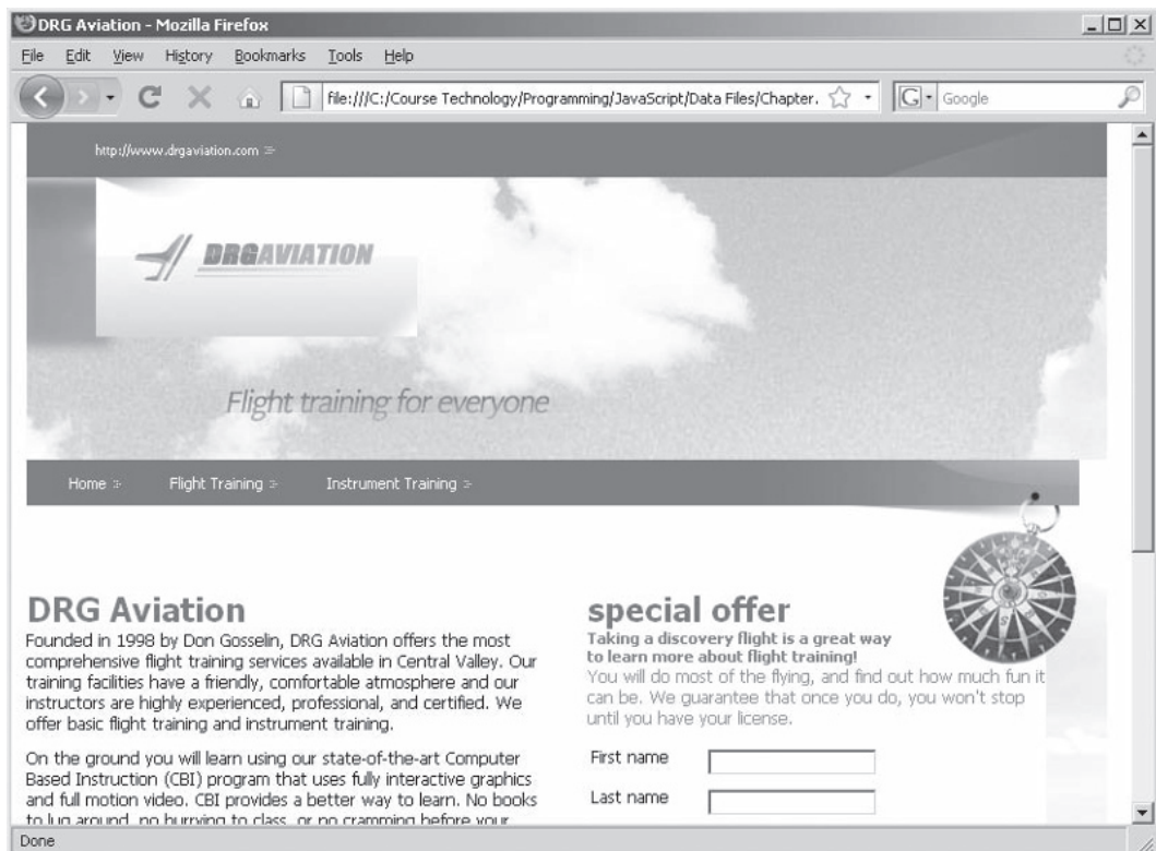
Figure 10-2 index.html
