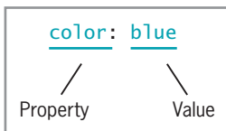
Figure C-2 Style declaration
