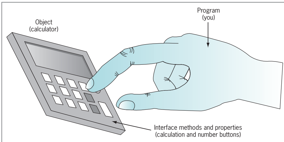
Figure 6-2 Calculator interface
