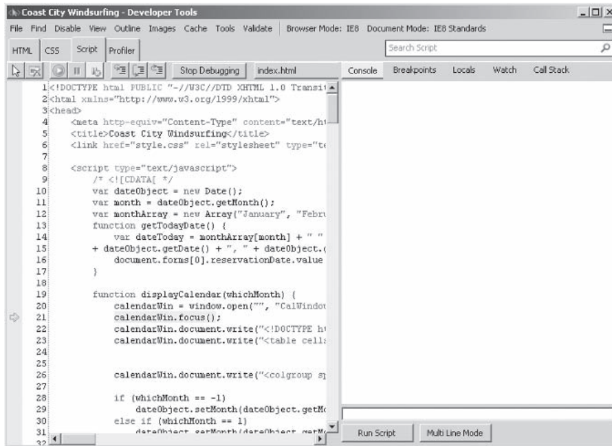
Figure 8-11 Document opened in JScript debugger
