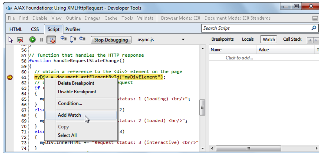
Figure 6-9: Watching variables
