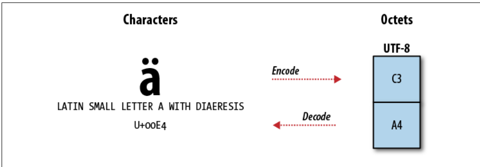
Figure C-1. The code point of a character is not its storage. The encoding transforms characters into storage.
