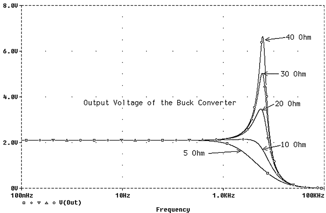
FIGURE 23.12 Simulation results for AC analysis of the buck converter from Fig. 23.11.
