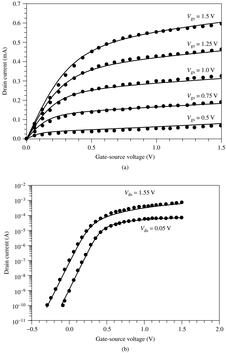
Figure 8.3 Experimental (symbols) and modeled (a) above-threshold and (b) subthreshold characteristics for a deep submicrometer nMOS with effective gate length L = 0.09 \mu\text{m} . Device parameters: W = 1 \mu\text{m} , d_i = 3.5 \text{ nm} , \mu_n = 0.026 \text{ m}^2/\text{Vs} , v_s = 6 \times 10^4 \text{ m/s} , m = 2.2 , R_s = R_d = 200 \Omega , \lambda = 0.142/\text{V} , \eta = 1.7 , V_{T0} = 0.335 \text{ V} , \sigma_0 = 0.11 , V_\sigma = 0.2 \text{ V} , V_{\sigma t} = 0.18 \text{ V} . Substrate-source bias V_{bs} = 0 \text{ V} . Reproduced from Ytterdal T., Shur M., and Fjeldly T. A. (1994) Sub-0.1 \mu\text{m} MOSFET modeling and circuit simulation, Electron. Lett. , 30 , 1545, 1546 and Mii Y. et al. (1994) Experimental high performance sub-0.1 \mu\text{m} channel nMOSFET's, IEEE Electron Devices Lett. , EDL-15 , 28–30
