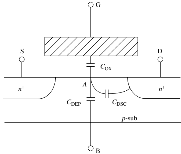
Figure 6.15 Illustration of the gate oxide capacitance, channel depletion capacitance, and C_{\text{dsc}} coupling capacitances
