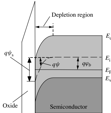
Figure 1.4 Band diagram for MOS capacitor in weak inversion ( \phi_b < \psi_s < 2\phi_b )
