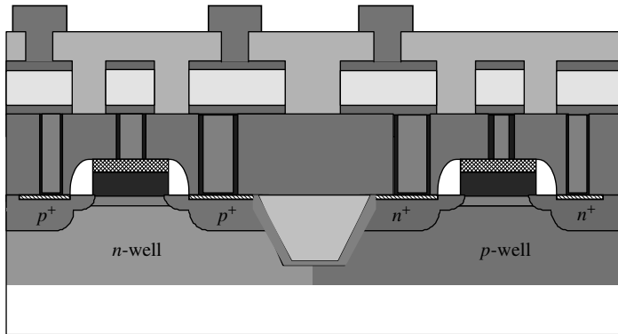
(22) Metal 2 etch
