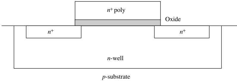
Figure 2.4 Cross section of a MOS varactor
