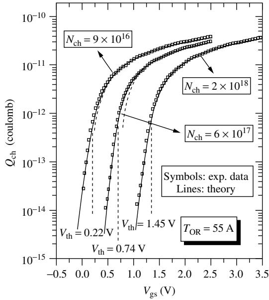
Figure 6.14 Channel charge model fits the measurement data taken from devices with different N_{\text{ch}} well. The model covers weak, moderate, and strong inversion regions of n MOSFETs. Reproduced from Cheng Y. et al. (1998) A unified MOSFET channel charge model for device modeling in circuit simulation, IEEE Trans. Computer-Aided Design Integrated Circuits Syst. , 17 , 641–644
